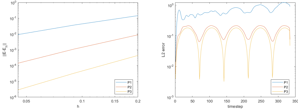
Figure 3: h -Convergence results for the PEC cavity problem with a centered fluxes DG discretization in the time interval [0, 1] (left) and evolution of the L_2 error in time (right).
