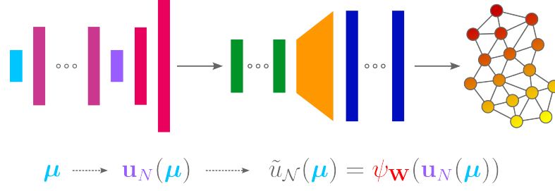
Figure 5: Online phase for the GCA-ROM architecture [6].
