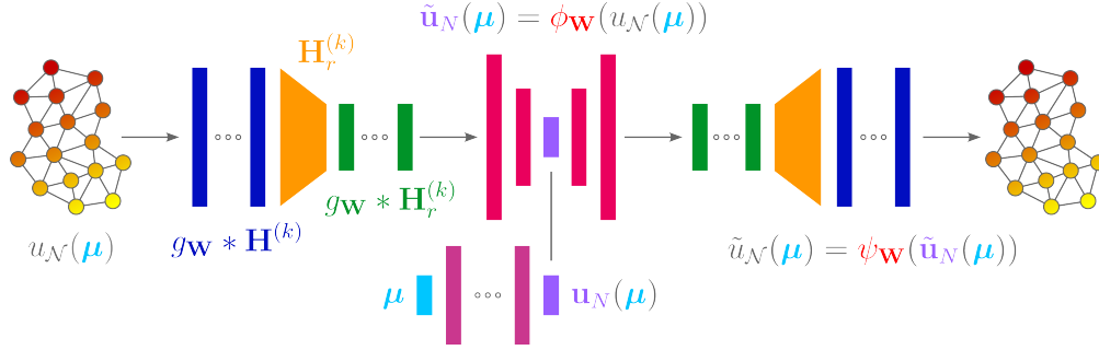
Figure 4: Offline phase for the GCA-ROM architecture [6].
