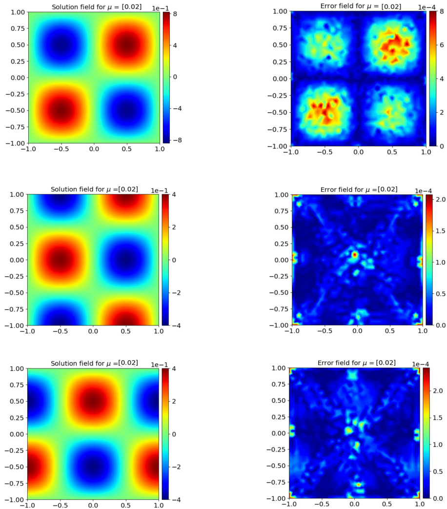
Figure 7: AVG-DG-GCA solution and error fields for the electric field (top) and x and y components of the magnetic field, at the instant of time t = 0.02 , on a mesh with 1220 nodes.
