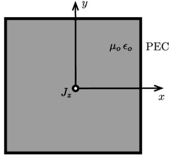
Figure 1: Metallic air-filled cavity \Omega = [-1, 1]^2 .
