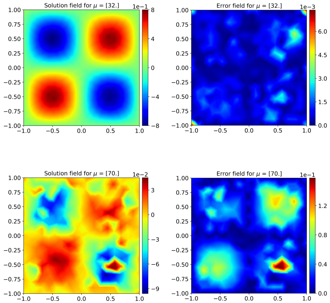
Figure 8: AVG-DG-GCA solution fields and error field for the electric field obtained training over a time of three periods.
