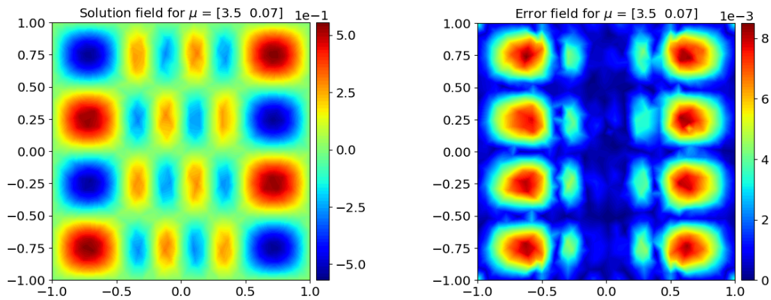
Figure 19: AVG-DG-GCA solution and error fields for the E^z component of the perfect electric conductor cavity with two material interfaces with \varepsilon_1 = 3.5 (training over half a period).
