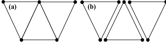
Figure 6: Representation of a classical Galerkin method (a), and representation of the DG method (b), for P_1 elements.
