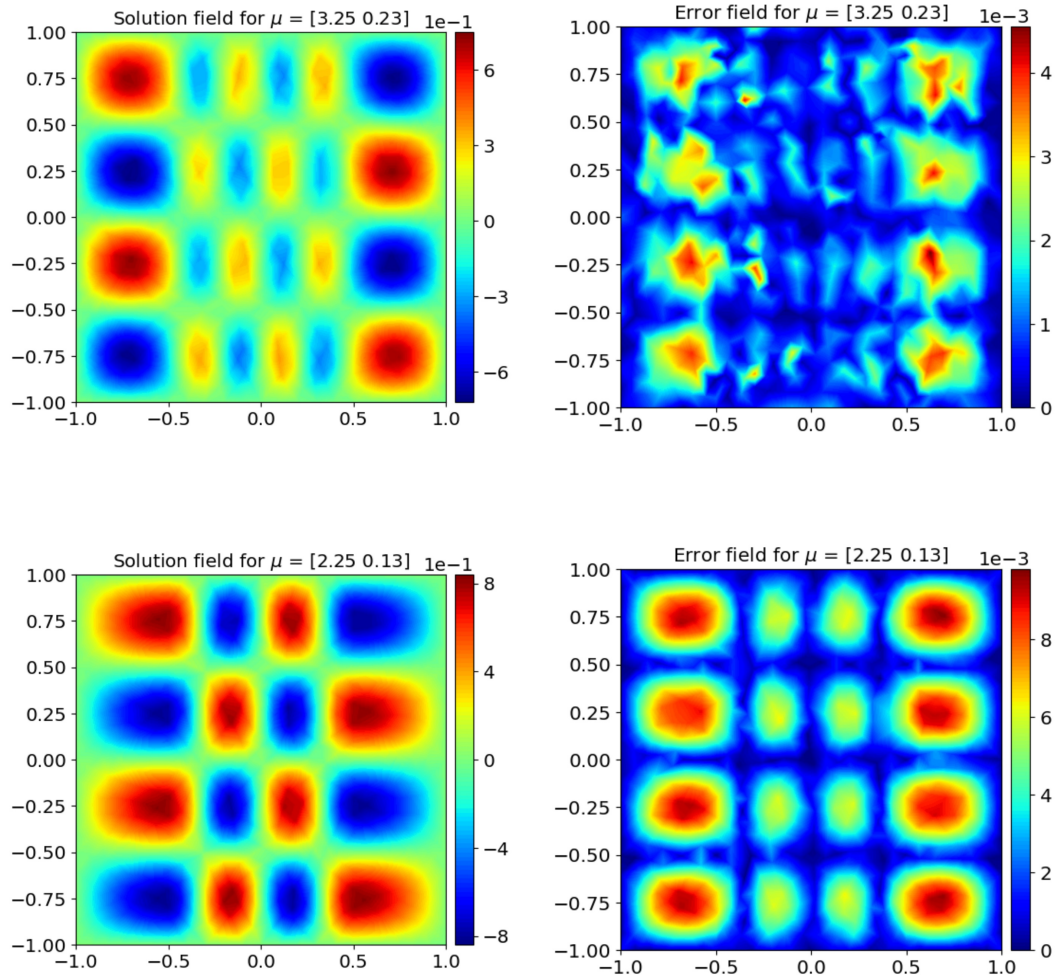
Figure 16: AVG-DG-GCA solution and error fields for the E_z component of the perfect electric conductor cavity with two material interfaces with \varepsilon_1 = \{3.25, 2.25\} .
