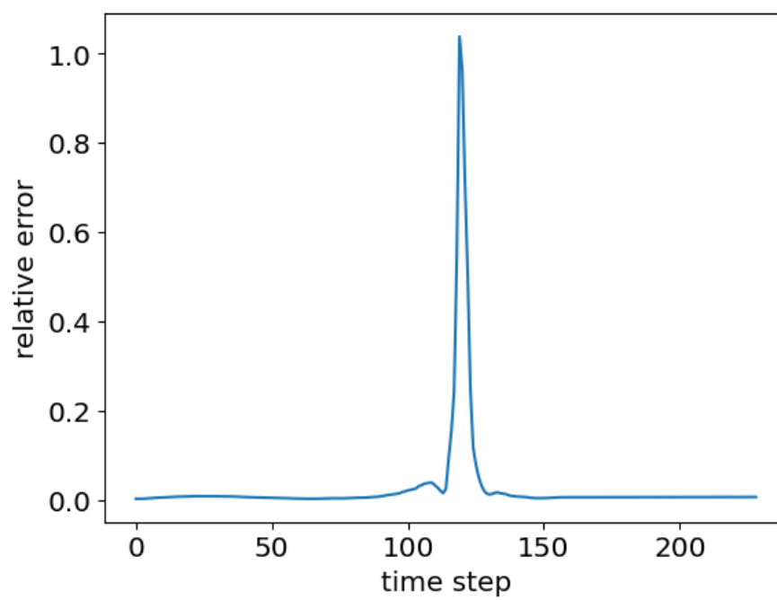
Figure 9: Relative error over one period for the electric field component obtained with the AVG-DG-GCA method.
