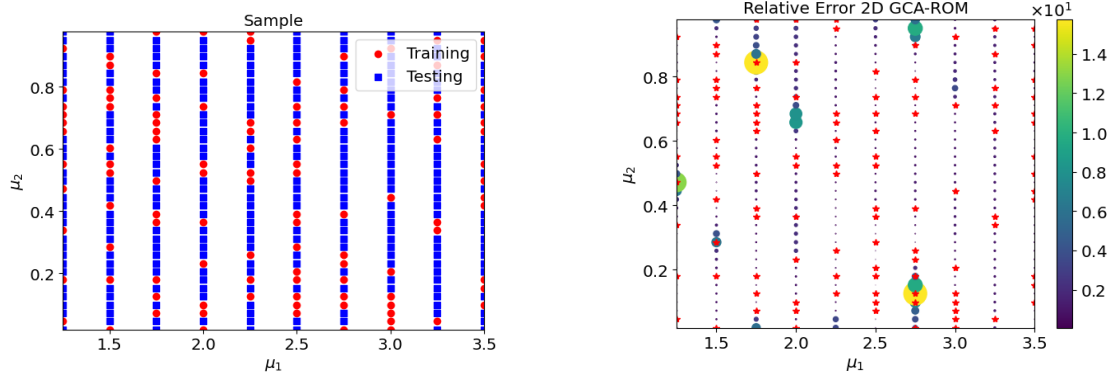
Figure 14: Dataset partitioning in training and testing set (left) and relative error (right).
