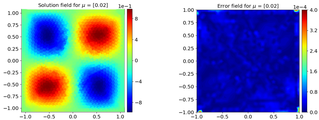
Figure 12: Solution field and error field obtained with the DC-GCA method with P_1 elements for the component E_Z at time t = 0.02 .
