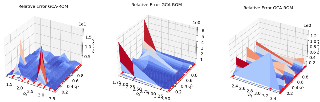
Figure 15: Relative error for the electric field over the parameter space \mathcal{P} = [1.25, 3.5] \times [0, 1] (left), \mathcal{P} = [1.75, 3.5] \times [0, 1] without critical values for \varepsilon_1 (center) and \mathcal{P} = [2.25, 3.5] \times [0, 1] (right).
