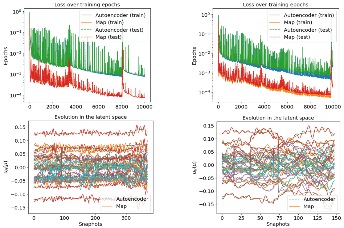
Figure 17: Loss and latent space for the training of the AVG-DG-GCA method over all the parameter space \mathcal{P} = [1.25, 3.5] \times [0, 1] (left) and \mathcal{P} = [1.75, 3.5] \times [0, 1] without critical values for \varepsilon_1 (right).
