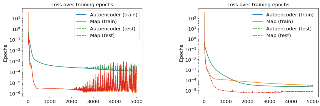
Figure 11: Loss evolution for P_1 and P_2 elements (2310 graph nodes), with MinMax scaling function (sample scaling) for the DG-GCA method.
