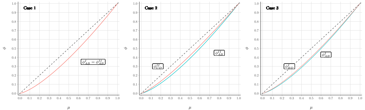
Figure 1: Illustration of the pmatchers for the three scenarios of Section 2.3
