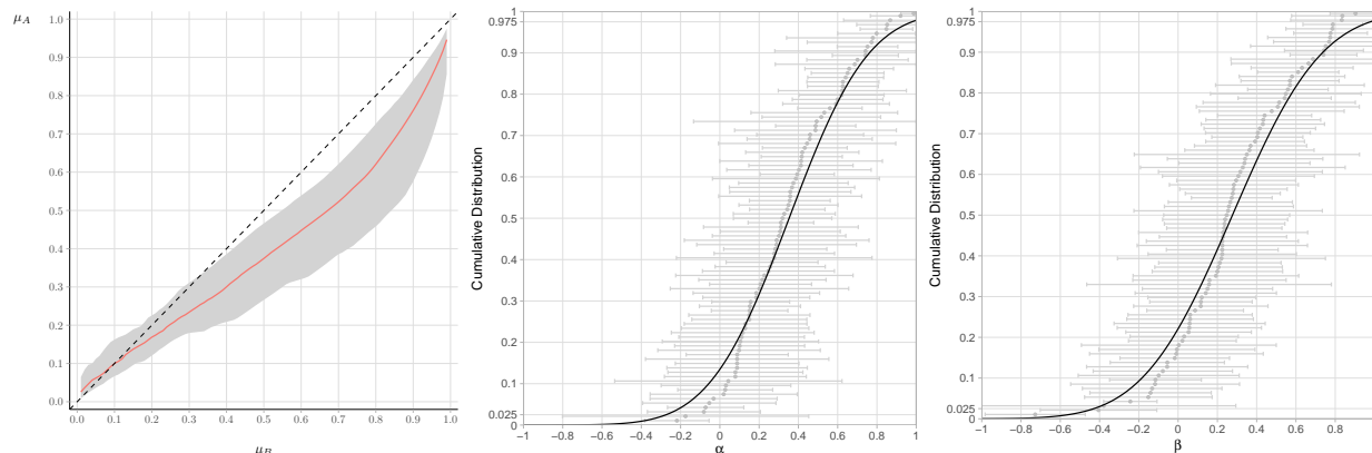
Note: the left panel plots the median \phi (plain red line) and its IQR (grey area). The middle (resp. right) panel plots the estimated distribution of \alpha (resp. \beta ) with plain lines and individual estimates and their 90% CI in grey.
