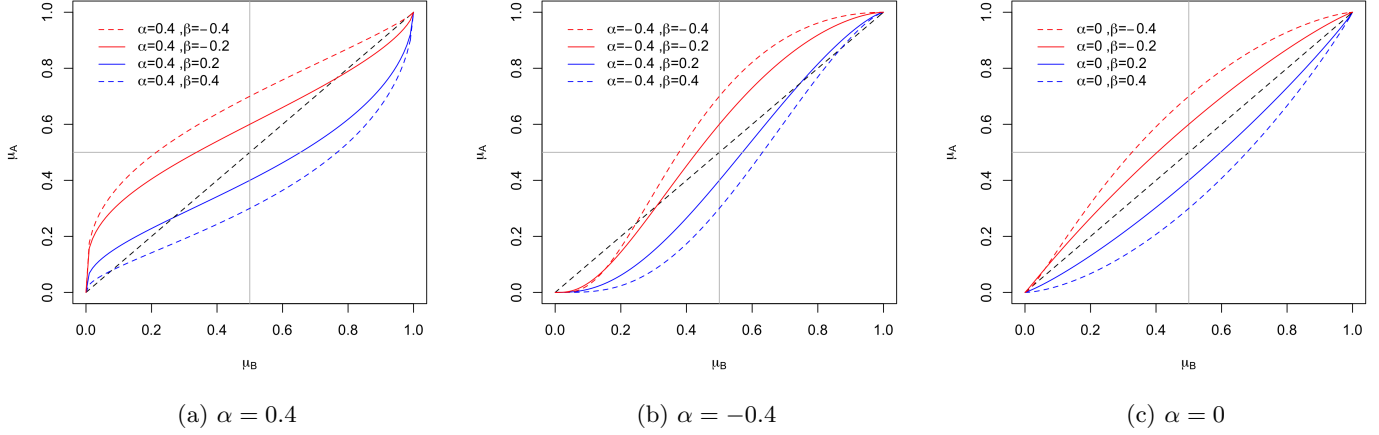
Figure 2: Illustration of the function \phi
