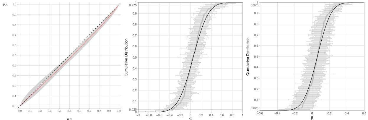
Figure 5: pmatcher \phi_{AB} and estimated distributions of its two parameters (Study C)
