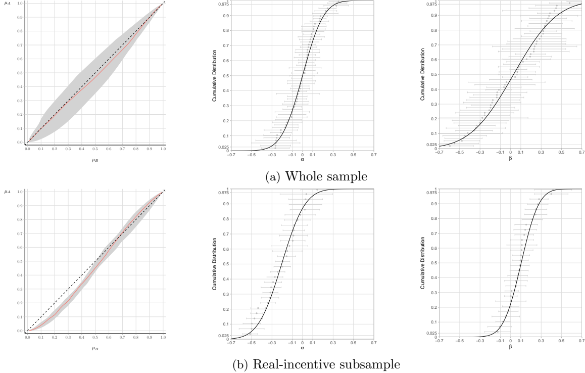
Note: the left panel plots the median \phi (plain red line) and its IQR (grey area). The middle (resp. right) panel plots the estimated distribution of \alpha (resp. \beta ) with plain lines, and individual estimates and their 90% CI in grey.
