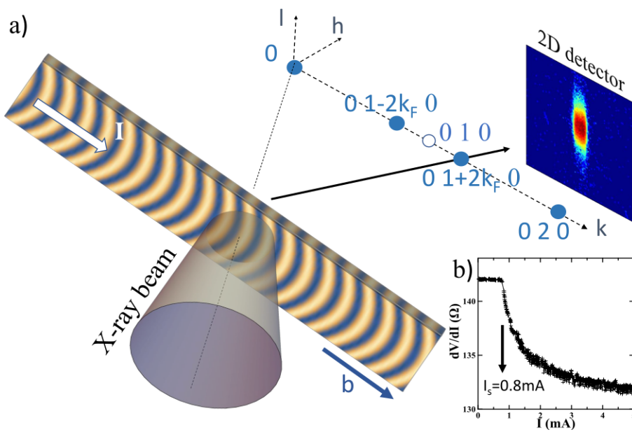
Fig. 1. Sketch of the experimental setup. (A) The bended CDW in NbSe 3 probed by diffraction in wide angle configuration as well as the corresponding reciprocal lattice. The external current is applied along the 2\mathbf{k}_F wave vector, parallel to the b axis. (B) NbSe 3 differential resistance measured during the experiment showing a threshold current equal to I_S=0.8\text{mA} .
