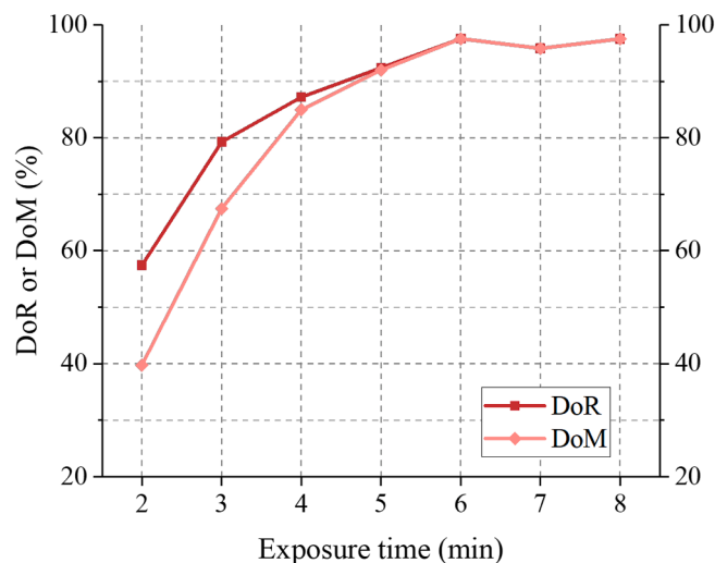
Fig. 4. Degree of reduction (DoR) and degree of metallization (DoM) of hematite disks samples exposed to the luminous flux for different time durations.
