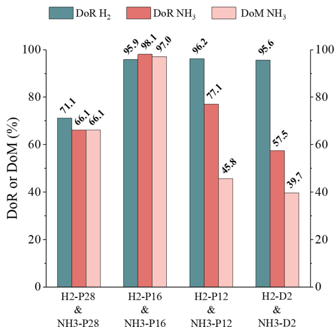
Fig. 3. Degree of reduction (DoR) or degree of metallization (DoM) of different samples reduced by H 2 (green) or NH 3 (red). For NH 3 the DoR and DoM are different and are represented in dark and light red respectively. The samples are, from left to right, pellets exposed for 28 min to the light flux, pellets exposed for 16 min with one rolling-over, pellets exposed for 12 min with three rolling-over and disks exposed for 2 min. (For interpretation of the references to colour in this figure legend, the reader is referred to the web version of this article.)
