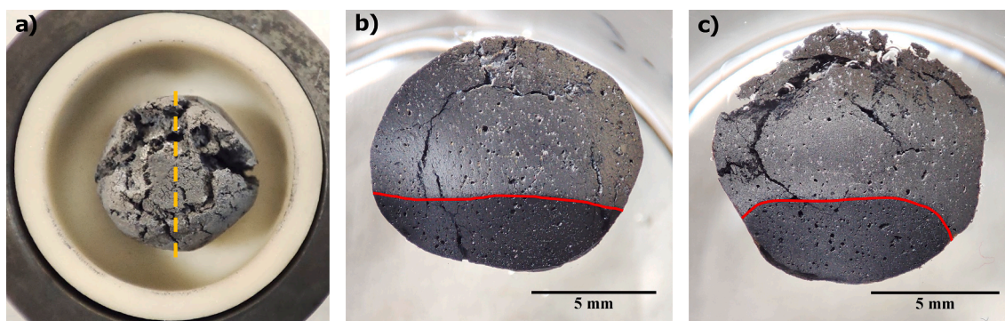
Fig. 2. a) top view of NH3-P28 pellet before cutting. the dashed yellow line corresponds to the cut line. Optical micrographs of b) H2-P28 and c) NH3-P28 pellets after their cut. The red line corresponds to the reduction front: the material above the line is iron whereas it is iron oxide below the line. (For interpretation of the references to colour in this figure legend, the reader is referred to the web version of this article.)
