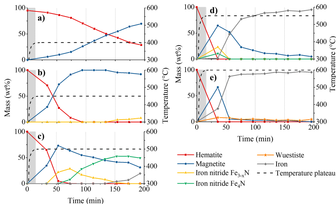
Fig. 1. Phase evolution as a function of time for different temperatures (a) 400 °C, b) 450 °C, c) 500 °C, d) 550 °C and e) 600 °C). Temperature is in dashed black line and the rising time has been greyed out.
