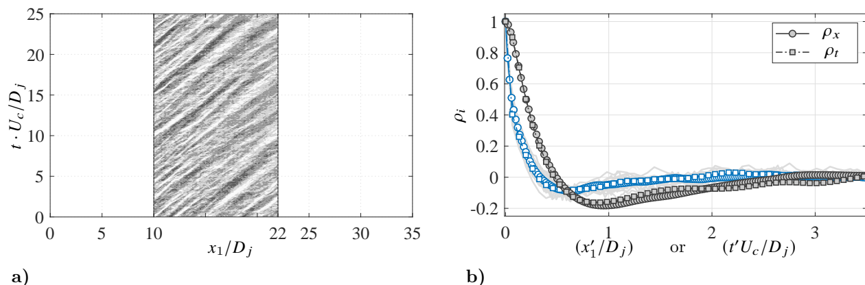
Figure 4: a) Experimental schlieren of Mach waves convecting through space and time at x_2/D_j = 4.0 . b) Space-delay ( \rho_x ) and time-delay ( \rho_t ) correlation coefficients at various points between 10 \leq x_1/D_j \leq 22 computed using experimental (closed symbols) and numerical (open symbols) databases.
