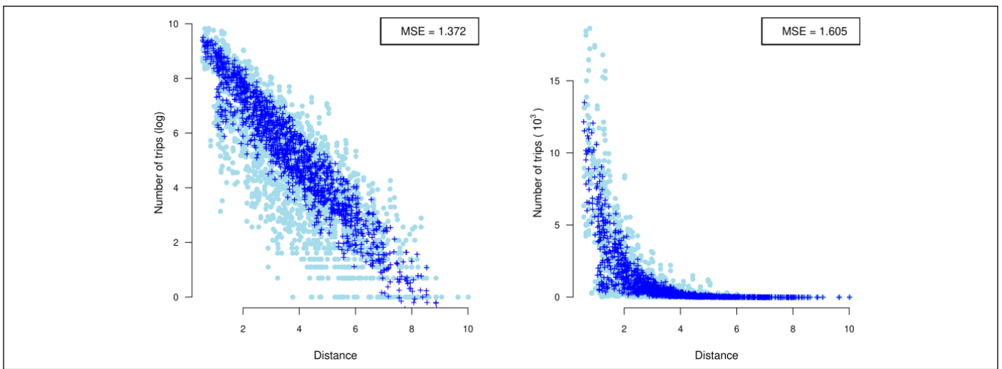
Figure 4: Comparison of the number of trips (light blue) and fitted values (dark blue) as a function of distance in the Poisson exponential gravity model, with a y -axis in logarithmic scale (left) and regular scale (right).
