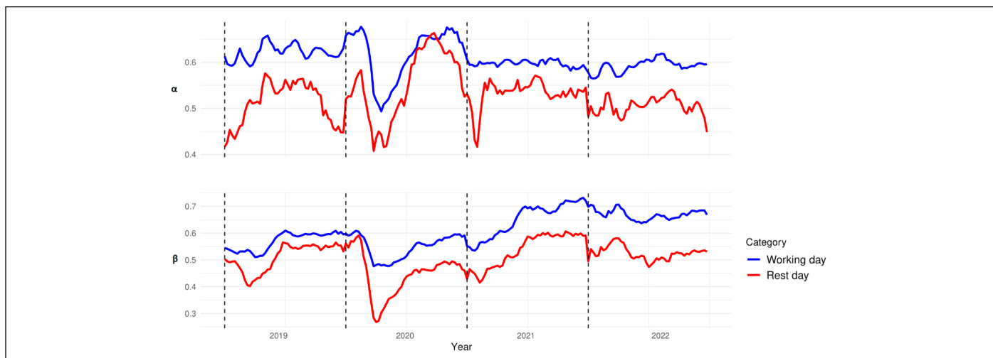
Figure 9: Evolution of the estimated \alpha and \beta coefficient in function of the week of Philadelphia.
