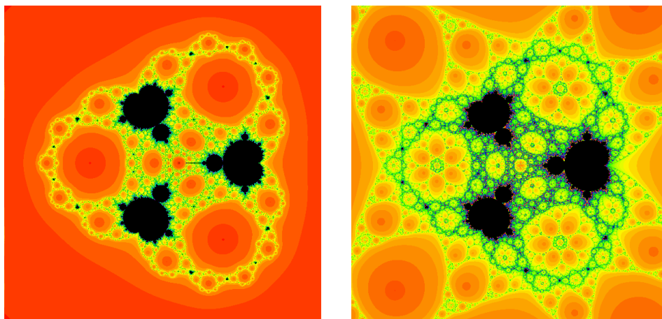
FIGURE 2. In the left side we show the parameter plane of M_\lambda (6) and in the right side the parameter plane of R_a (1) near a = 0 .
