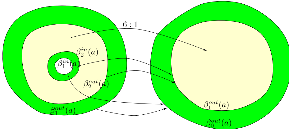
FIGURE 9. Sketch of the dynamics of the curves \beta_1^{in}(a) , \beta_2^{in}(a) , \beta_0^{out}(a) , \beta_1^{out}(a) , and \beta_2^{out}(a) .
