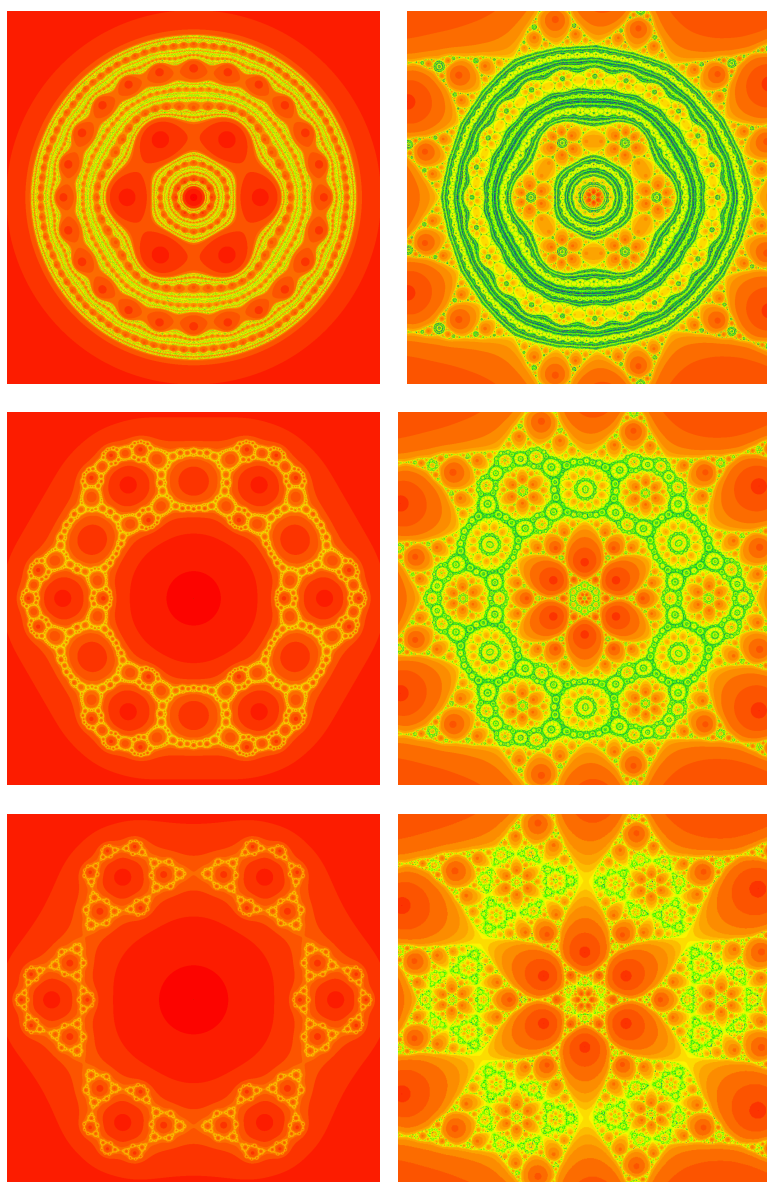
FIGURE 3. In the first column we show the dynamical plane of M_\lambda (6) for \lambda = 0.005 (top) \lambda = -0.28 (middle) and \lambda = -0.455 (bottom). In the second column the dynamical plane of R_a (see (1)) for a = -0.0003 (top) a = -0.0164 (middle) and a = -0.028 (bottom) with \text{Re}(z) \in (-0.245, 0.245) and \text{Im}(z) \in (-0.245, 0.245) . In the dynamical plane of R_a red points represent points converging to a third root of unity while in the McMullen family M_\lambda red points represent points converging to infinity.
