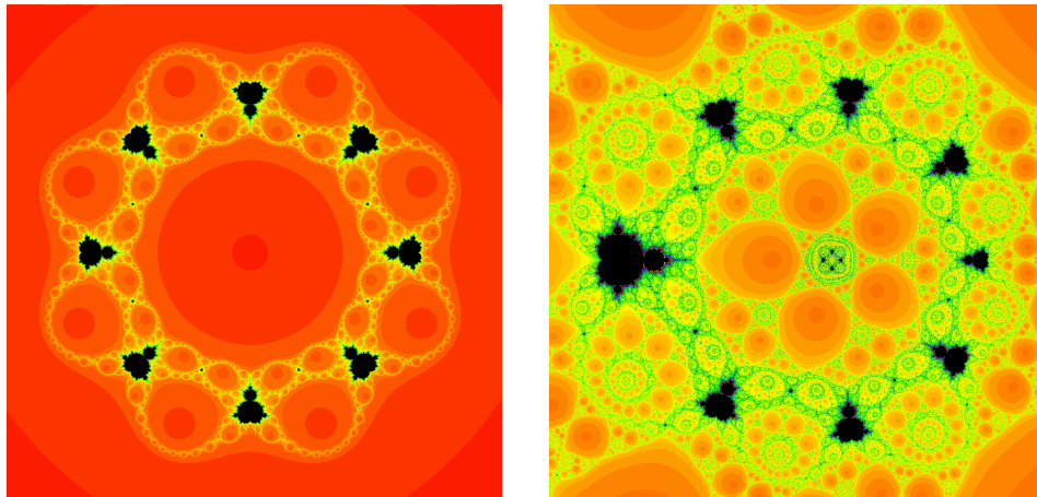
FIGURE 10. In the left side we show the parameter plane of M_{9,3,\lambda} and in the right side the parameter plane of O_{4,\alpha} near \alpha = 7/6 .
