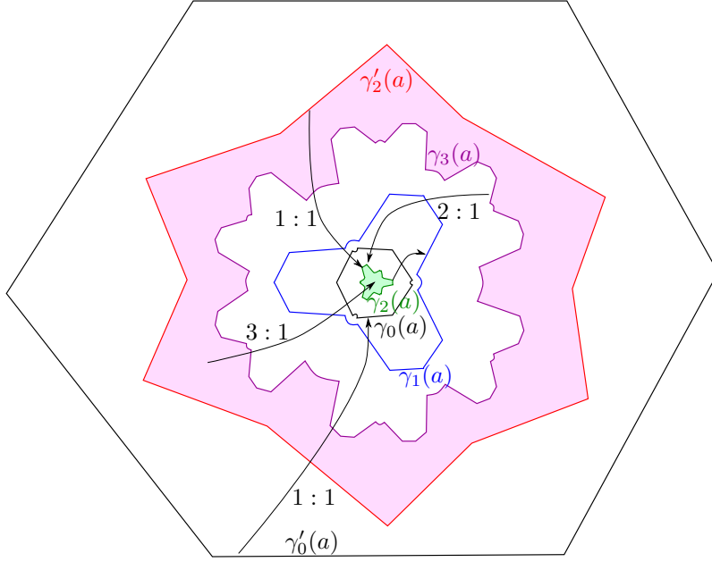
FIGURE 8. Sketch of the dynamics described in Proposition 15. The pink annulus contains three critical points and is mapped onto the green disc.
