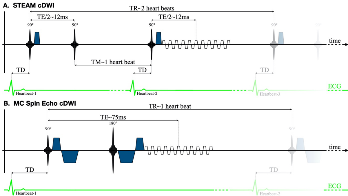
Figure 2: Cardiac Diffusion-Weighted Sequences. The two most common cardiac diffusion-weighted (cDWI) pulse sequences both use ECG triggering, diffusion-weighting gradients (dark blue) and single-shot echo-planar imaging (EPI) readouts. (A) Stimulated echo acquisition mode (STEAM) cDWI uses smaller diffusion-encoding gradients and longer diffusion mixing times (TM), which requires two heartbeats per image. (B) Motion-compensated spin echo (MCSE) uses larger diffusion-encoding gradients applied within a single heartbeat.
