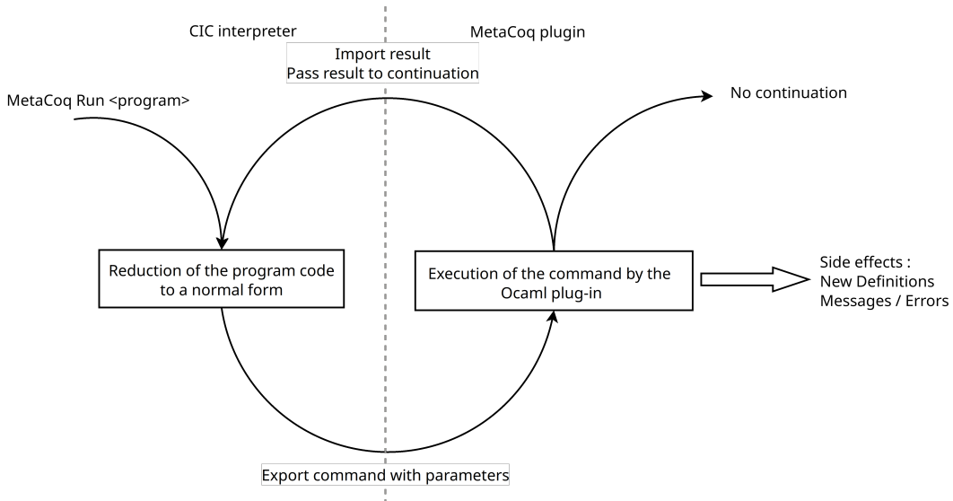
Figure 1. Sequential execution of a MetaCoq Run.
