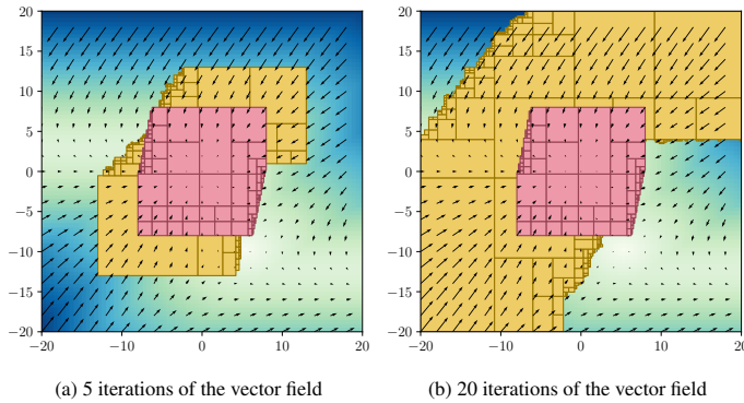
Figure 10: Capture basin computation
