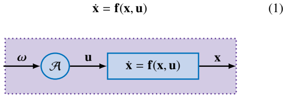
Figure 3: Block diagram of the system controlled by a timed automaton
