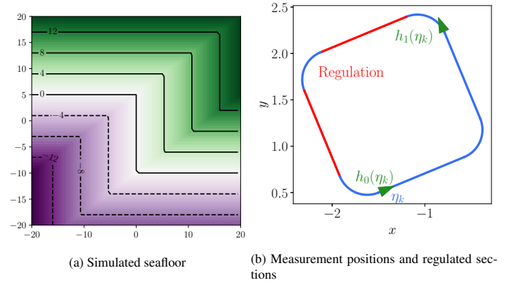
Figure 5: Simulated seafloor and measurements along the cycle
