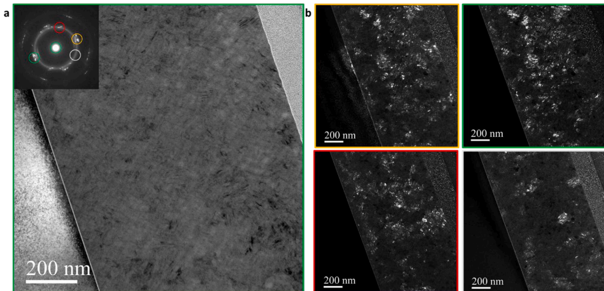
Fig. 4. (a) BF-TEM micrograph and corresponding SAED pattern for the Cantor alloy thin film with 10 at% Ag. (b) Dark field TEM micrographs.
