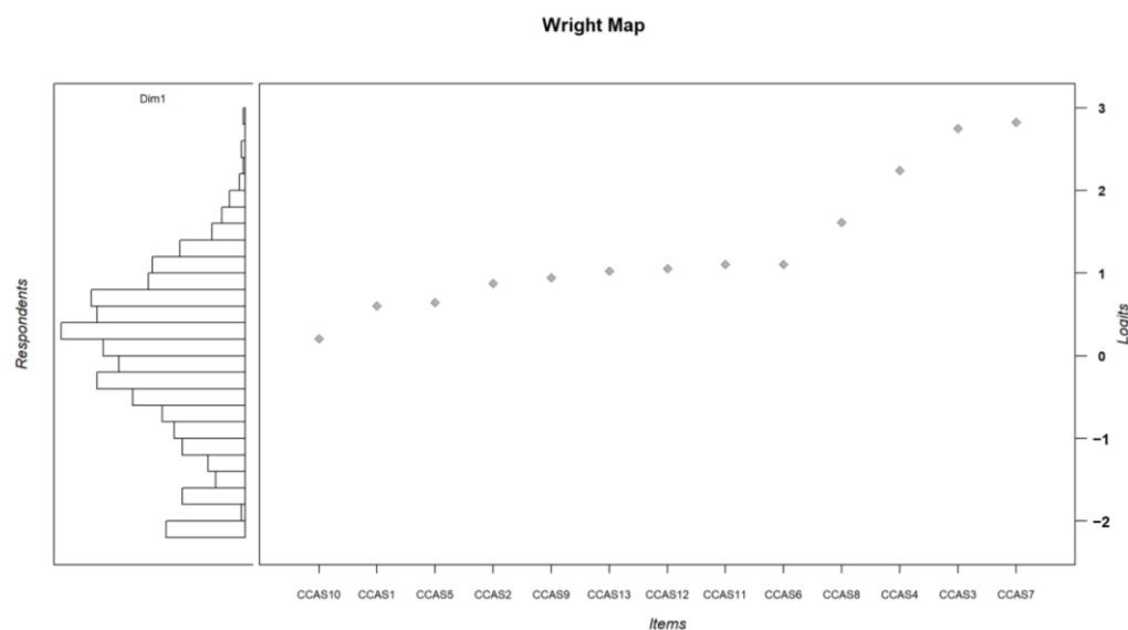
Figure 3. Wright map: comparison between persons' scores and general items difficulty. Right panel: items are sorted by their general level of difficulty. Left panel: persons' latent trait level of eco-anxiety.
