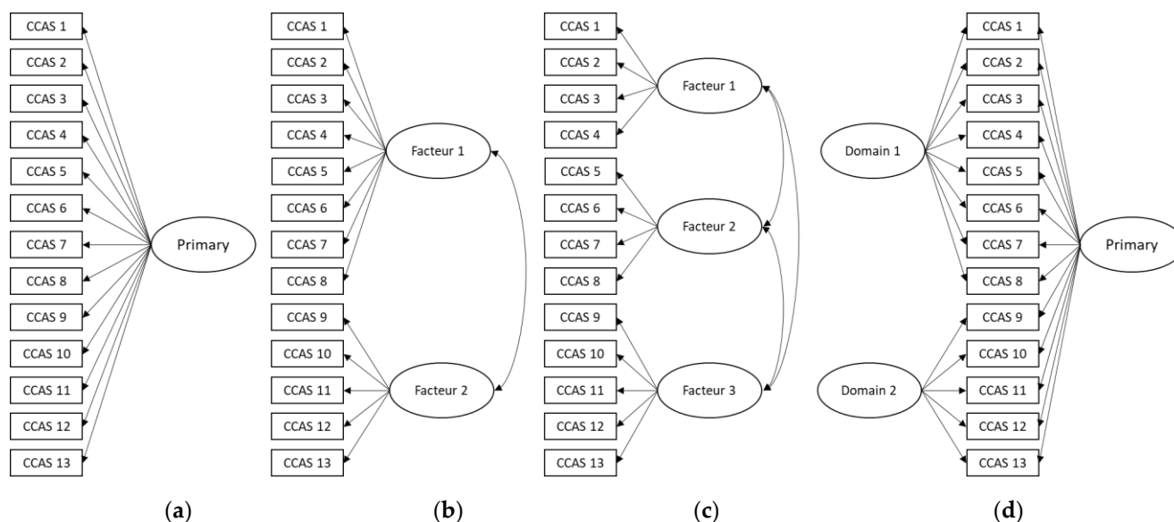
Figure 1. The four models tested in this study: (a) unidimensional model, (b) correlated 2 factor model, (c) correlated 3 factor model, and (d) bifactor model.
