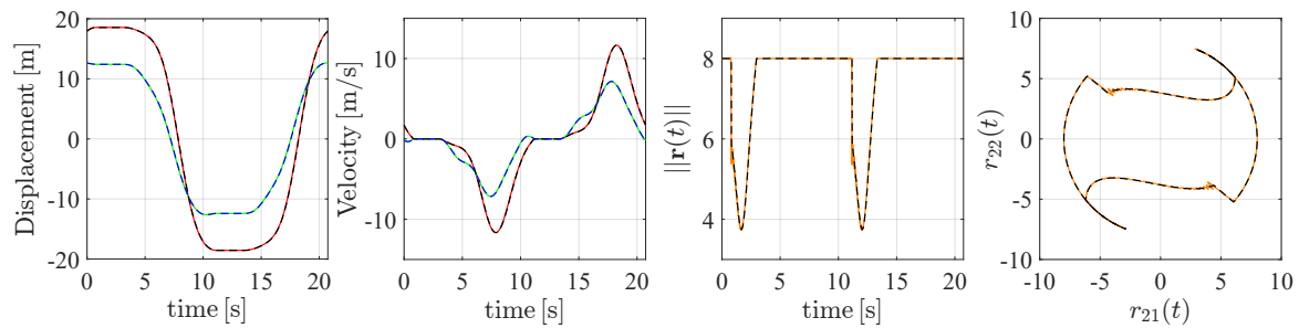
Fig. 22: Comparison of the response of damper mass m_2 using the E-WR method with N_\phi = 160 and implicit Euler time integration, at \omega = 0.303 , for \mu N = 8 and N_\phi = 160 . Displacements and velocities: E-WR [red] and Euler [black] in \mathbf{i}_1 direction; E-WR [green] and Euler [blue] in \mathbf{i}_2 direction. Friction force: E-WR [orange] and Euler [black].
