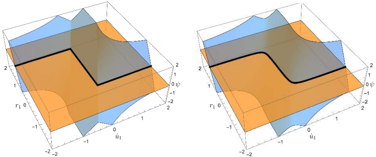
Fig. 2: 1D equality-based version of Coulomb's friction in direction \mathbf{i}_1 only (that is r_2 = \dot{u}_2 = 0 in Equation (2)), for illustration purposes: [blue] \Psi(r_1, \dot{u}_1) = r \max(\mu N, |r_1 - \rho \dot{u}_1|) - \mu N(r_1 - \rho \dot{u}_1) , [orange] 0 plane, [solid black line] dry friction solution set seen as the zero-level set of the function \Psi , that is the set (r_1, \dot{u}_1) satisfying \Psi(r_1, \dot{u}_1) = 0 ; [left] nonsmooth function \Psi involving the max operator; [right] set-valued regularization of \Psi where \max \approx \max_\epsilon through Equation (17) with \epsilon = 0.1 : stiffening is avoided.
