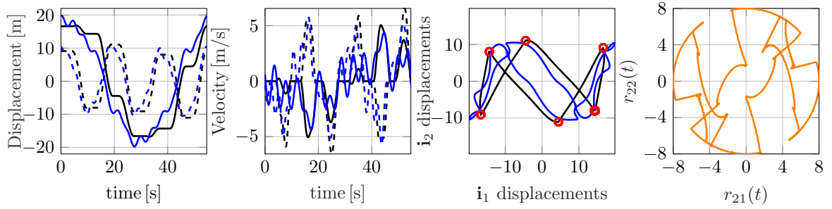
Figure 21: Response at \omega = 0.115 , for \mu N = 8 and N_\phi = 1800 , to multi-frequency excitation f_{11}(t) = 20 \cos \omega t and f_{12}(t) = 20 \cos 3\omega t . Displacement and velocity plots indicate mass m_1 [blue] and mass m_2 [black]. Time histories of displacement and velocity indicate the \mathbf{i}_1 -direction DOF [solid line] and \mathbf{i}_2 -direction DOF [dashed line].
