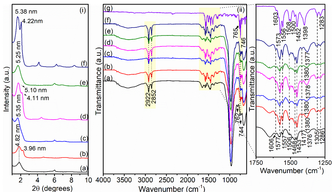
Figure 11.2 (i) XRD patterns and (ii) FTIR spectra of (a) C 14 -Ver-100%, (b) C 14 -Ver-200%, (c) C 16 -Ver-100%, (d) C 16 -Ver-200%, (e) C 18 -Ver-100%, and (f) C 18 -Ver-200% after diclofenac adsorption, (25 °C, pH 6.0 or 8.0 and C i = 500 mg L -1 ) and g) free diclofenac sodium.
