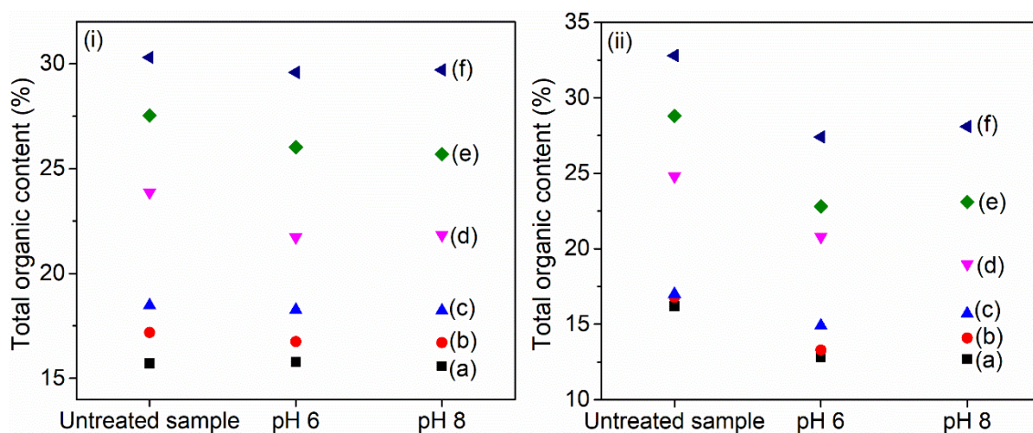
Figure 10. Total organic content of (a) C 14 -Ver-100%, (b) C 16 -Ver-100%, (c) C 18 -Ver-100%, (d) C 14 -Ver-200%, (e) C 16 -Ver-200% and (f) C 18 -Ver-200% before and after stability test at pH 6.0 and 8.0 determined by (i) CHN, and (ii) TG/DTG.
