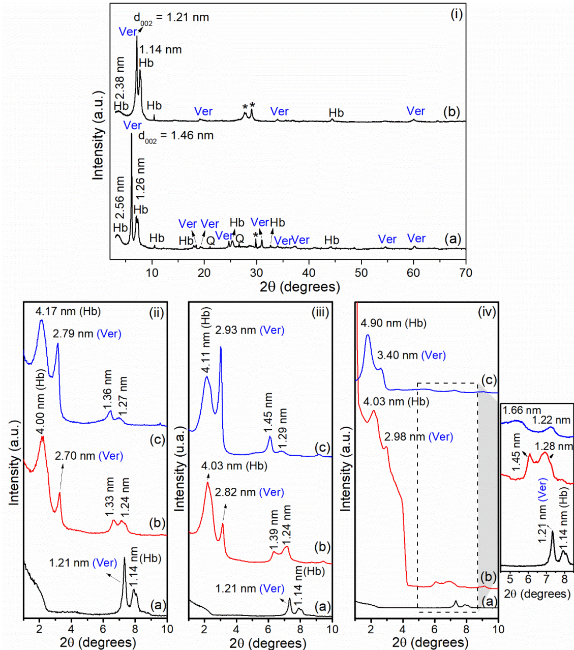
Figure 1. XRD patterns of (i): (a) Ca, Mg-Ver, and (b) Na-Ver (Ver = vermiculite, Hb = hydrobiotite, Q = quartz, *unidentified phase); (ii): (a) Na-Ver, (b) C 14 -Ver-100%, and (b) C 14 -Ver-200%; (iii): (a) Na-Ver, (b) C 16 -Ver-100%, and (b) C 16 -Ver-200%; and (iv): (a) Na-Ver, (b) C 18 -Ver-100%, and (b) C 18 -Ver-200%.
