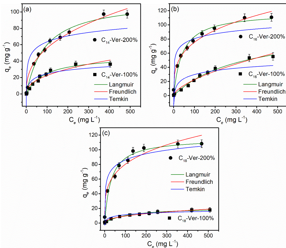
Figure 9.1 Equilibrium isotherms and their fit to the Langmuir, Freundlich and Temkin models for the adsorption of diclofenac sodium by organo-vermiculites (a) C 14 -Ver, (b) C 16 -Ver, and (c) C 18 -Ver at 25 ° C (pH 6.0 or 8.0, 25 °C and C_i = 1 - 500 mg L -1 ).
