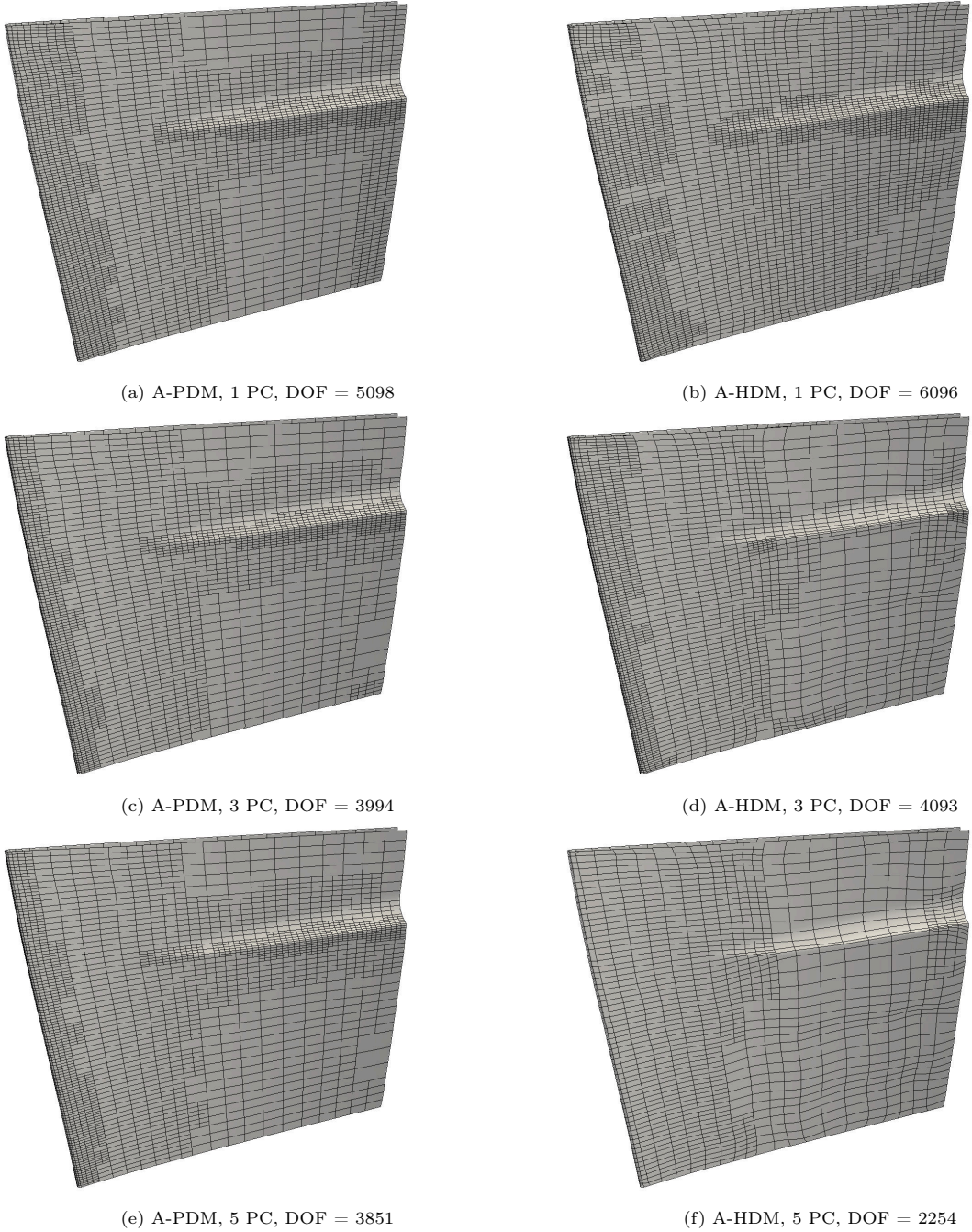
Figure 11: Blade geometry reconstruction from Section 6.1 for a varying number of PC steps (increasing from top to bottom) for A-PDM (left column) and A-HDM with error-based weights suggested in [38] (right column). The dimension of each geometric model (DOF) is also reported.
