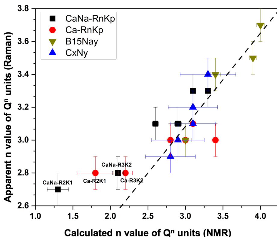
Figure 6. Comparison of average (apparent) n value of Q^n units determined via NMR and Raman methods (dashed line represents the correlation line of this two methods). The error bars were determined from standard deviation calculation and also replicated measurements.
