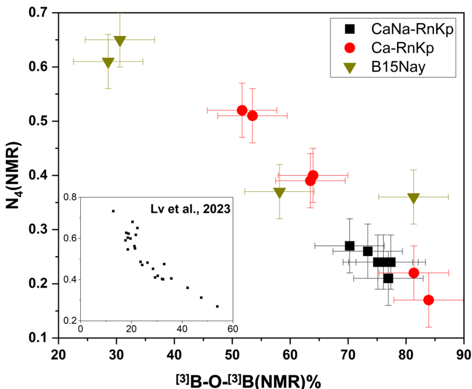
Figure 8. Plots of ^{13}\text{B-O-}^{13}\text{B} % values plotted against N_4 values of our investigated glasses as determined from NMR results: 1\text{D }^{11}\text{B} spectrum fitting for N_4 and DQ-SQ DQ projection for ^{13}\text{B-}^{13}\text{B} %. The inset contains data obtained from the literature (Lv et al., 2023 [ 12 ]), which shares the same axis units as the main figure.
