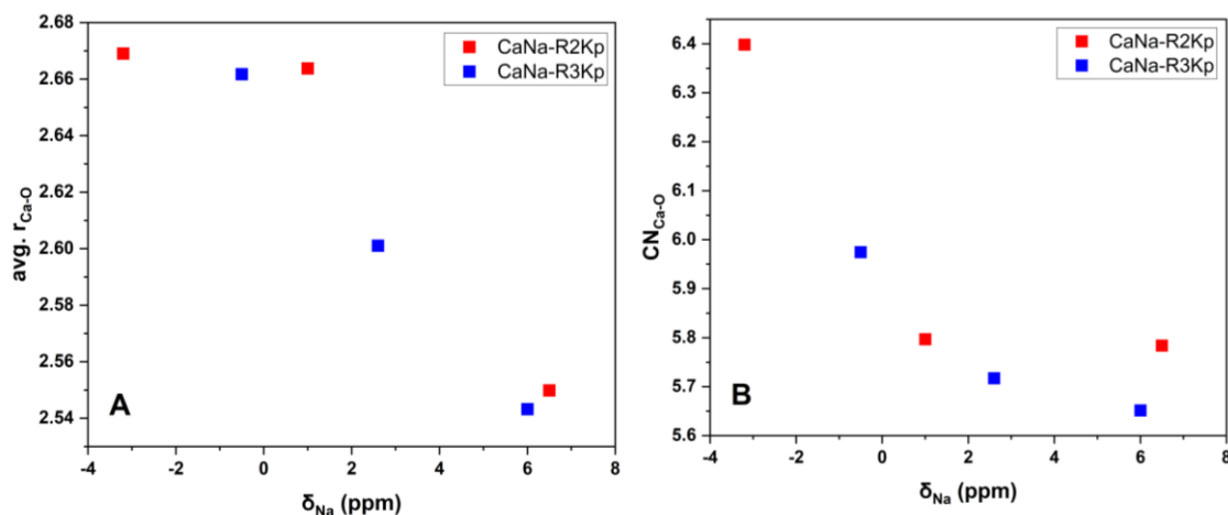
Figure 9. Relationship between Na environment obtained by NMR spectroscopy and Ca environment obtained by XAS spectroscopy in the CaNa-RnKp glass series. The average distance of Ca-O (A) and the coordination number of Ca-O (B) against the chemical shift of ^{23}\text{Na} .
