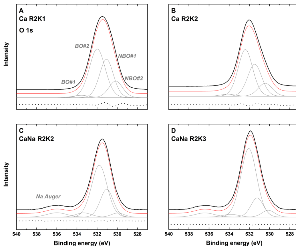
Figure 2. Examples of XPS O 1s spectra (in black) and the associated fit (in red) for Ca-R2K1 (A), Ca-R2K2 (B), CaNa-R2K2 (C) and CaNa-R2K3 glasses. The spectra are fitted with two peaks for BO species and two peaks for NBO species. In addition, for Na-bearing glasses, there is a peak at 536 eV corresponding to the Na Auger line. The residual from the fit is also reported (dotted line at bottom).
