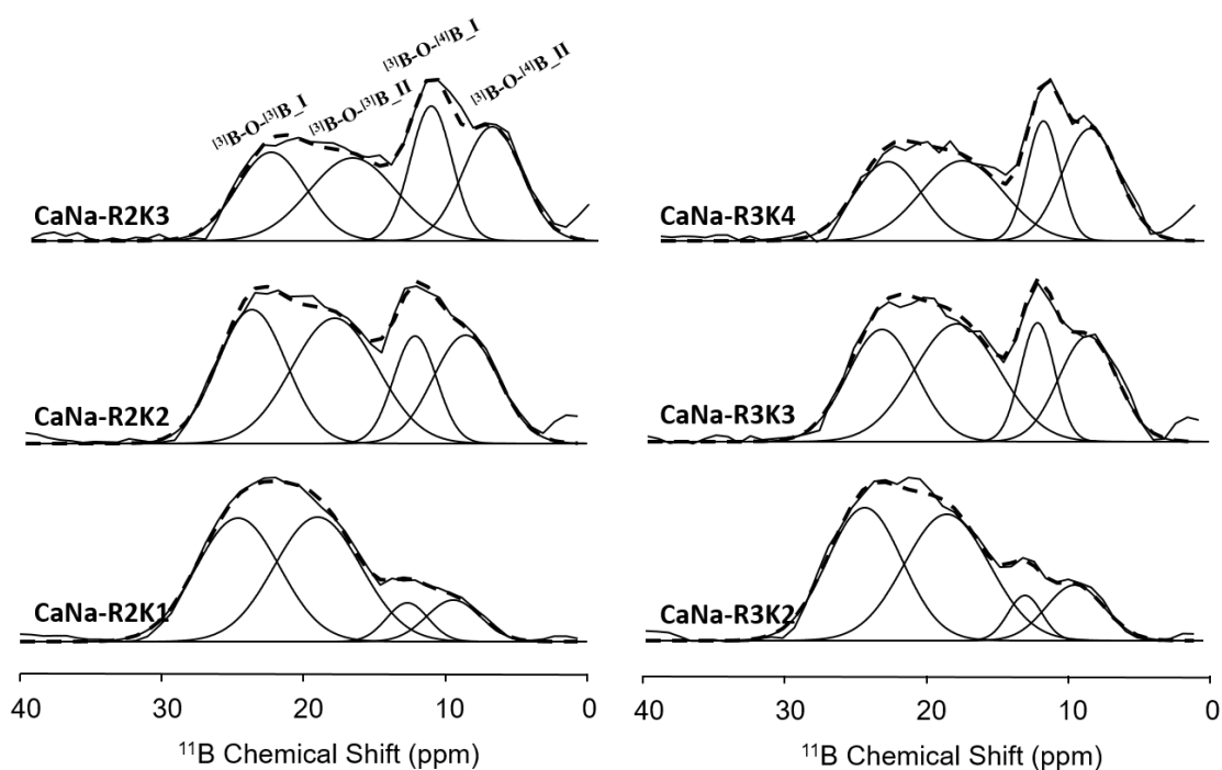
Figure 5. DQ projection of ^{11}\text{B} DQ-SQ NMR maps of CaNa-RnKp glass series (dashed lines represent the decomposition spectra of ^{[3]}\text{B-O-}^{[3]}\text{B} and ^{[3]}\text{B-O-}^{[4]}\text{B} correlations using full Gaussian peaks ( G/L = 1 ); two lines for reproducing ^{[3]}\text{B-O-}^{[3]}\text{B} species and two lines for ^{[3]}\text{B-O-}^{[4]}\text{B} species).
