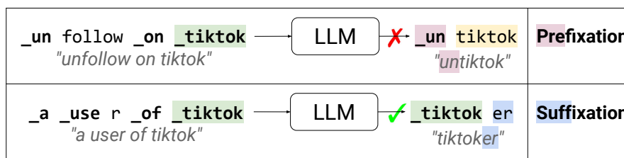
Figure 7: In BPE tokenization, marking word-initial tokens with “_” hinders the generation of prefixed forms (e.g., “_un tiktok”), as they do not share any token with their base (e.g., “_tiktok”). Identical tokens are highlighted in the same color.
