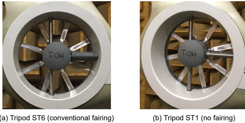
FIGURE 14 – Different drive shaft fairings
