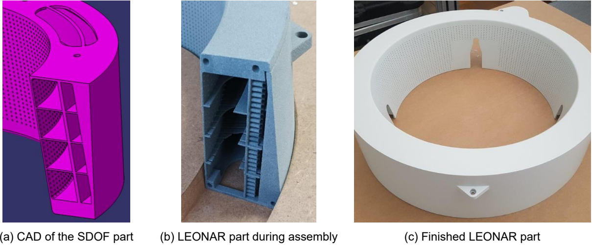
FIGURE 13 – Manufacturing process for the diffuser parts
