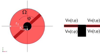
FIGURE 2 – Top view of the propeller disk (left) and equivalent source distribution for thickness noise on a cross section of the propeller disk (right).
