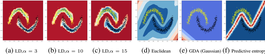
Figure 5.1: Methods for uncertainty estimation applied on the same neural net trained to classify 2 classes in moon-shape (represented by yellow and black points respectively). Uncertainty estimations are computed based solely on the feature space of the model without seeing directly the inputs. Red represents high uncertainty. Our method (Fig. 5.1a, 5.1b and 5.1c) gives excellent results and much better than other methods.
