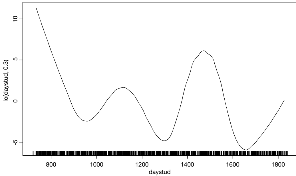
Deviation from mean Daily Deaths with span of 0.3
