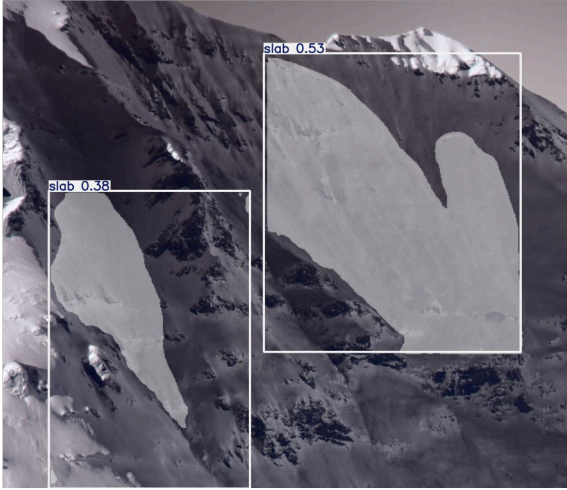
Figure 5: Catalogued slab avalanches (2023-12-03 at 3 PM).
