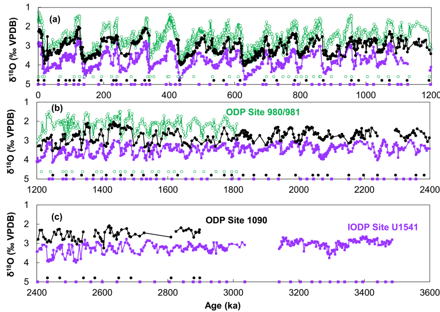
Figure 2. Benthic foraminiferal \delta^{18}\text{O} records based on Cibicidoides and Cibicides spp. from IODP Site U1541 (purple, squares), ODP Site 1090 (black, filled circles), and ODP Sites 980/981 (green, open circles). Data plotted using age models derived from manual alignment of each record to the LR04 global stack (Lisiecki and Raymo, 2005) for (a) 0–1200 ka, (b) 1200–2400 ka, and (c) 2400–3600 ka. The benthic foraminiferal \delta^{18}\text{O} records for ODP Site 1090 and ODP Site 980/981 are plotted with a -0.5\text{‰} shift and a -1.0\text{‰} shift, respectively, for clarity. Stratigraphic tie points for each manual alignment are denoted on the x axis (Table S1).
