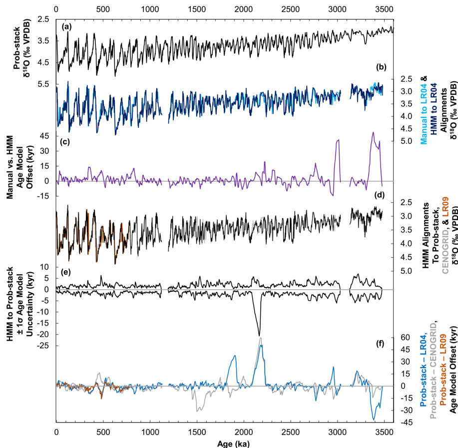
Figure 4. Stratigraphic benthic foraminiferal \delta^{18}\text{O} alignments for IODP Site U1541. (a) Prob-stack benthic foraminiferal \delta^{18}\text{O} target (Ahn et al., 2017) for comparison. (b) Manual (light blue) and automated HMM-Match-based (dark blue; Lin et al., 2014) alignments of the benthic foraminiferal \delta^{18}\text{O} record from IODP Site U1541 to the LR04 benthic foraminiferal \delta^{18}\text{O} stack (Lisiecki and Raymo, 2005). (c) Age model offset between the age models for IODP Site U1541 plotted in (b) . (d) Automated alignments of the benthic foraminiferal \delta^{18}\text{O} record from IODP Site U1541 to Prob-stack (black), CENOGRID (gray; Westerhold et al., 2020), and the LR09 Pacific stack (brown; Lisiecki and Raymo, 2009) using HMM-Match. (e) 1\sigma age model uncertainties reported by HMM-Match for the benthic foraminiferal \delta^{18}\text{O} alignment of IODP Site U1541 to Prob-stack. (f) Age offsets between the age models at IODP Site 1541 generated by the automated HMM-Match-based alignments to Prob-stack and LR04 (blue), Prob-stack and CENOGRID (gray), and Prob-stack and LR09 Pacific stack (brown). The zero line is plotted in (c) , (e) , and (f) for reference.
