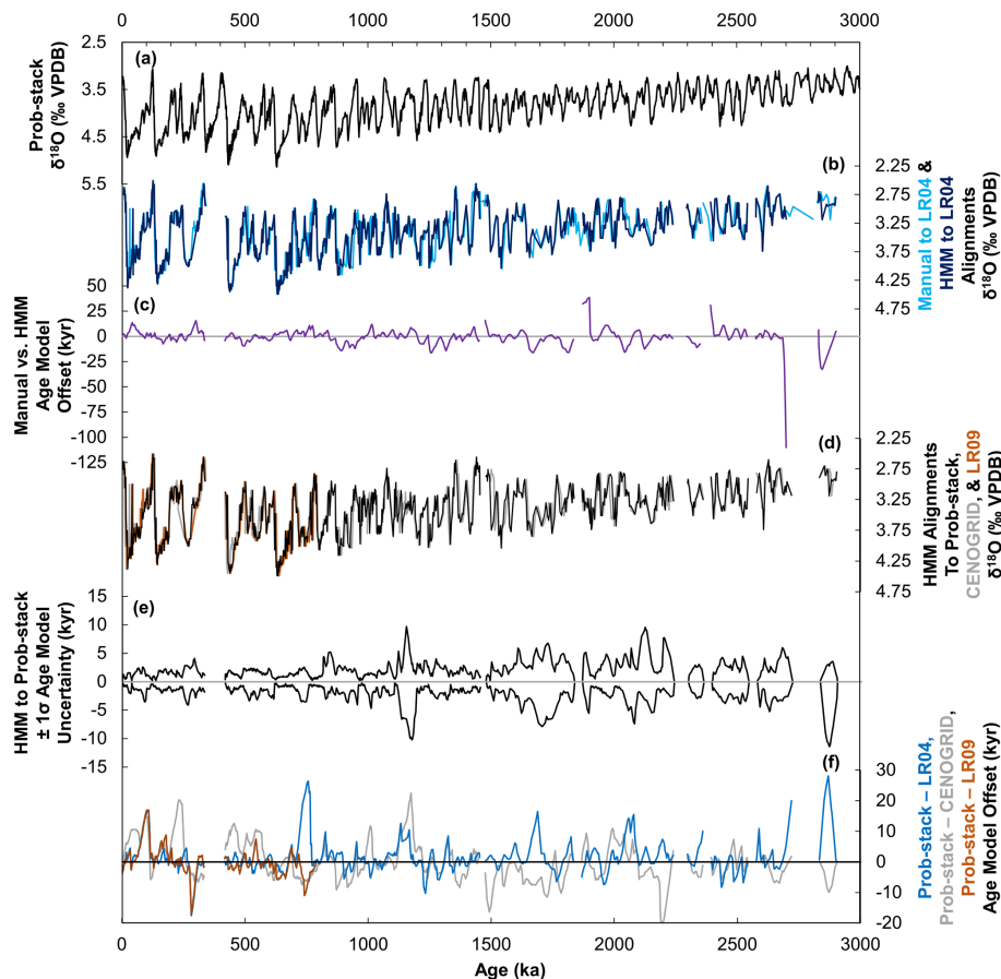
Figure 5. Stratigraphic benthic foraminiferal \delta^{18}\text{O} alignments for ODP Site 1090. (a) Prob-stack benthic foraminiferal \delta^{18}\text{O} target (Ahn et al., 2017) for comparison. (b) Manual (light blue) and automated HMM-Match-based (dark blue; Lin et al., 2014) alignments of the benthic foraminiferal \delta^{18}\text{O} record from ODP Site 1090 to the LR04 benthic foraminiferal \delta^{18}\text{O} stack (Lisiecki and Raymo, 2005). (c) Age model offset between the age models for ODP Site 1090 plotted in (b). (d) Automated alignments of the benthic foraminiferal \delta^{18}\text{O} record from ODP Site 1090 to Prob-stack (black), CENOGRID (gray; Westerhold et al., 2020), and the LR09 Atlantic stack (brown; Lisiecki and Raymo, 2009) using HMM-Match. (e) 1\sigma age model uncertainties reported by HMM-Match for benthic foraminiferal \delta^{18}\text{O} alignment of ODP Site 1090 to Prob-stack. (f) Age offsets between the age models at ODP Site 1090 generated by the automated HMM-Match-based alignments to Prob-stack and LR04 (blue), Prob-stack and CENOGRID (gray), and Prob-stack and LR09 Atlantic stack (brown). The zero line is plotted in (c), (e), and (f) for reference.
