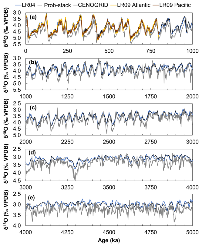
Figure 3. Selected benthic foraminiferal \delta^{18}\text{O} alignment target records over the past 5 Myr. Plotted targets include Prob-stack (black; Ahn et al., 2017), LR04 (blue; Lisiecki and Raymo, 2005), the CENOGRID splice (gray; Westerhold et al., 2020), and the LR09 Atlantic (yellow) and Pacific stacks (dark red; Lisiecki and Raymo, 2009) for (a) 0–1000 ka, (b) 1000–2000 ka, (c) 2000–3000 ka, (d) 3000–4000 ka, and (e) 4000–5000 ka.
