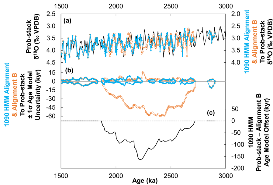
Figure 6. Comparison of age models at ODP Site 1090 generated by automated HMM-Match-based benthic foraminiferal \delta^{18}\text{O} alignments to Prob-stack using different segmentation. (a) HMM-Match-based benthic foraminiferal \delta^{18}\text{O} alignments to Prob-stack based on seven user-defined segments (blue; i.e., the standard 1090 HMM-Match alignment as plotted in Fig. 5) versus four user-defined stratigraphic segments (orange; ODP Site 1090 Alignment B) compared to the Prob-stack target (black). (b) 1\sigma age model uncertainties reported by the automated HMM-Match alignment algorithm for the standard alignment and Alignment B of ODP Site 1090 to Prob-stack. (c) Age model offset between the standard alignment and Alignment B of ODP Site 1090 to Prob-stack.
