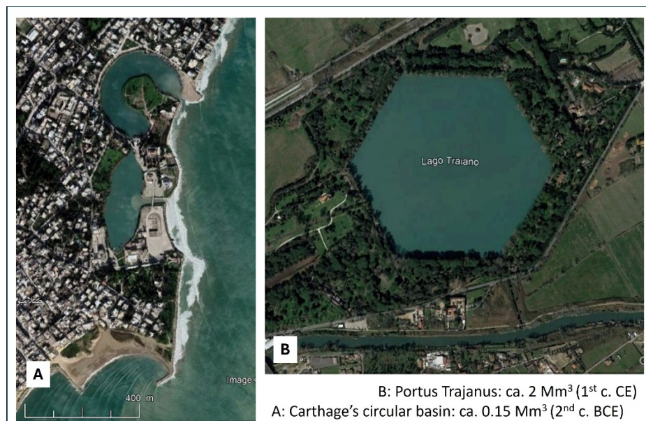
Figure 17. Dredging of Carthage's circular basin and Trajan's hexagonal basin. (Google Earth)
