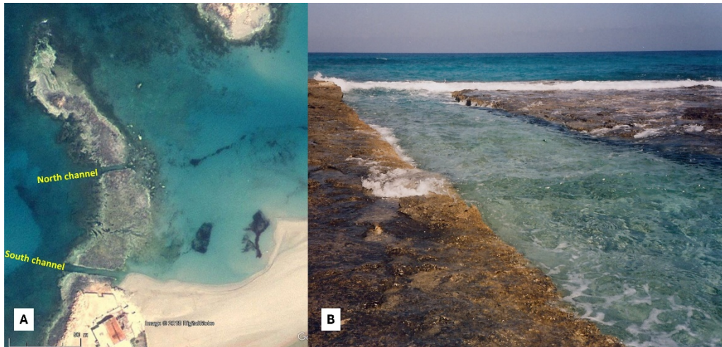
Figure 15. A: El-Hanieh harbour (Libya). B: northern flushing channel (Photo Misson, 5/10/2010).
