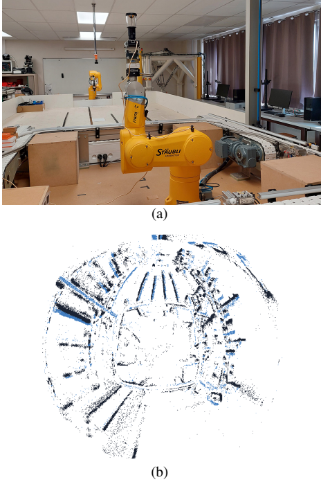
Figure 6. (a) Experimental setup: The catadioptric event camera is mounted on the end-effector of a Staubli TX-60 robot and observes the parallel lines in the environment. (b) Event frame captured by the catadioptric event camera, 2.5 seconds after the beginning of Sequence 1a (a pixel is blue if the polarity p_k = +1 , and black if p_k = -1 ).
