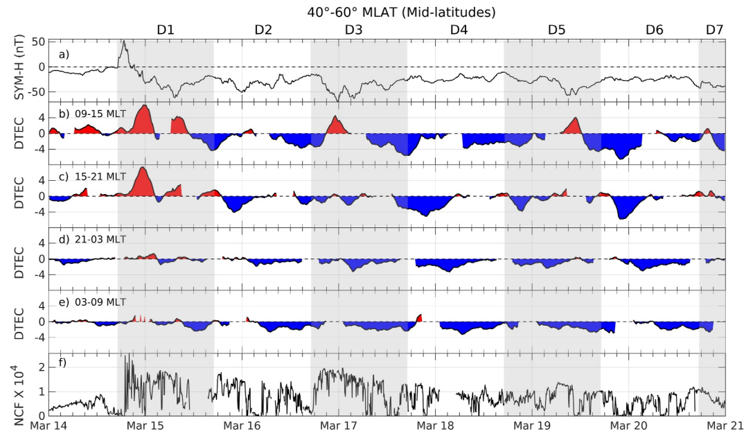
Figure 6. Same as Figure 4, but for the latitude range 40°–60° MLAT (mid-latitudes). Also panel (a) is changed to the SYM-H index and panel (f) to the Newell coupling function.
