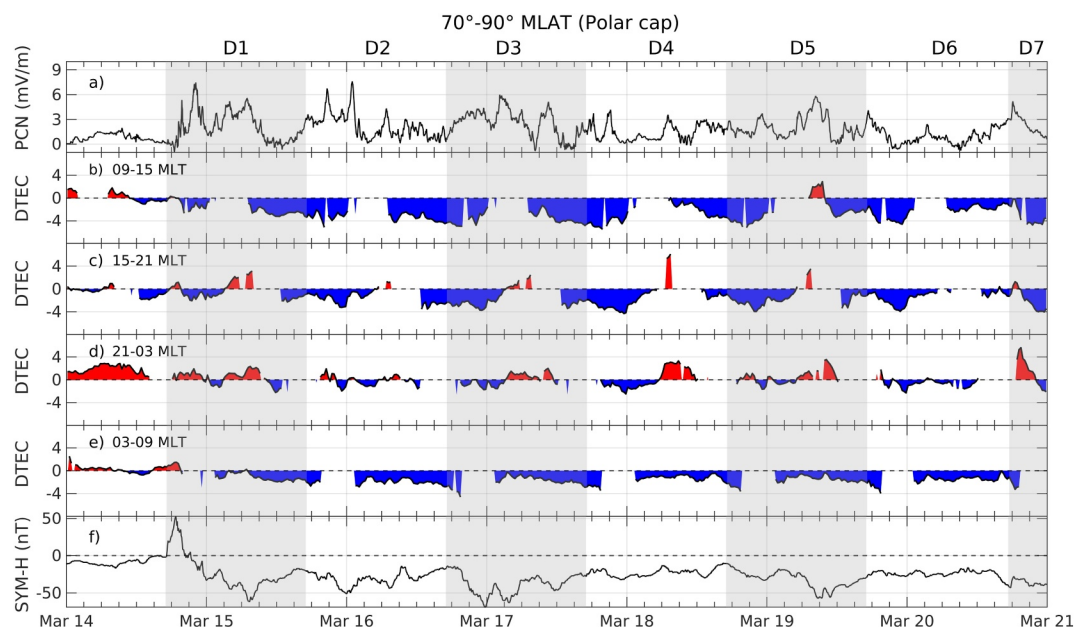
Figure 4. Parameters for 70°– 90° MLAT (polar cap). Panels from top to bottom: (a) PCN index. (b)–(e) DTEC (in unit of TECU) in the dayside (09–15 magnetic local time (MLT)), dusk sector (15–21 MLT), night sector (21–03 MLT) and dawn sector (03–09 MLT) (f) SYM-H index. The date numbers refer to 00 UT. The sequence of shaded and non-shaded periods indicate the days after the storm onset numbered D1–D7.
