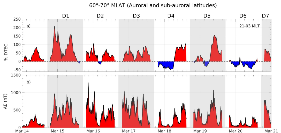
Figure 10. DTEC enhancements at 60^{\circ} – 70^{\circ} (auroral and sub-auroral latitudes in the night sector (21-03 MLT)). (a) DTEC in percentage, (b) AE index. For comparison, AE index is plotted only when there are sufficient data points in DTEC.
