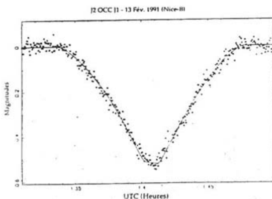
Symmetrical deep lightcurve with the fit
