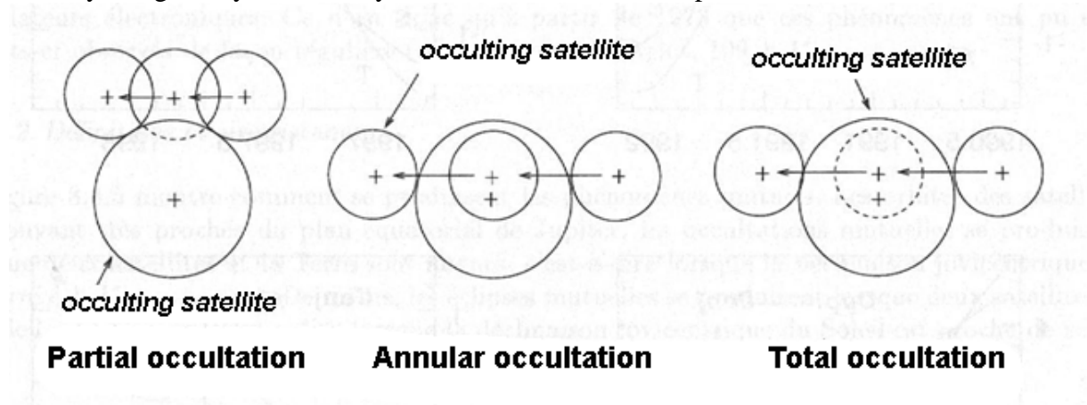
Figure: geometry of a mutual occultation
