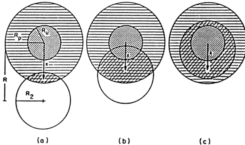
eclipse: (a) by penumbra; (b) partial; (c) annular (total if R_2 < R_u )
