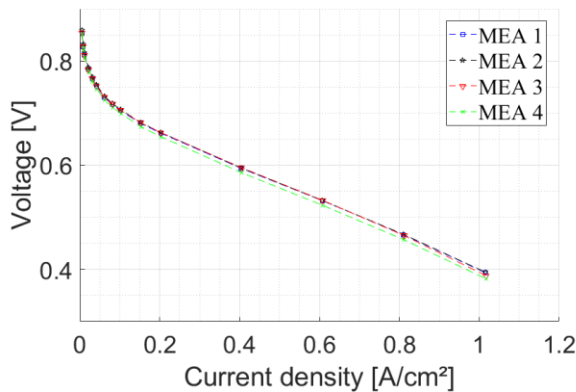
Fig. 6. Initial reference polarization curves of the 4 MEAs (cycle current profile v(i)_1 , 160 °C, in H 2 /AIR at 1.2/2 stoichiometries). Atmospheric pressures are given as an indication.
