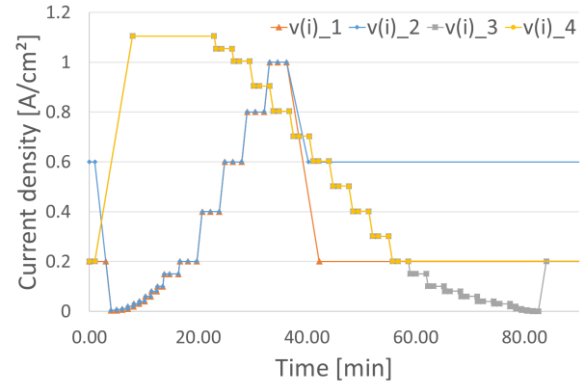
Fig. 4. Current profiles used for the four cycles.
