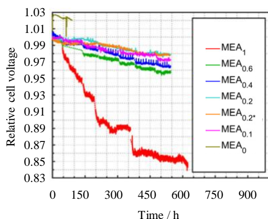
Fig. 1. Voltages referred to the initial voltage of 7 MEAs aging at different constant currents (from 0.1 to 1 A \cdot cm^{-2} , at 160 \text{ }^\circ C , in H_2/AIR at stoichiometries of 1.2/2 and without pressure regulation). The characterizations have been replaced by dotted lines for better lisibility. Figure from [16].
