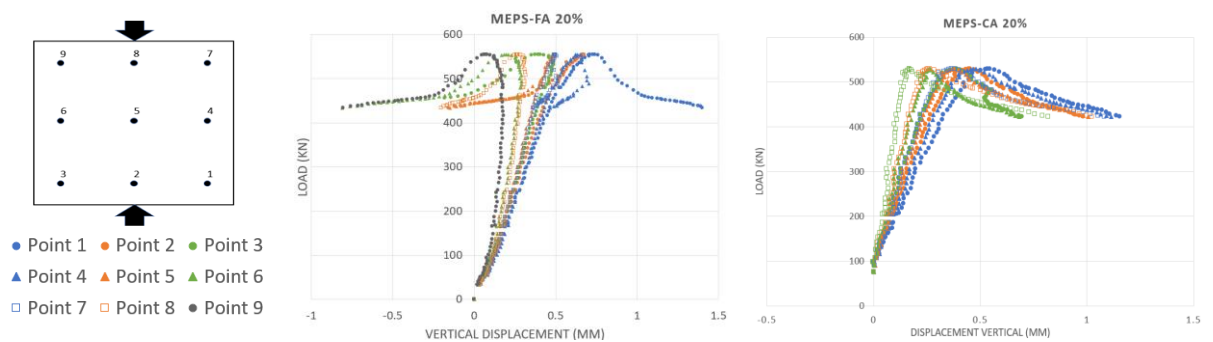
Figure 6 Load – v displacement (vertical displacement) response of using 20% MEPS material as a substitute for fine aggregate (FA) and coarse aggregate (CA) in concrete
