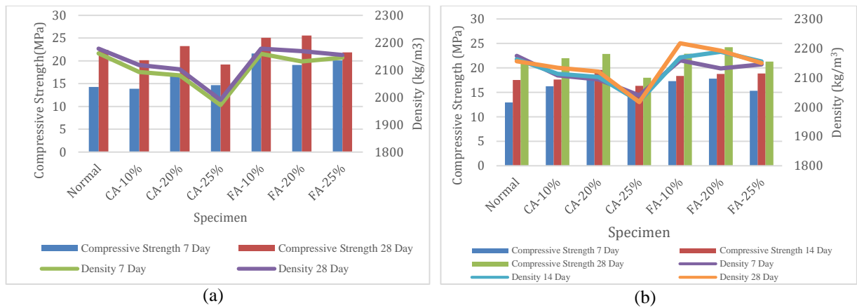
Figure 3 Compressive strength and density of using MEPS material as a substitute of fine (FA) and coarse aggregate (CA) in concrete for (a) cube and (b) cylinder specimens
