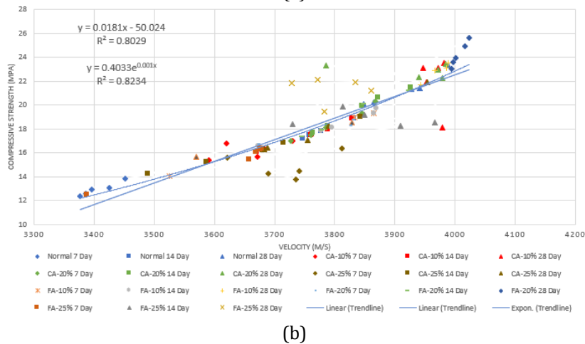
Figure 4 Compressive strength and UPV of using MEPS material as a substitute for fine (FA) and coarse (CA) aggregate in concrete for (a) cube and (b) cylinder specimens
