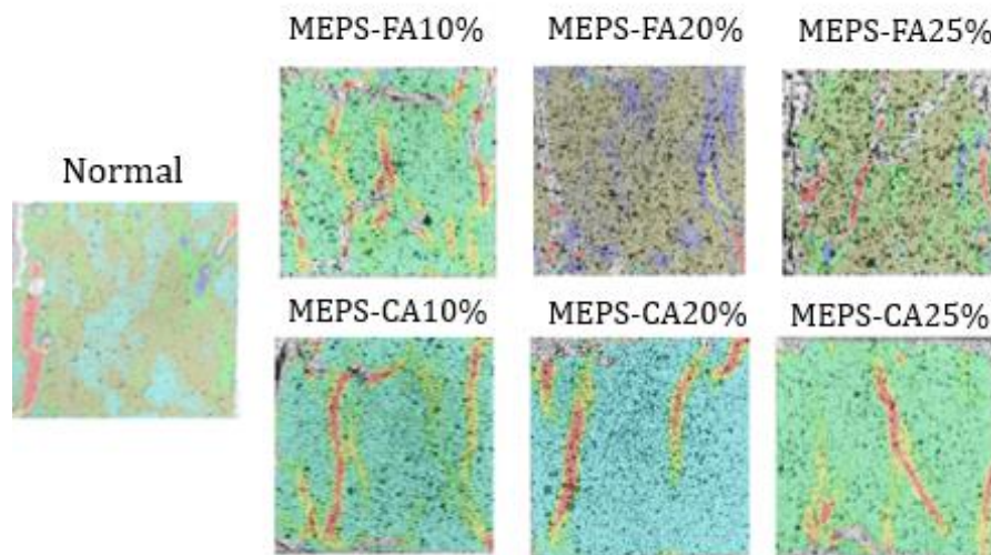
Figure 7 Failure pattern of specimens
