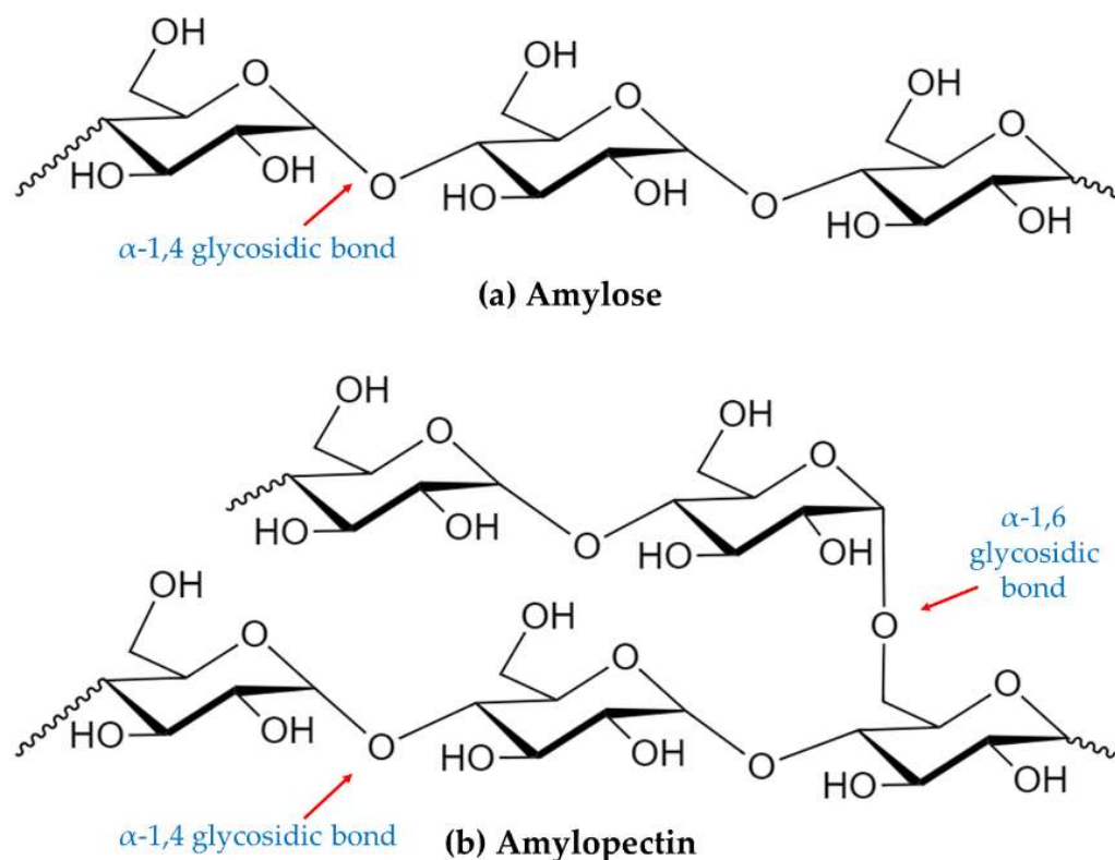
Figure 3. Structure of the amylose and amylopectin.
