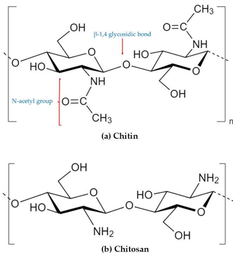
Figure 6. Chemical structure of (a) chitin and (b) chitosan.
