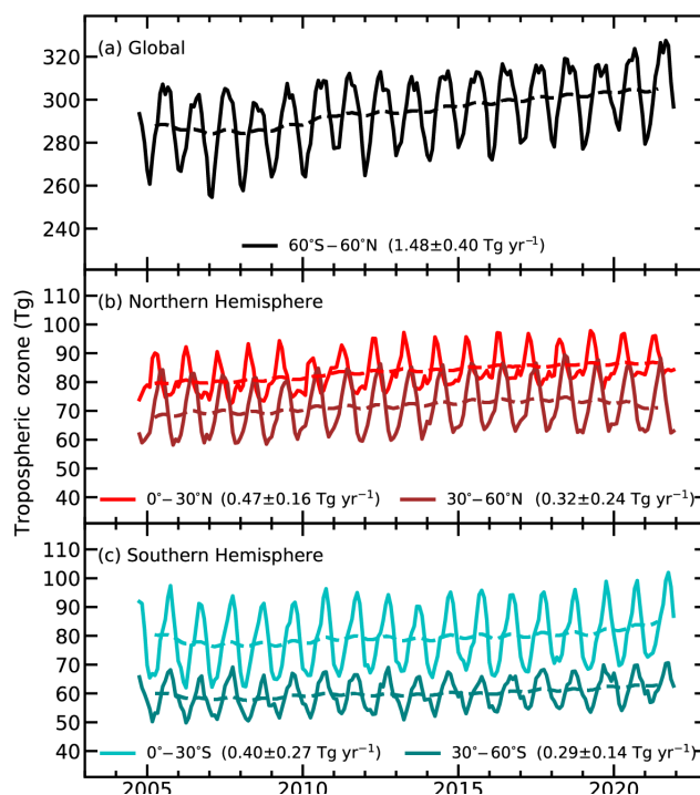
Fig. 2.62. Monthly averages (solid lines) and 12-month running means (dashed lines) of OMI/MLS tropospheric ozone burdens (Tg) from Oct 2004 through Dec 2021. (a) 60^\circ\text{S} – 60^\circ\text{N} monthly averages with 12-month running mean, (b) monthly averages and running means for the NH tropics and midlatitudes, and (c) monthly averages and running means for the SH tropics and midlatitudes. Slopes of linear fits to the data are presented with their 95% confidence-level uncertainties. Vertical resolution of OMI/MLS monthly TCO is \sim 3 km about the tropopause with \sim 2 DU (7%) precision regionally; trend uncertainties are about 0.5 DU \text{decade}^{-1} ( 1.5\% \text{decade}^{-1} ).
