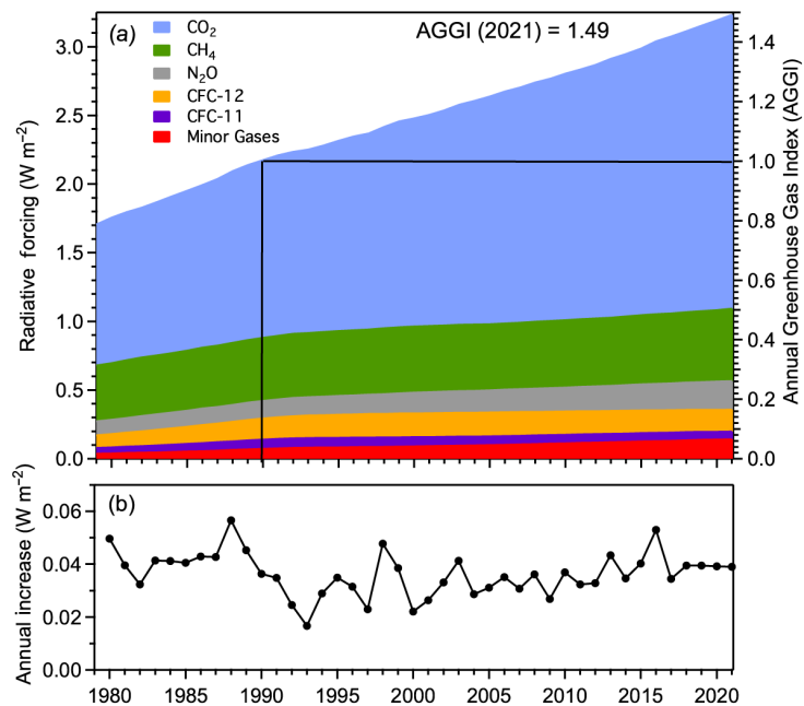
Fig. 2.51. (a) Direct radiative forcing ( W m^{-2} ) due to five major long-lived greenhouse gases (LLGHG) and 15 minor gases (left axis; see Table 2.10 for details of the 15 minor gases) and the associated values of the NOAA AGGI (right axis). The Annual Greenhouse Gas Index (AGGI) is defined to have a value of 1 in 1990. (b) Annual increase in direct radiative forcing ( W m^{-2} ).
