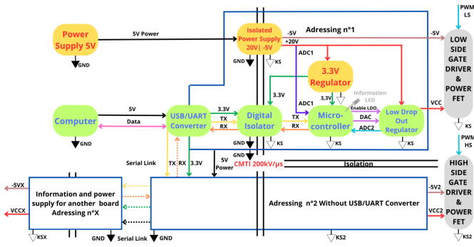
Fig. 3. Principle of isolated gate driver supply with adjustable voltages, applied identically at High Side and Low Side, with isolated digital control.
