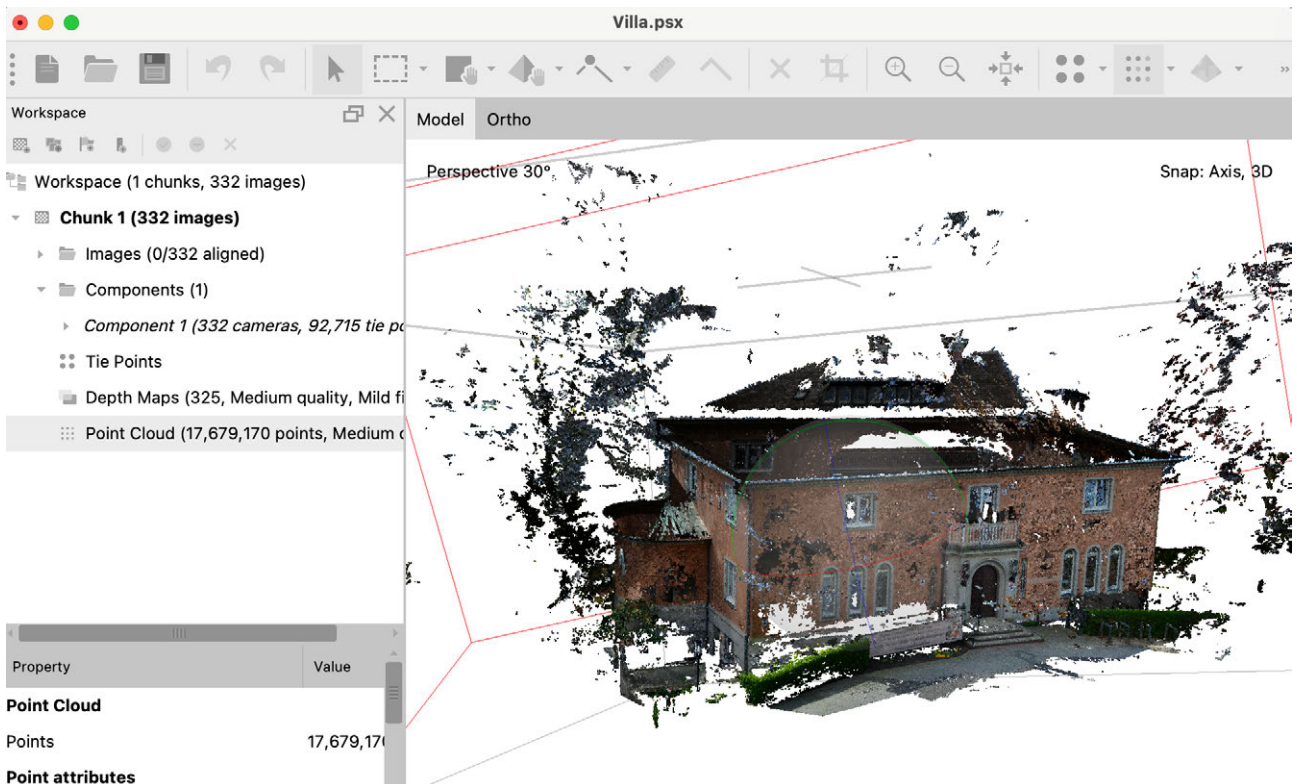
Fig. 2.3.11: Point Cloud from Agisoft Metashape
