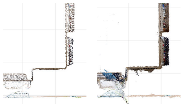
Fig. 2.2.26: Detail comparing the point densities and accuracy of the pointclouds (left .XYZ, right .E57)
