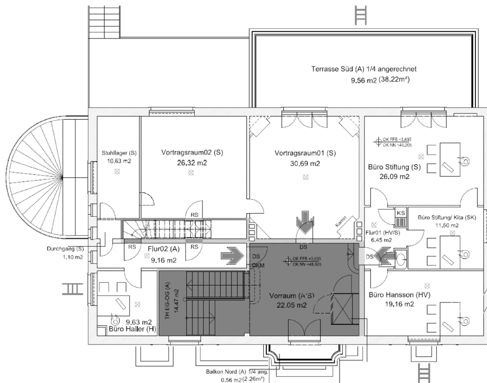
Fig. 2.3.9: Ohlendorff'sche Villa First Floor
