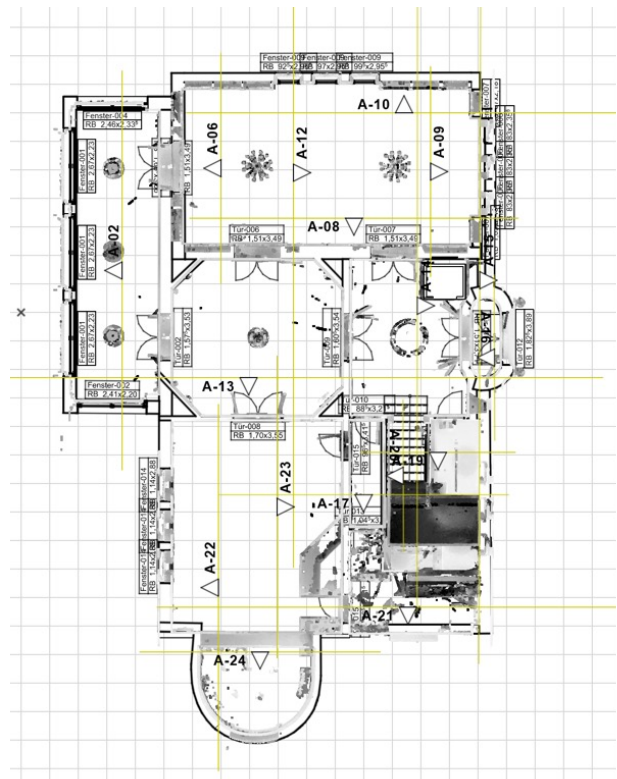
Fig. 2.1.22: Reconstructed floor plan with point cloud in the background
