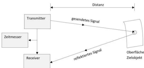
Fig. 2.6.1: Systematic of LiDAR measurement technology
