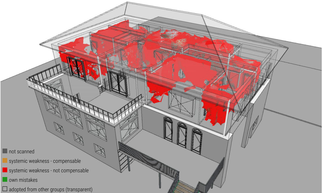
Fig. 2.4.18: 3D Meshes in CAD Model
