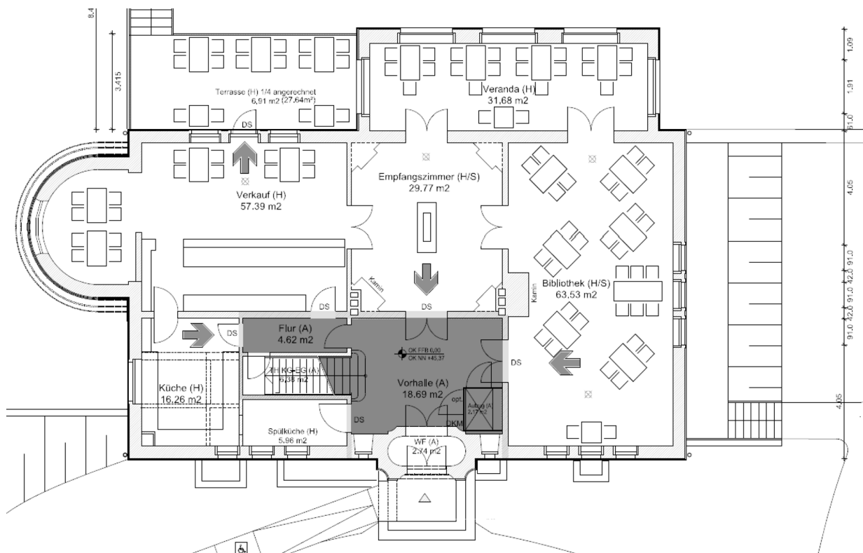
Fig. 2.3.8: Ohlendorff'sche Villa Ground Floor
