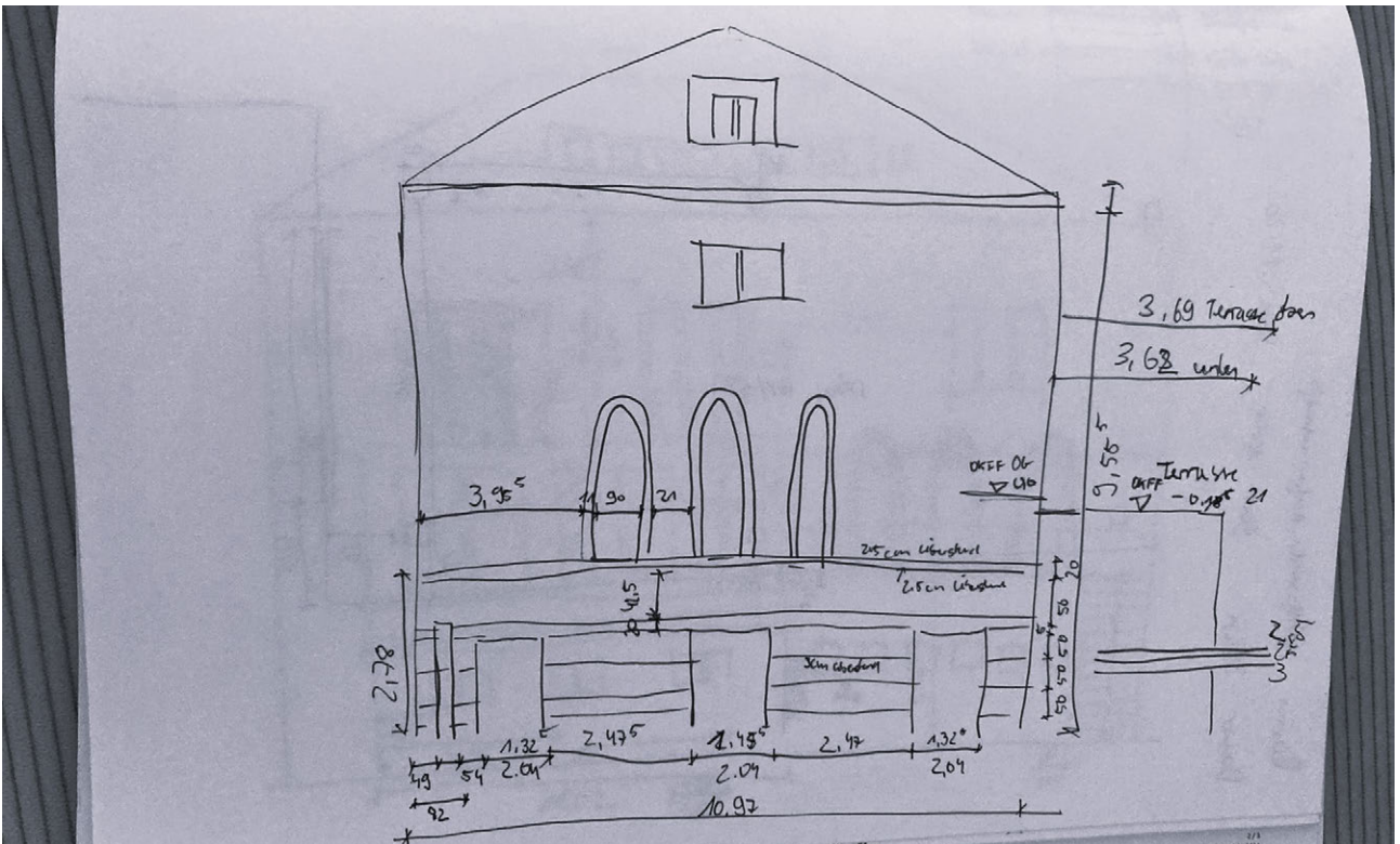
Fig. 2.7.6: Hand sketch, Westfacade
