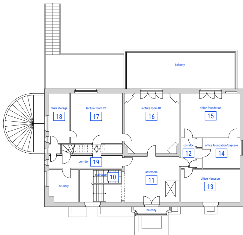
Fig. 1.3.5: Ohlendorff Villa floor plan upper floor
