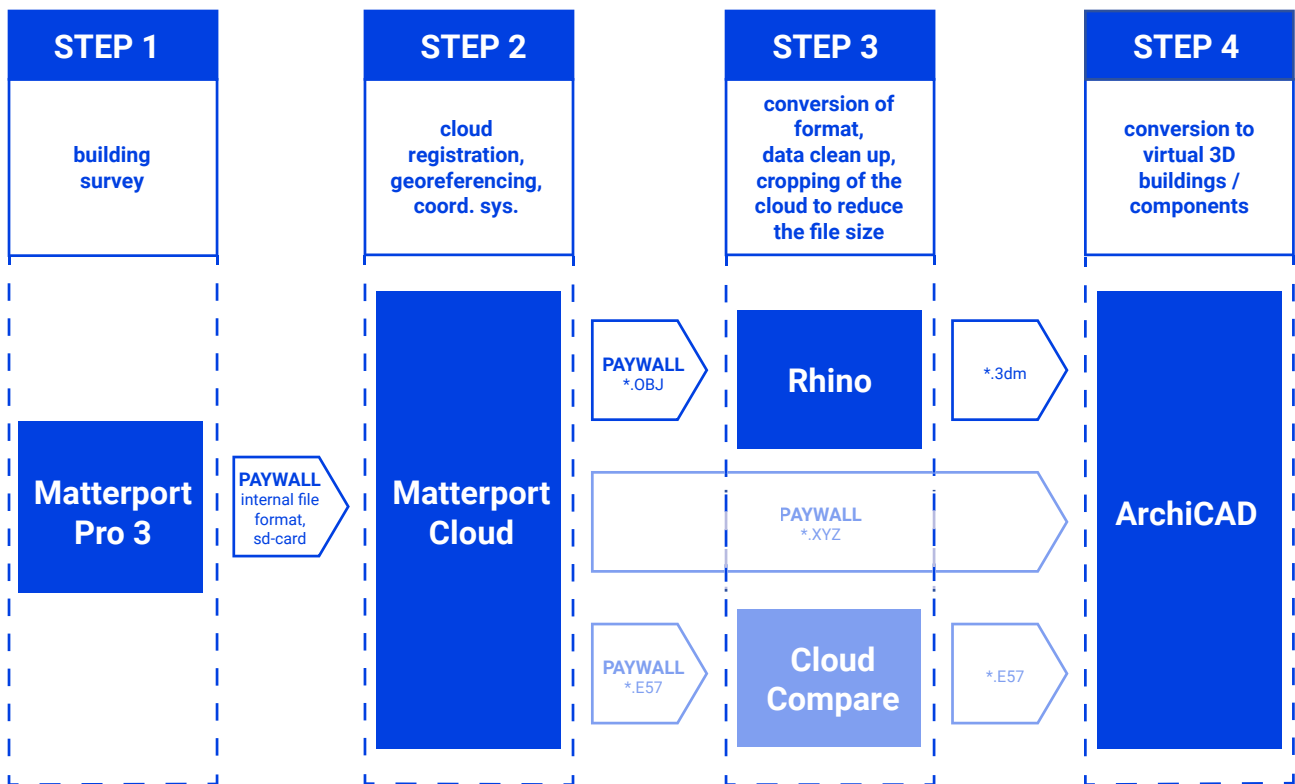
Fig. 2.2.5: Schematic diagram of procedure
