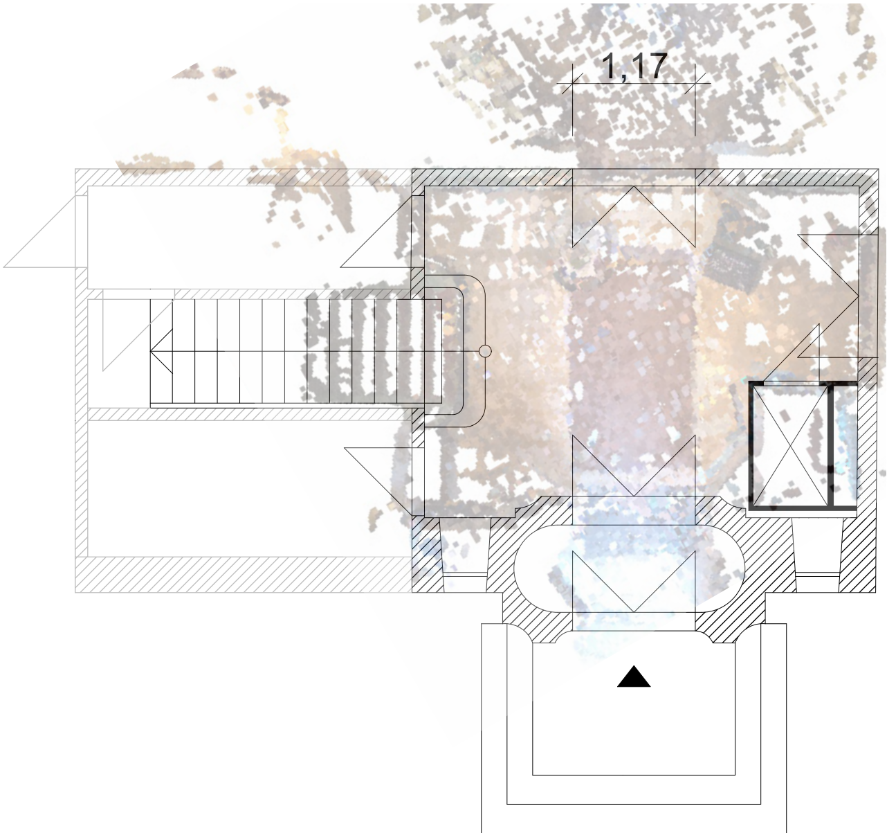
Fig. 2.5.27: Floorplan overlapping
