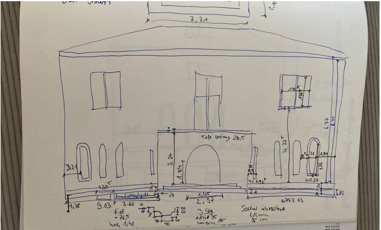
Fig. 2.7.5: Hand sketch, entrance Northfacade
