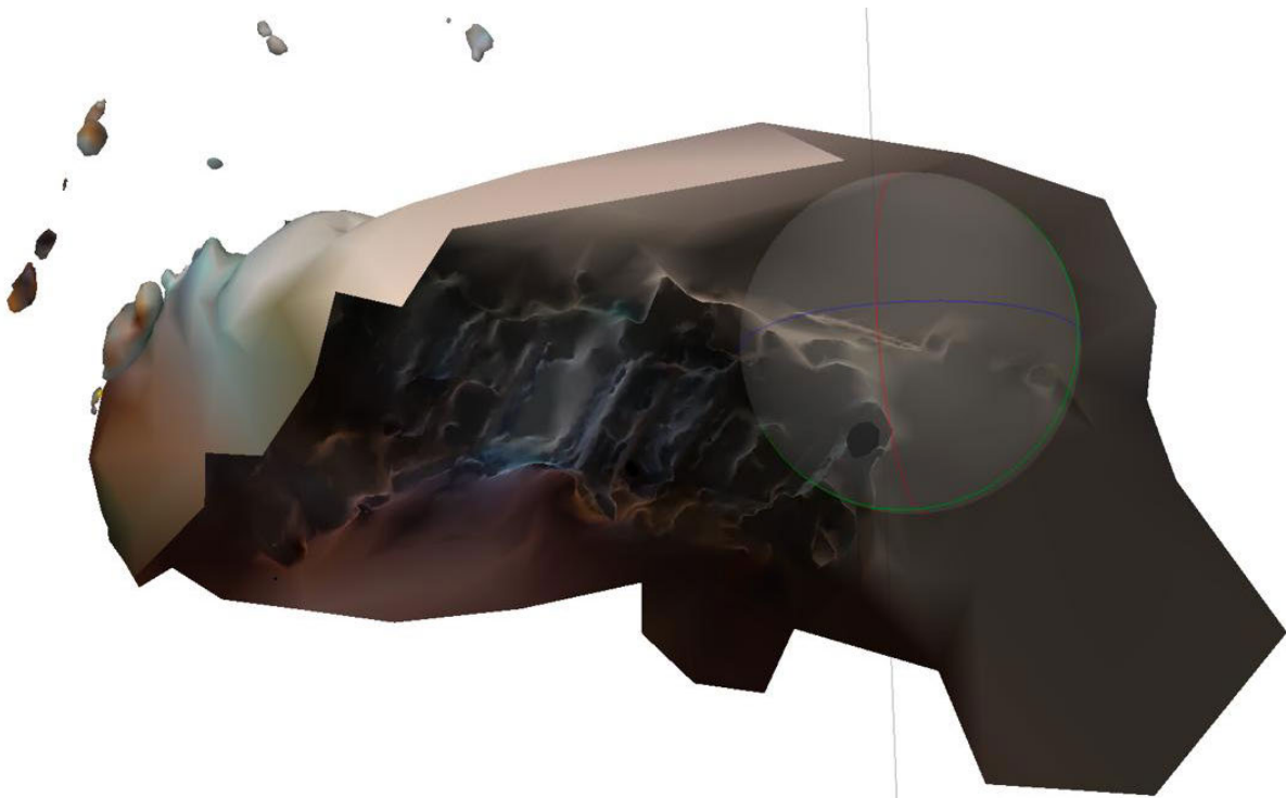
Fig. 2.5.4: Representation of the vestibule, ground floor in Metashape with 15 photos; Attempt 1
