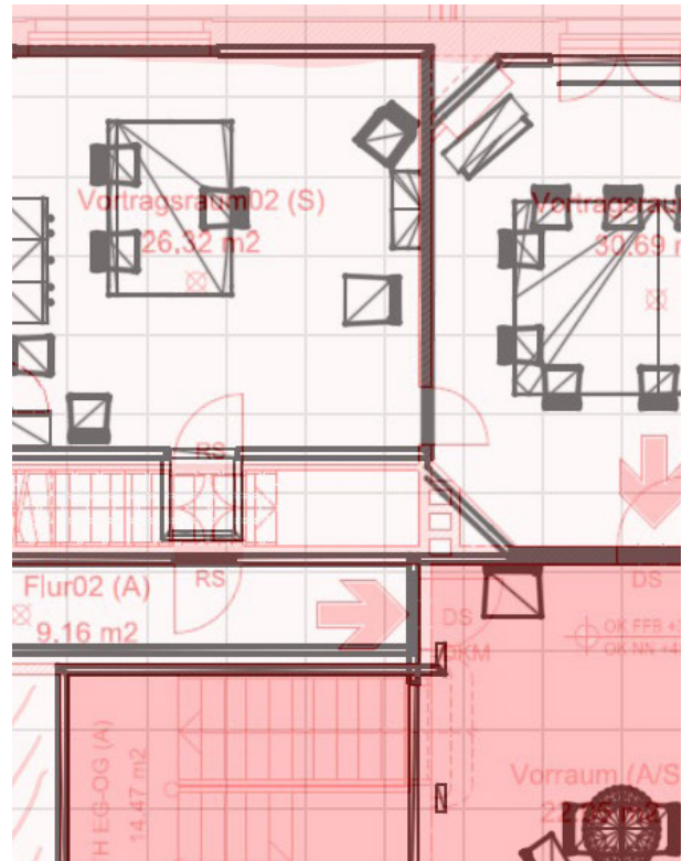
Fig. 2.6.71: Screenshot Archicad, inner corners with transparent layer
