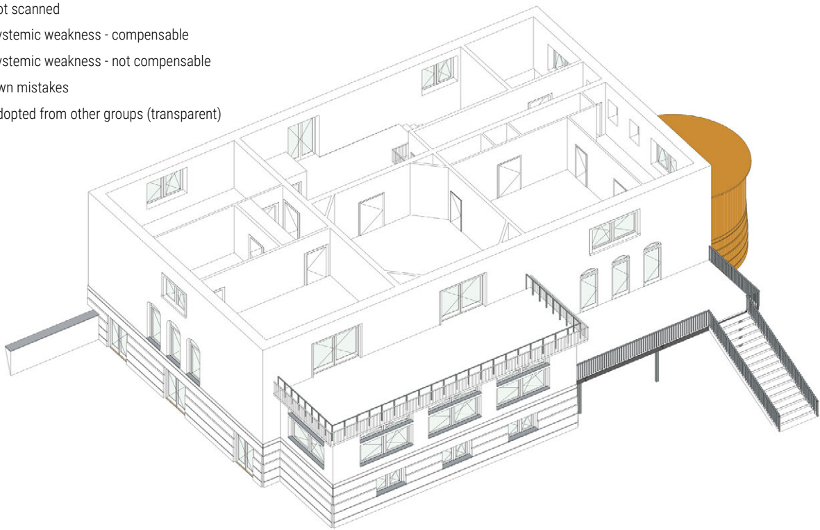
Fig. 2.7.13: 3D Modell, extruded facades and interior walls, south-west
