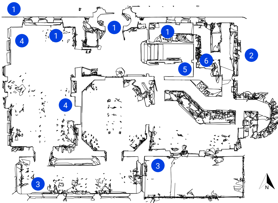
Fig. 2.2.30: Ground floor plan of the .3DM file in Archicad
