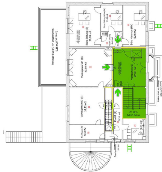
Fig. 2.2.15: Original floor plan
