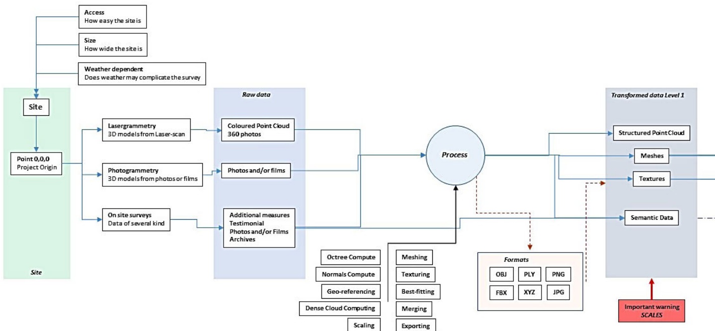
Fig. 1.1.3: Synoptic view of the data workflow
