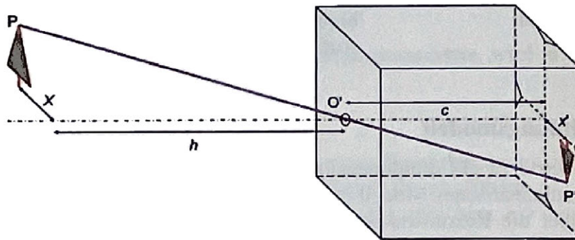
Fig. 2.4.2: Model of the pinhole camera 2
