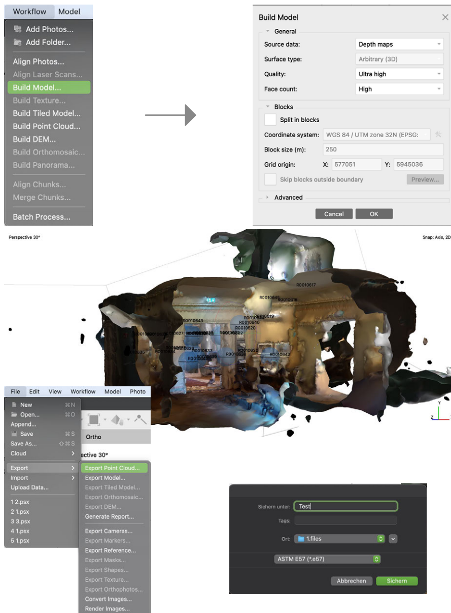
Fig. 2.5.14: Screenshots MetashapePRO
