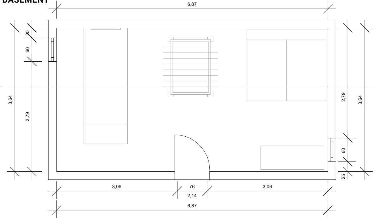
Fig. 2.4.29: CAD Plan view of the Basement
