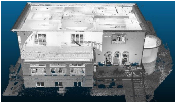
Fig. 1.2.9: Segmented point cloud from terrestrial laser scanning
