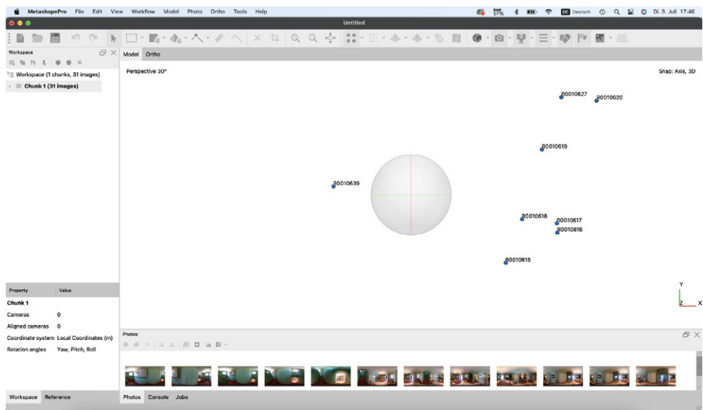
Fig. 2.5.11: Screenshots MetashapePRO
