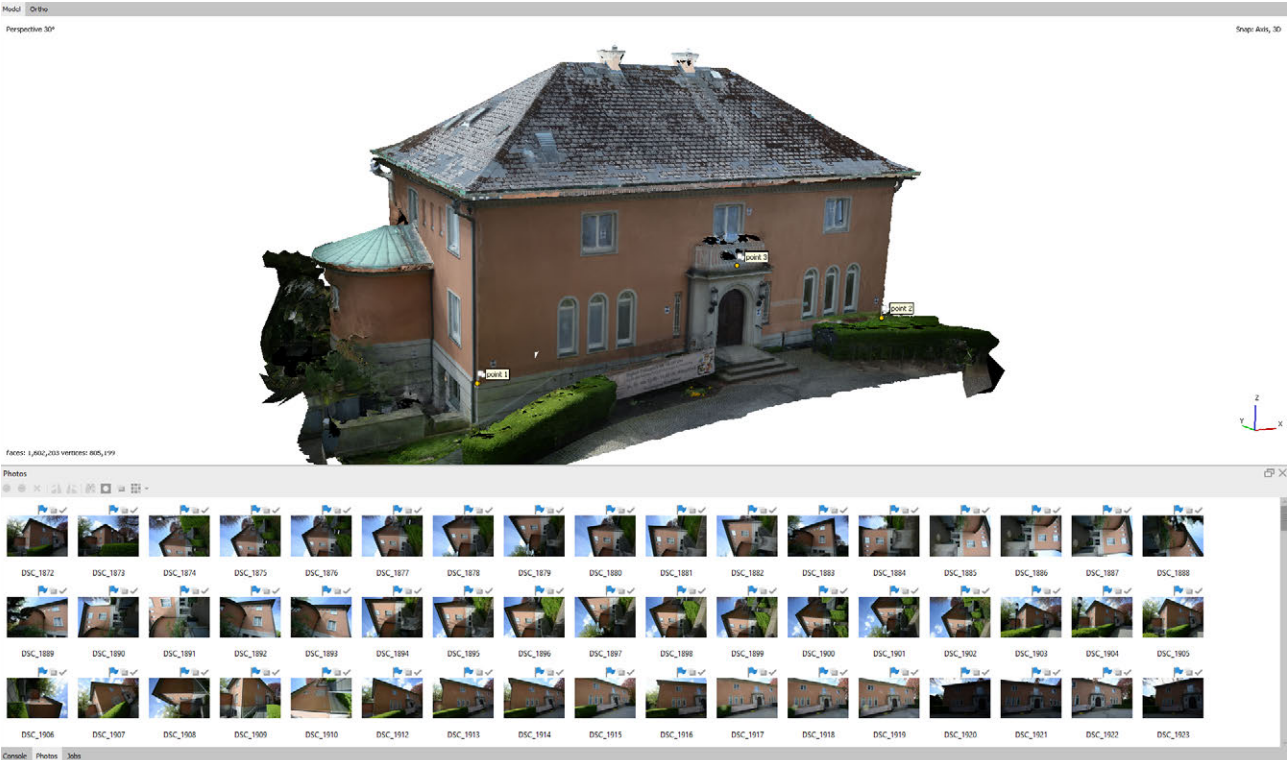
Fig. 1.1.1: Metashape interface
