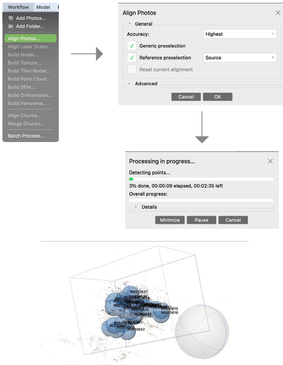
Fig. 2.5.13: Screenshots MetashapePRO
