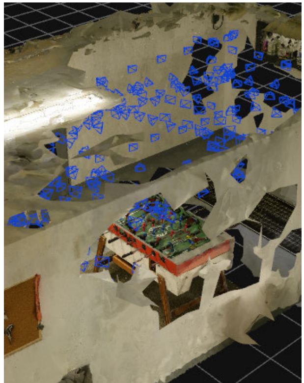
Fig. 2.4.22: Photogrammetry Results of the Basement from 3DF Zephyr
