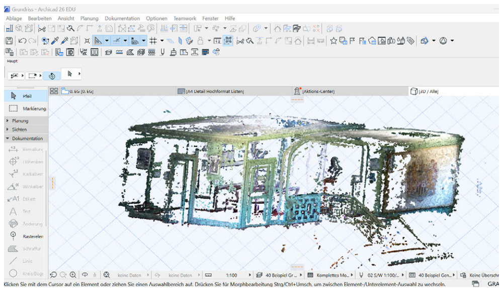
Fig. 2.5.19: Import Model to ArchiCad, 3D Mode
