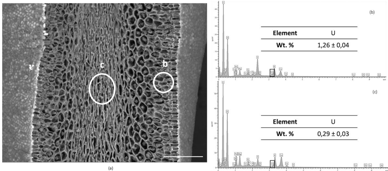
Figure 3. a) Scanning electron micrographs (SEM) of dehydrated tissues from contaminated lateral branch of A. nodosum , showing the surface and inner meristoderm structures. EDX spectra obtained from b) algal surface tissues (zone b ) and c) inner part of tissues (zone c ). Scale bar 100 μm.
