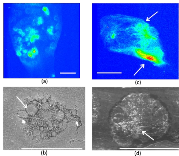
Figure 5. a) \mu -XRF cartography of uranium distribution (LII edge) inside a female receptacle of A. nodosum . Uranium hotspots are visible inside the conceptacles (red marks). b) SEM image of the female conceptacle from the receptacle of figure 6a, arrows point to the oogonium cells c) \mu -XRF cartography of uranium distribution (LII edge) inside a male receptacle of A. nodosum . d) SEM image of a male conceptacle from the receptacle of Figure 6c, arrows point to the antheridium filamentous structure cells, typical of male gametes. Scale bar: a = 1.6 cm, b and d = 500 \mu m, c = 2 cm.
