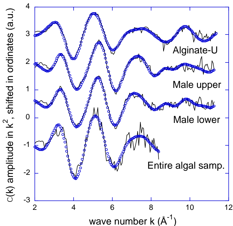
Figure. 7 : Experimental (straight line) and adjusted (dots) EXAFS spectra of Alginate-U (bulk EXAFS), A. nodosum male receptacle upper part (imaging EXAFS), A. nodosum male receptacle lower part (imaging EXAFS) and A. nodosum entire algal sample (bulk EXAFS).
