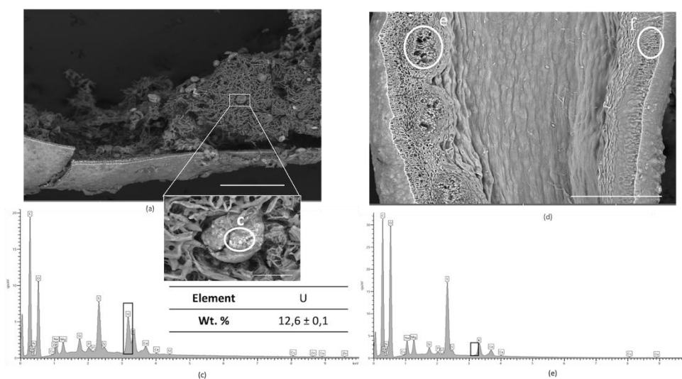
Figure 4. SEM images of contaminated receptacles from 2 different individuals of A. nodosum exposed for 5 days at 10^{-4} M of uranyl nitrate and the EDX spectra. a) Micrograph of a female receptacle, blown up after dehydration, showing the exposed oogonium b) Zoom on the oogonium structure, filled with eggs contaminated with ^{235}\text{U} , stored under the cell membrane (translucent white spots). c) EDX spectrum obtained in the middle of one egg highlighting the presence of accumulated uranium (zone c). d) Cross section SEM image of male receptacle showing the antherridium filament structure. e) EDX spectrum recorded inside the male receptacle, zone e, showing no visible U. Scale bar: a = 500 \mu\text{m} , b = 50 \mu\text{m} and d = 500 \mu\text{m} .
