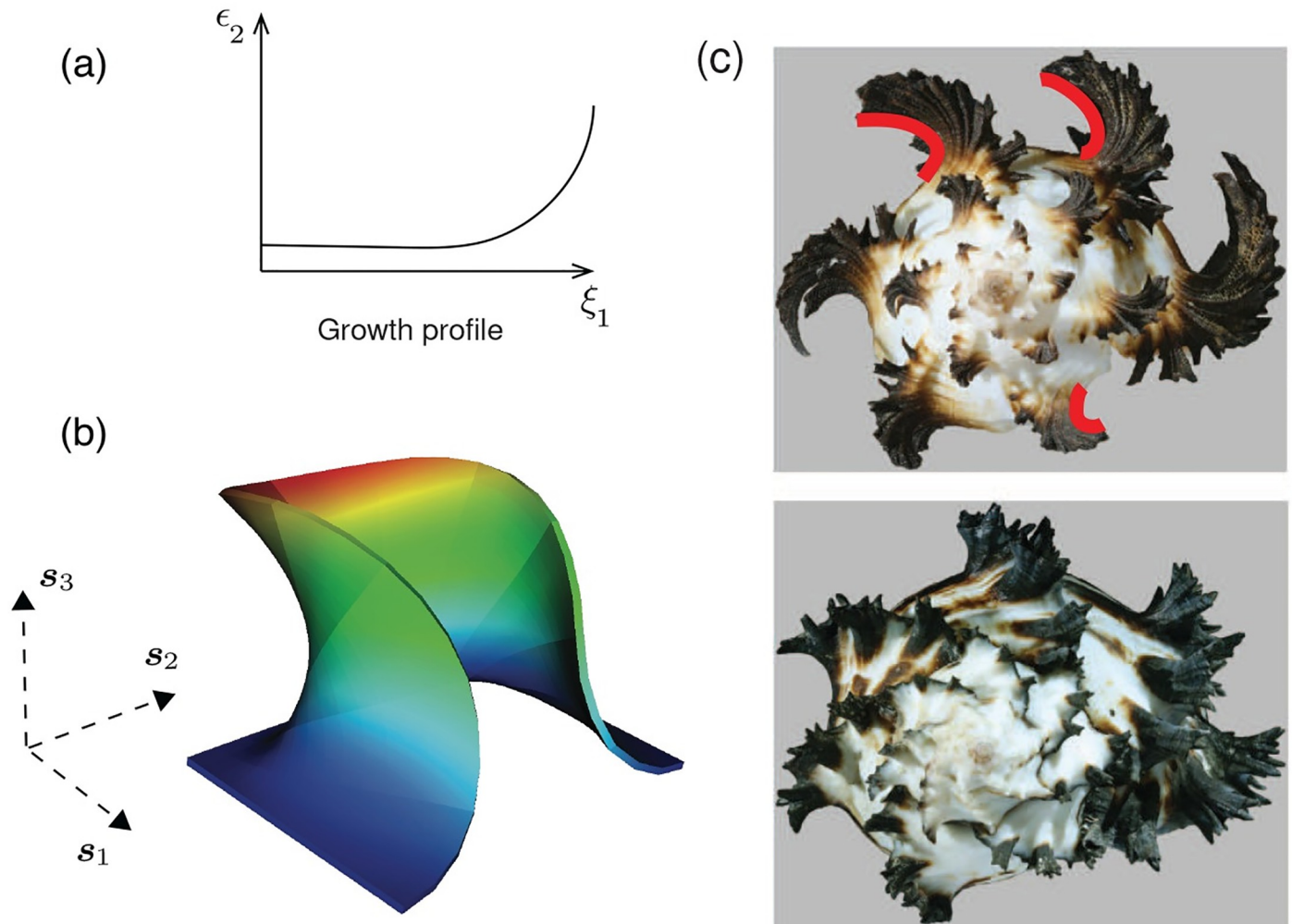
Fig 14. Spatially varying volume growth. We impose volume growth strain increments that vary along the \xi_1 direction that is the curvilinear coordinate defining s_1 , with an increasing gradient toward the leading edge, as shown in (a). The result appears in (b), displaying large, negative Gaussian curvature, mimicking the strongly backward arching morphology observed in a number of shell species, for example as seen also in (c) Hexaplex chicoreum . Dirichlet boundary conditions, u = 0 , are applied on the trailing surface (boundary) and the lateral surfaces (boundaries) of the mantle, which are perpendicular to s_1 , and traction-free Neumann conditions, PN = 0 , are applied on the front surface (boundary). Also see S6 Movie for the evolution of deformation leading to a morphology with strongly negative Gaussian curvature.
