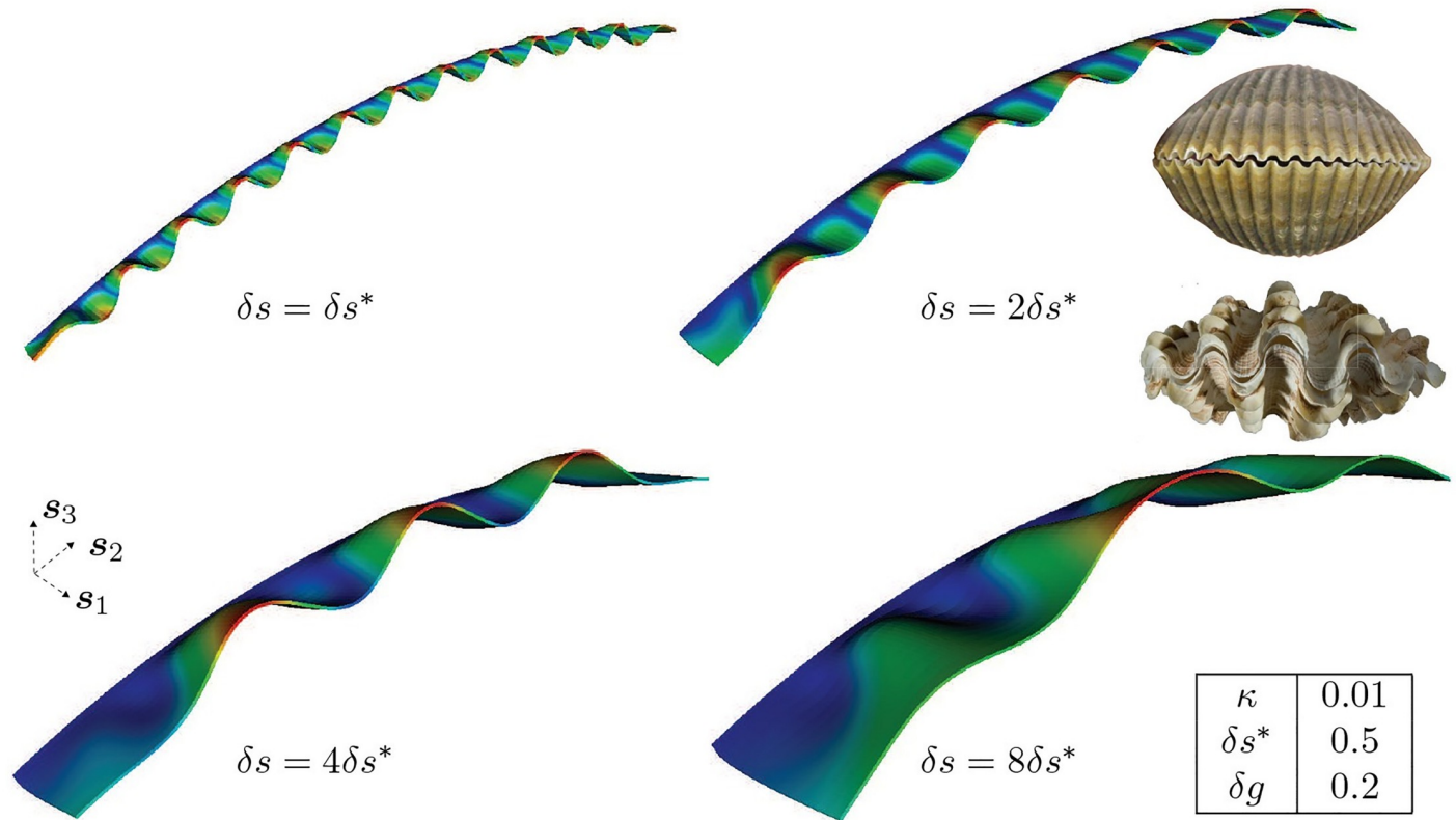
Fig 7. Effect of incremental active mantle widths on mantle deformation for fixed \delta g and \kappa . Increasing the active mantle width \delta s = |v_1 s_1 - v^v| \Delta t over \Gamma_0 leads to morphologies bearing a similarity with the ornamentalations on Clinocardium nuttallii (upper inset) and Tridacna squamosa (lower inset). Dirichlet boundary conditions, \mathbf{u} = \mathbf{0} , are applied on the trailing surface (boundary) and traction-free Neumann conditions, \mathbf{PN} = \mathbf{0} , are applied on the remaining surfaces (boundaries). See Fig 4 for location of the trailing surface, front surface and the lateral surfaces. Also see S3 Movie for a morphology that is similar to the case \delta s = \delta s^* , and bears comparison to the ornamentation on members of the class Bivalvia .
