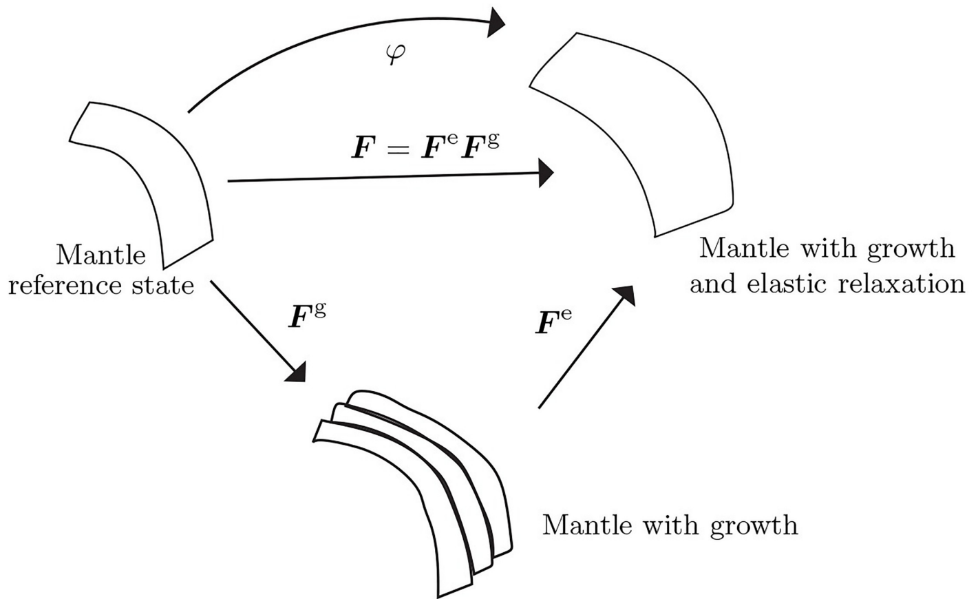
Fig 3. The kinematics of growth. The observed deformation gradient, F , is composed of an incompatible growth component, F^g , and another incompatible, but elastic component, F^e , which restores compatibility of F .
