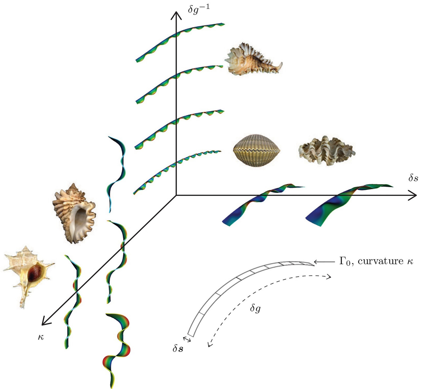
Fig 15. Phase diagram representing the effect of the growth and geometric parameters—growth strain increment ( \delta_g ), active mantle width ( \delta_s ), and curvature of the reference curve ( \kappa ), on the morphology of shell ornamentations.
