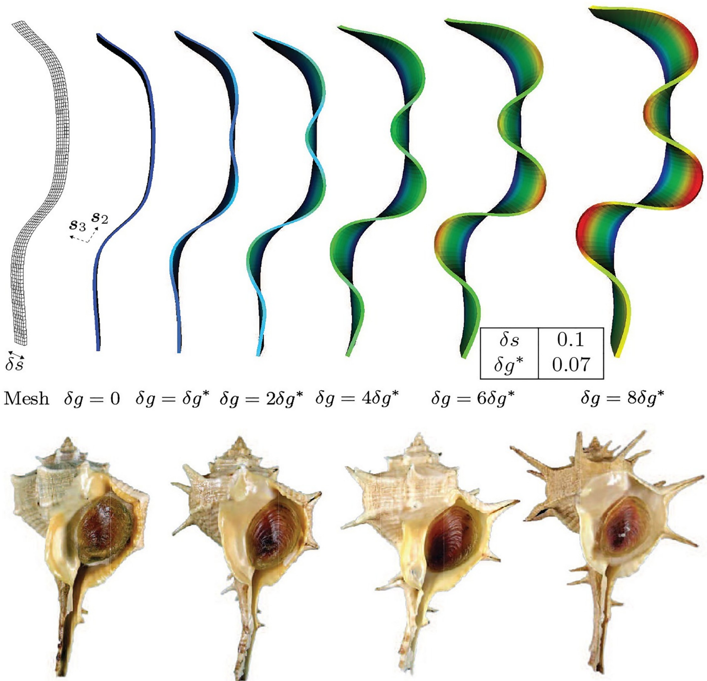
Fig 11. Progression of curvature-compatible ornamentation with volume growth strain increments, \delta g . The deformed mantles show marginally preferred localization around points of high curvature and thereafter the amplitude increases with volume growth strain increments. Some of these shapes with different amplitudes can be observed in the shells of the species Bolinus brandaris (bottom row of inset images). Dirichlet boundary conditions, \mathbf{u} = \mathbf{0} , are applied on the trailing surface (boundary) and traction-free Neumann conditions, \mathbf{PN} = \mathbf{0} , are applied on the remaining surfaces (boundaries).
