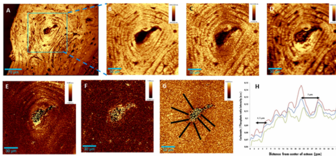
Fig. 11. A) optical image x20; B) 960 \text{cm}^{-1} ; C) 1660 \text{cm}^{-1} ; D) 2950 \text{cm}^{-1} ; E) Ratio phosphate 960/amide I 1660; F) Ratio phosphate 430/amide III 1246; G) Ratio carbonate/ \nu_1 phosphate; H) plotted profile of black line shown in G (blue line: mean curve; red and green line: standard deviation curves).
