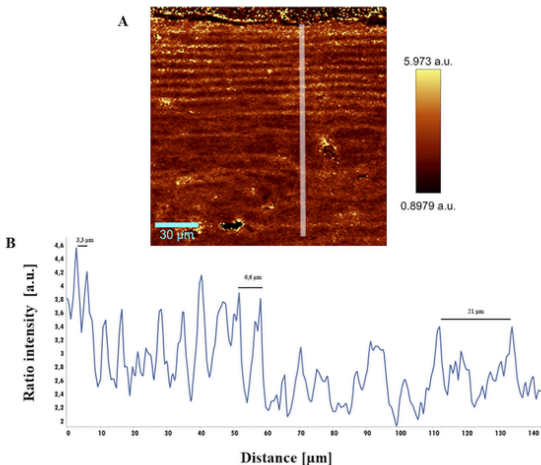
Fig. 9. 960/1660\text{ cm}^{-1} Raman intensity peak ratio. A) cartography of ratio with connected lookup table. B) plotted profile corresponding to the line shown in A.
