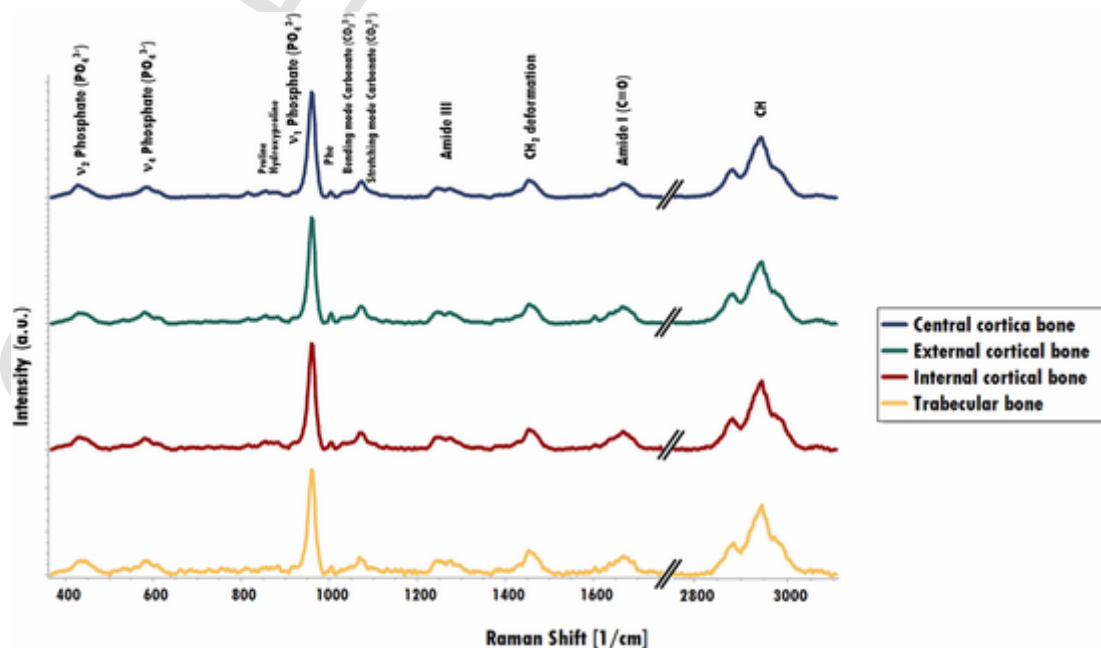
Fig. 6. Characteristic Raman spectra for the 4 scanned areas: external, central, internal cortical bone, and trabecular bone.
