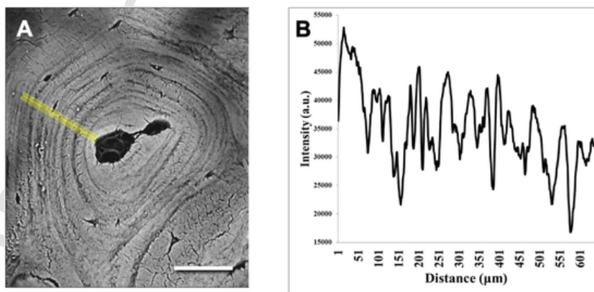
Fig. 10. Scanning electron microscopy image of the lamellar bone around an osteon. In panel B, a plotted of intensity is represented to illustrate formation of bone in concentric circles, and measurement of spatial frequencies could be evaluated. Scale bar: 50\text{ }\mu\text{m} .
