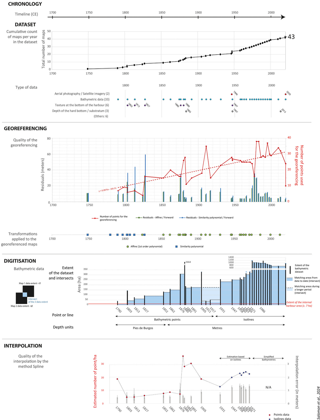
Fig. 2. Dataset of old maps and their characteristics, including a quality assessment of the georeferencing of the maps, the digitising, and the interpolation of the bathymetric data. All data are plotted referring to the date of the map.
