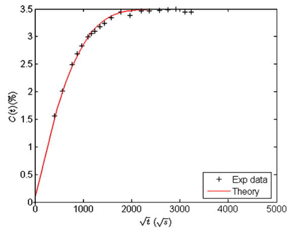
Figure 7: Experimental and simulated moisture content in composite vs. root of time
