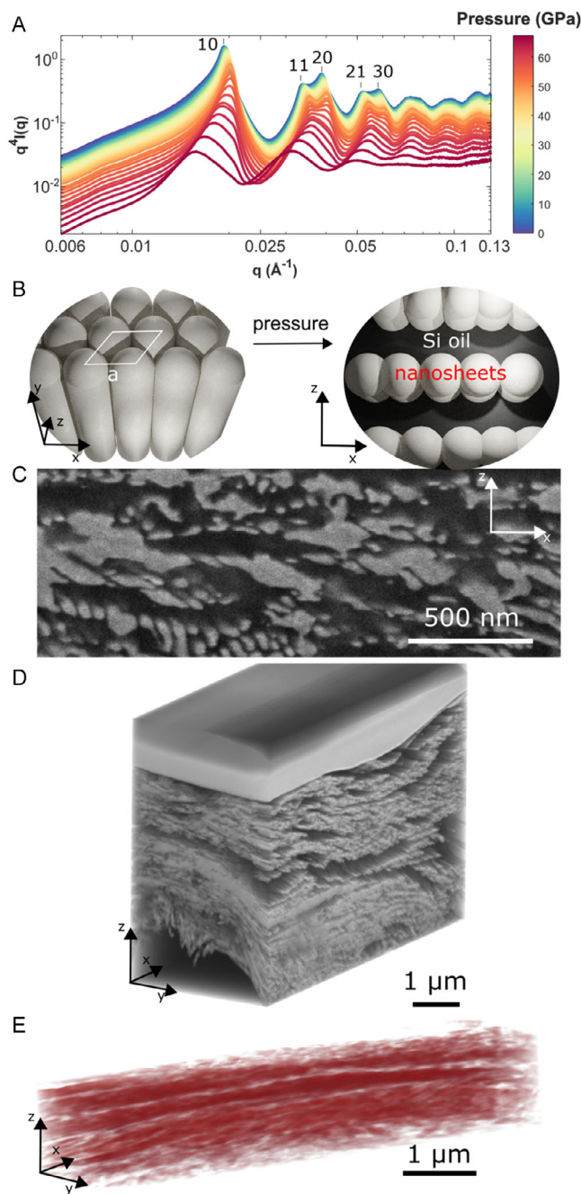
Figure 5. In situ and ex situ characterization of the deformation of Au@AgNR 217 × 31 supercrystals. A) HP-SAXS-integrated diffractogram collected at varied pressures during compression for Au@AgNR 217 × 31 supercrystal. The vertical lines indicate the expected positions of some Bragg peaks of a hexagonal 2D lattice. B) Scheme of the unit cell and proposed deformation pathway for the lattice. C–E) Corresponding FIB–SEM tomography images after releasing the pressure. (C) SEM micrograph showing the cross section of the supercrystal. (D,E) 3D reconstructions of a portion of the supercrystal. NPs in (C,D) appear in light contrast, while voids are depicted in dark contrast. In (E), NPs are color coded in red.
