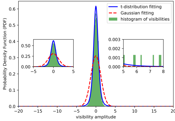
Fig. 3: Comparison of t -distribution fitting and Gaussian distribution fitting.
