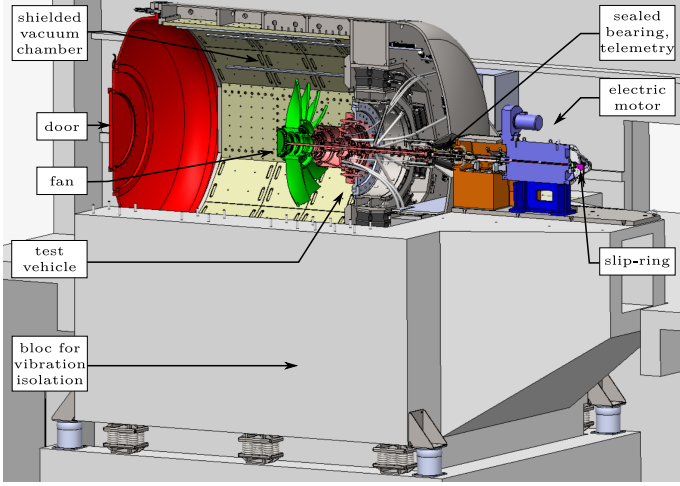
Fig. 6: Cross-sectional view of test rig PHARE#1.
