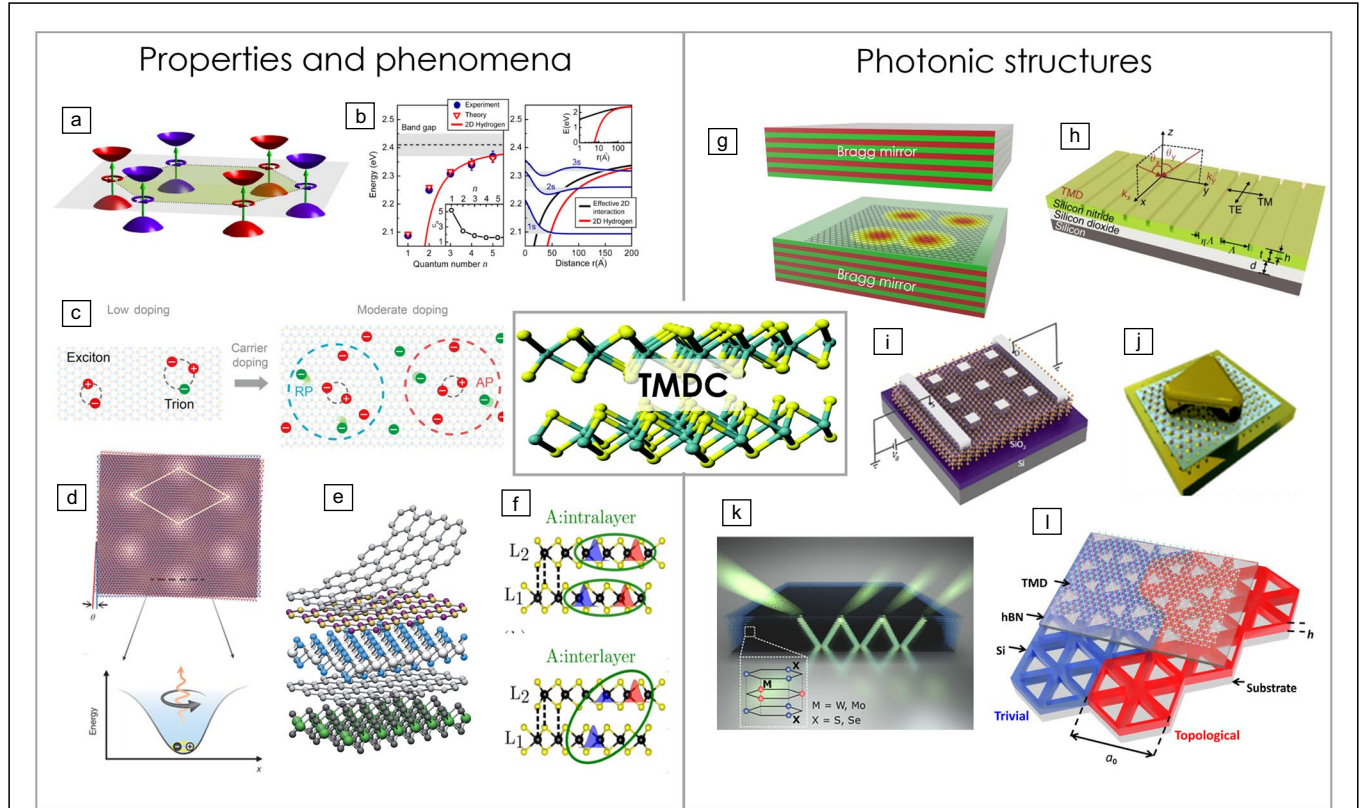
Figure 3. Properties and unique phenomena of TMDCs for exciton-polariton studies (Left panel) as well as the photonic structures that enable the realization of polaritons (Right panel). (a) Valley polarization property. Reprinted with permission from Reference 108. © 2014 Springer Nature. (b) Rydberg excitons observable due to the large binding energy. Reprinted with permission from Reference 109. © 2014 American Physical Society. (c) Charged excitons-trions and Fermi-polarons. Reprinted from Reference 110. CCBY 4.0. (d) Moiré excitons. Reprinted with permission from Reference 111. © 2019 Springer Nature. (e) Van der Waals heterostructures. Reprinted with permission from Reference 112. © 2013 Springer Nature. (f) Dipolar interlayer excitations. Reprinted with permission from Reference 113. © 2021 Springer Nature. (g) Bragg reflector-based 1D cavity. Reprinted with permission from Reference 96. © 2014, Springer Nature Limited. (h) Photonic crystal. Reprinted from Reference 99. CCBY 4.0. (i) Plasmonic array. Reprinted with permission from Reference 114. © 2020 American Chemical Society. (j) Nanoparticle on mirror. Reprinted with permission from Reference 115. © 2020 American Physical Society. (k) Self-hybridized polaritons. Reprinted with permission from Reference 102. © 2019 American Chemical Society. (l) Topological photonic crystals. Reprinted from Reference 116. CCBY 4.0.
