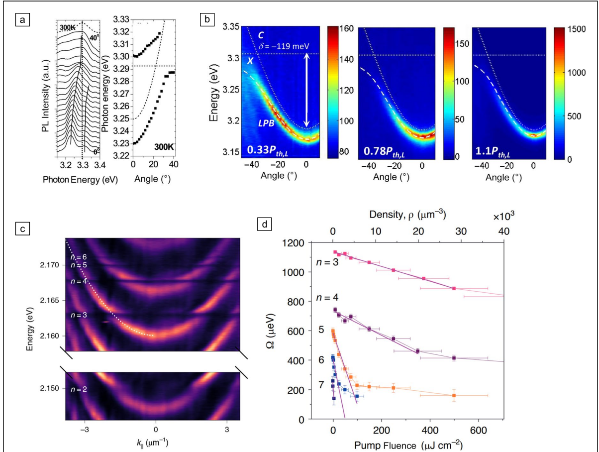
Figure 2. (a) Angle-resolved room-temperature spectra for a hybrid ZnO \lambda -thick microcavity. Reprinted with permission from Reference 70. © 2008 AIP Publishing. (b) Polariton lasing in an optically pumped 3\lambda/2 -thick hybrid ZnO microcavity at room temperature. Reprinted with permission from Reference 71. © 2012 Optical Society of America. (c) Rydberg polaritons up to n = 6 in a \sim 30 \mu\text{m} thick Cu 2 O microcavity. Reprinted with permission from Reference 72. © 2022 The Author(s), under exclusive license to Springer Nature Limited. (d) Quenching of Rabi splitting for Rydberg polaritons in a Cu 2 O microcavity under resonant pulsed excitation. Reprinted from Reference 11. CCBY 4.0.
