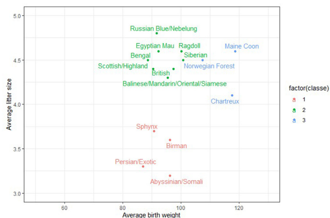
Fig. 4. Representation of the three clusters of feline breeds identified by K-means algorithm depending on their average birth weight and their average litter size. Cluster 1 (in red): small litter sizes and average birth weights (n = 4 breeds), Cluster 2 (in green): average litter sizes and average birth weights (n = 8 breeds), Cluster 3 (in blue): average litter sizes and high birth weights (n = 3 breeds).
