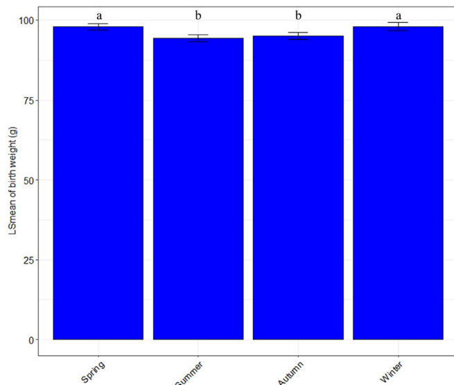
Fig. 3. Least square mean of birth weight according to season of birth. Any two seasons receiving the same letter at the top of the bar were not significantly different, as per Tukey's HSD method. The error bars represent the standard error of the least square mean values.
