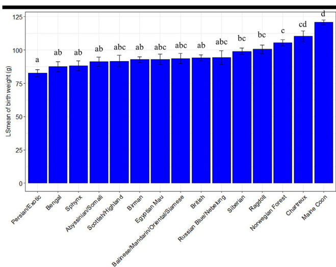
Fig. 2. Least square mean of birth weight for the 15 breeds represented. Any two breeds receiving the same letter at the top of the bar were not significantly different as per Tukey's HSD method. The error bars represent the standard error of the least square mean values. Number of kittens included for each breed is detailed in Table 1.
