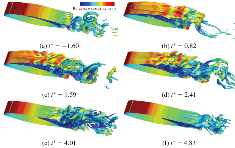
Fig. 9 Instantaneous vorticity magnitude isosurfaces for |\vec{\omega}|c/U = 10
