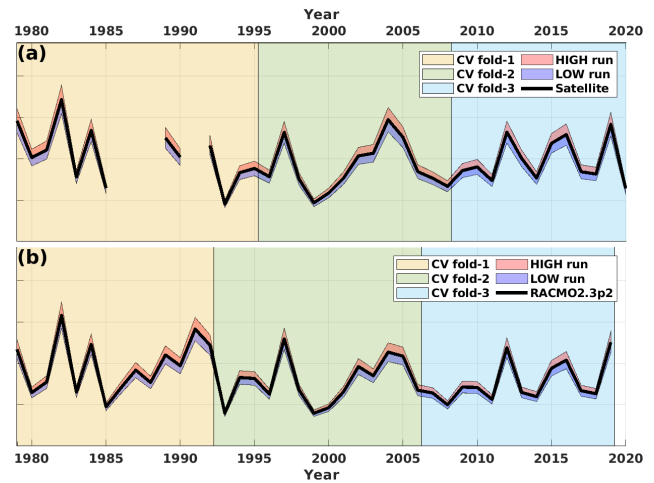
Figure 2. Schematic overview of the time periods for each CV folders and the HIGH/LOW sensitivity experiments. Panel (a) is for satellite estimates and PDD melt day calculations. Panel (b) is for RACMO2.3p2 simulations and PDD melt amount calculations.
