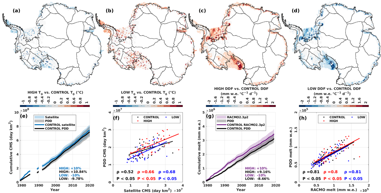
Figure 8. Panels (a) and (b): difference between T_0 parameterized in the HIGH/LOW experiment and the CONTROL (optimal) T_0 . Panels (c) and (d): spatial maps for the difference between the DDF parameterized in the HIGH/LOW experiment and the CONTROL (optimal) DDF. Panels (e) and (g): CMS/annual melt amount for the satellite estimates/RACMO2.3p2 simulations and dist-PDD outputs. Note that the period for (e) is from 1979/1980 to 2020/2021 (with 1986/1987 to 1988/1989 and 1991/1992 omitted). The period for (g) is from 1979/1980 to 2019/2020. The upper and lower boundaries of the semi-transparent shaded areas indicate the HIGH/LOW satellite estimates and the HIGH/LOW dist-PDD outputs. The percentage difference annotated in the bottom-left corner is calculated between the HIGH/LOW and the CONTROL for each variable (by “variable”, we mean satellite melt occurrence data/dist-PDD melt occurrence and amount data/RACMO2.3p2 melt amount data) respectively. Panels (f) and (h): scatter plots and the Spearman’s \rho (with its statistical significance) for dist-PDD outputs and satellite/RACMO2.3p2, from each sensitivity experiment (HIGH, LOW and CONTROL). This analysis is based on dist-PDD.
