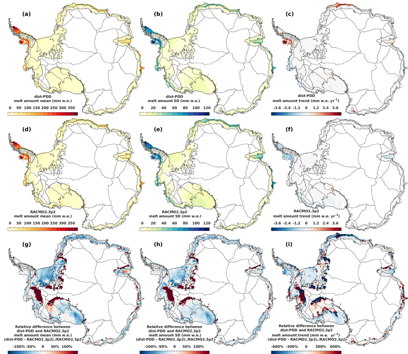
Figure D4. Panels (a) to (f): mean, SD and trend of dist-PDD/RACMO2.3p2 melt amounts for the period 1979/1980 to 2019/2020 respectively. Panels (g) to (i): relative difference between dist-PDD and RACMO2.3p2 melt amount mean, SD and trend for the period 1979/1980 to 2019/2020 respectively.
