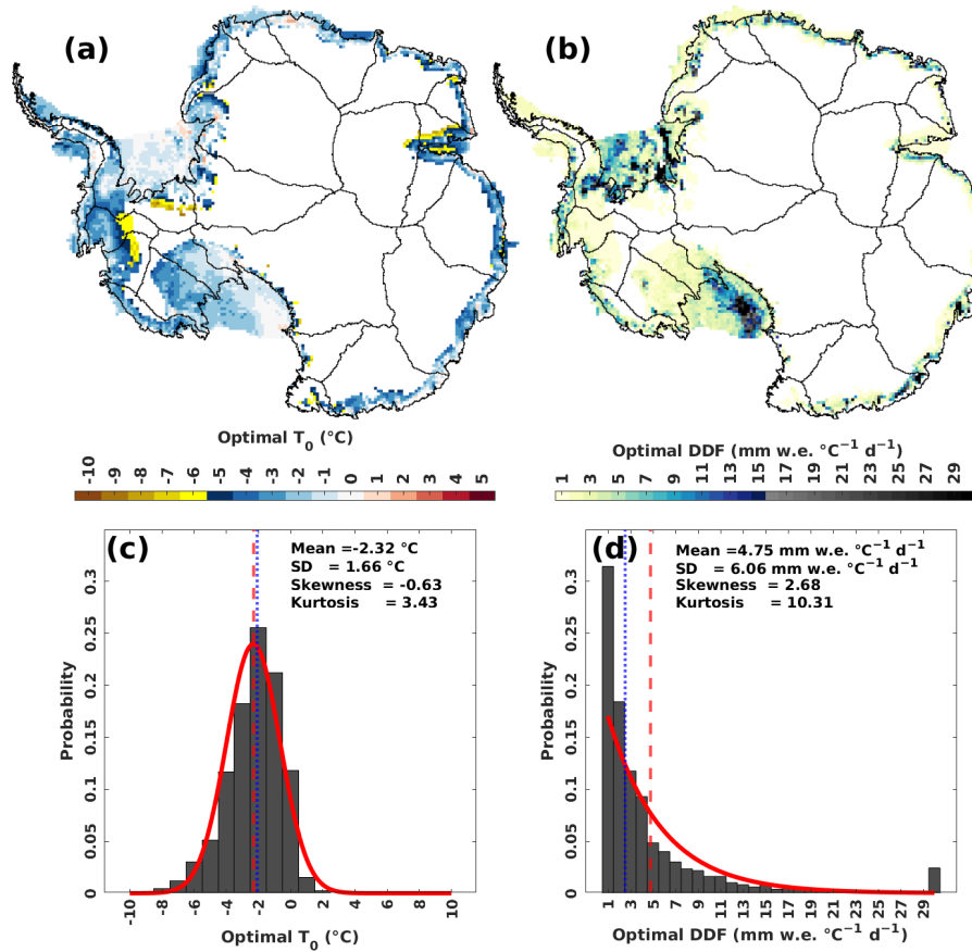
Figure 3. (a) The optimal T_0 (°C) of each computing cell. (b) The optimal DDF (mm w.e. °C -1 d -1 ) for each computing cell. (c) Probability histogram of the optimal T_0 (°C). Red curve is the fitted normal distribution. Vertical dashed red line is the mean of T_0 for all computing cells. Dotted blue line is the median of T_0 for all computing cells. (d) Probability histogram for the optimal DDF (mm w.e. °C -1 d -1 ). Red curve is the fitted exponential distribution. Vertical dashed red line is the mean of DDF for all computing cells. Dotted blue line is the median of DDF for all computing cells.
