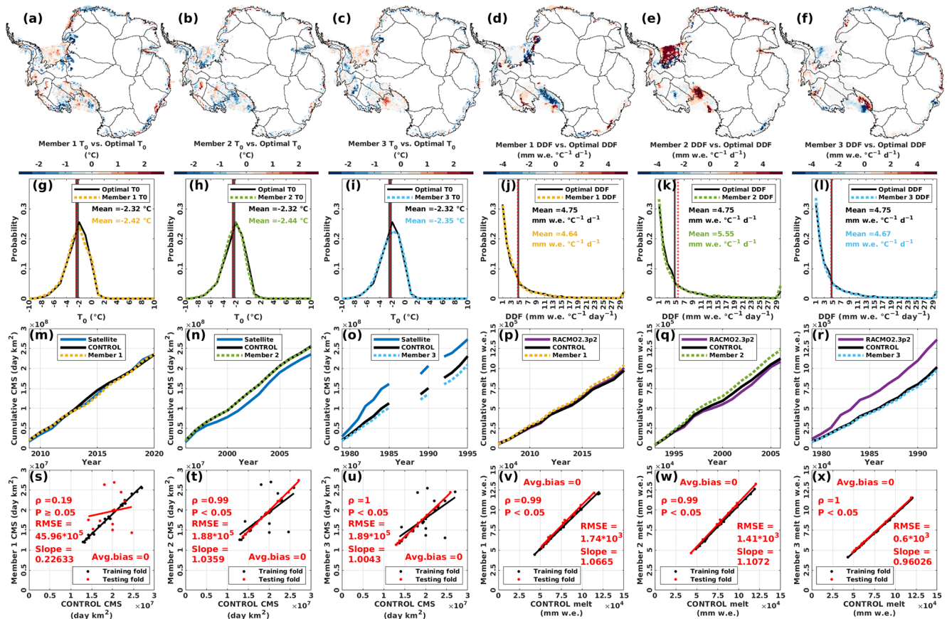
Figure 7. Panels (a) to (f): differences between the T_0 /DDF parameterized in each member of the T_0 /DDF 3-fold CV and the optimal T_0 /DDF respectively. Panels (g) to (l): probability distributions for the T_0 /DDF of each T_0 /DDF 3-fold CV and the optimal T_0 /DDF respectively. Vertical black lines indicate the mean of optimal T_0 s/DDFs. Vertical dotted red lines indicate the mean of T_0 /DDF for each member respectively. Panels (m) to (r): CMS/annual melt amount for satellite estimates/RACMO2.3p2 simulations, CONTROL (which is the PDD model run with optimal T_0 and DDF) and each member for the period of the testing fold respectively. We calculate the difference in CMS/annual melt amount between each member and the CONTROL, at the end of the testing fold respectively. Panels (s) to (x): scatter plots for the CMS/annual melt amount of each 3-fold CV member against the CONTROL respectively. The Spearman’s \rho and its statistical significance, as well as the slope, RMSE and average bias for the OLS fit, for the testing fold between each member and the CONTROL are calculated respectively. This analysis is based on dist-PDD.
