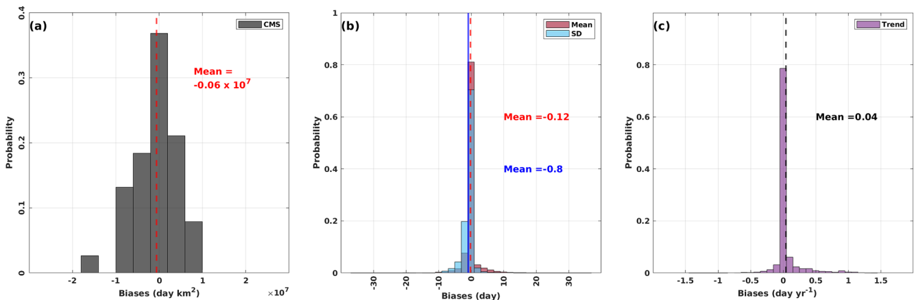
Figure D1. Panel (a): probability histogram for the biases between the dist-PDD and satellite CMS. Vertical dashed red line indicates the mean of all biases. Panels (b) and (c): probability histograms for the biases between the dist-PDD outputs and satellite estimates of mean, SD and trend. Vertical dashed red line indicates the mean of all biases between means. Vertical blue line indicates the mean of all biases between SDs. Vertical dashed black line indicates the mean of all biases between trends. Note that for all panels the satellite estimates from 2002/2003 to 2010/2011 are the average the SMMR and SSM/I sensors and the AMSR-E sensor. The satellite estimates from 2012/2013 to 2020/2021 are the average the SMMR and SSM/I sensors and the AMSR-2 sensor.
