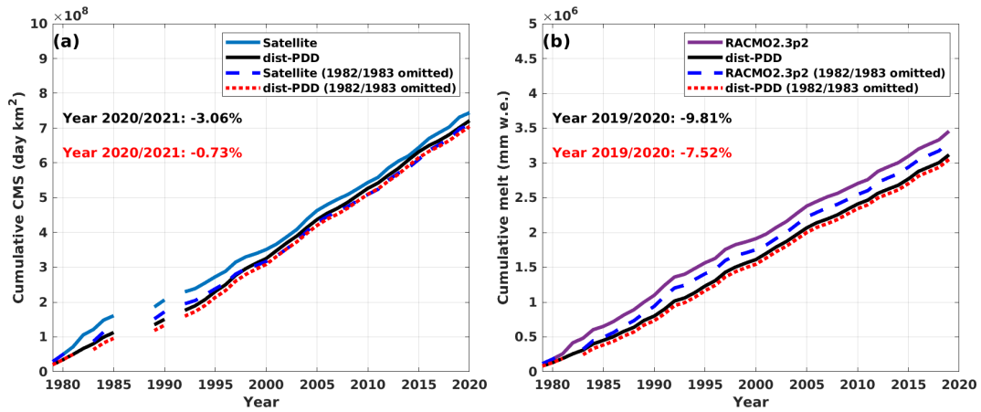
Figure E2. (a) CMS for satellite estimates and dist-PDD/dist-PDD (1982/1983 omitted) outputs from 1979/1980 to 2020/2021 (with 1986/1987 to 1988/1989 and 1991/1992 omitted). (b) Cumulative annual melt amount for RACMO2.3p2 simulations and dist-PDD/dist-PDD (1982/1983 omitted) outputs from 1979/1980 to 2019/2020.
