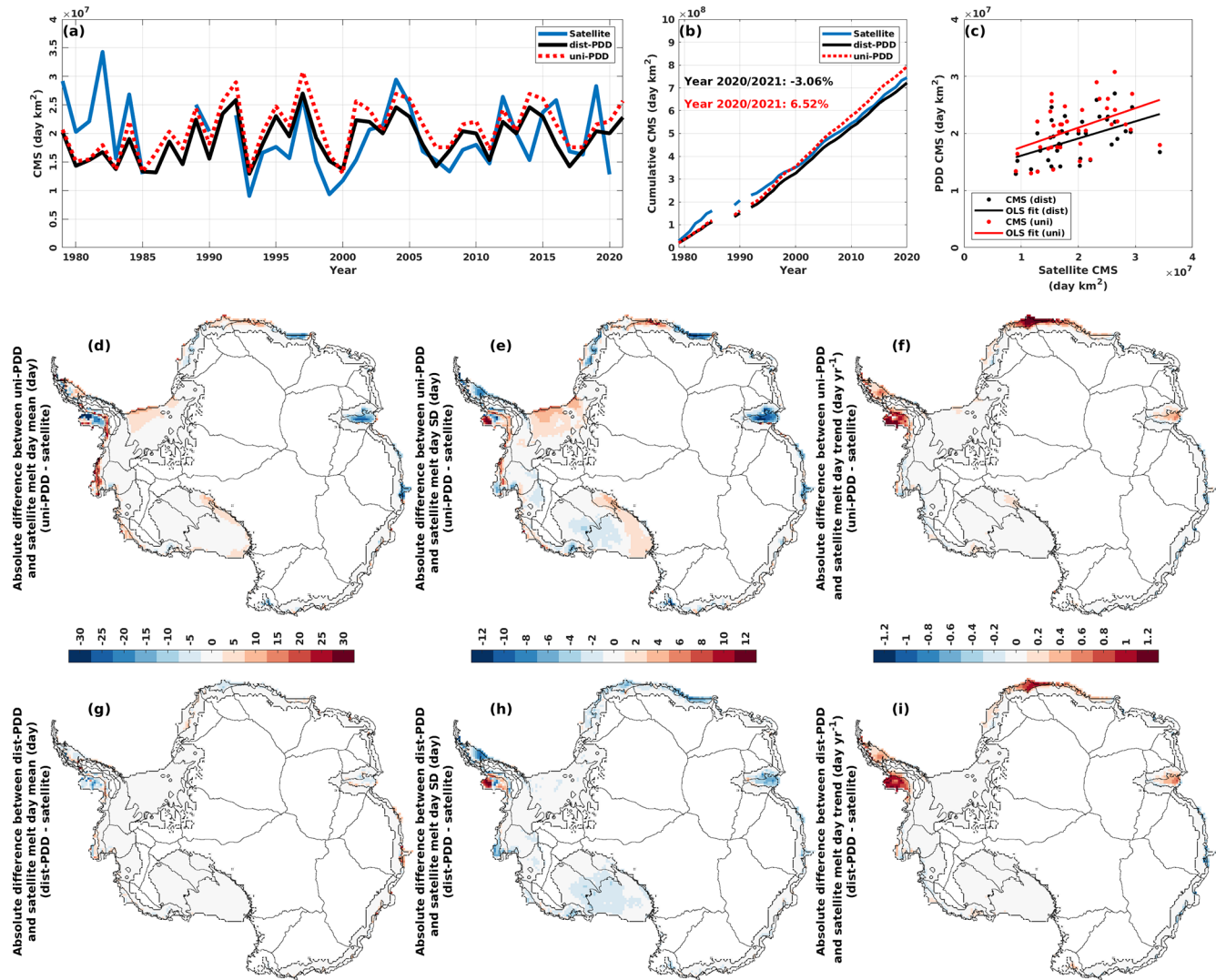
Figure 5. (a) Time series for the cumulative melting surface (CMS; \text{d km}^2 ) for satellite estimates during the period from 1979/1980 to 2020/2021 (with 1986/1987 to 1988/1989 and 1991/1992 omitted), and for dist-PDD/uni-PDD outputs during the period from 1979/1980 to 2021/2022. (b) CMS for satellite estimates and dist-PDD/uni-PDD outputs from 1979/1980 to 2020/2021 (with 1986/1987 to 1988/1989 and 1991/1992 omitted). (c) scatter plot and ordinary least squares (OLS) fit between satellite CMS and dist-PDD/uni-PDD CMS. Panels (d) to (i): absolute differences between mean, standard deviation (SD) and trend of dist-PDD/uni-PDD outputs and satellite estimates of the annual melt days. Mean, SD and trend for the dist-PDD/uni-PDD outputs and satellite estimates are calculated over the period from 1979/1980 to 2020/2021 (with 1986/1987 to 1988/1989 and 1991/1992 omitted) respectively. Note that for all panels the satellite estimates from 2002/2003 to 2010/2011 are the average of the SMMR and SSM/I sensors and the AMSR-E sensor. The satellite estimates from 2012/2013 to 2020/2021 are the average of the SMMR and SSM/I sensors and the AMSR-2 sensor.
