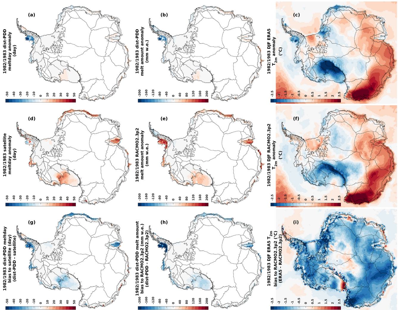
Figure E1. Panels (a) and (d): 1982/1983 dist-PDD/satellite melt day anomaly to the dist-PDD/satellite mean melt day over the period 1979/1980–2020/2021 (with 1982/1983, 1986/1987, 1987/1988, 1988/1989 and 1991/1992 omitted). Panel (g): absolute differences between 1982/1983 dist-PDD and satellite melt day. Panels (b) and (e): 1982/1983 dist-PDD/RACMO2.3p2 melt amount anomaly to the dist-PDD/RACMO2.3p2 mean melt amount over the period 1979/1980–2019/2020 (with 1982/1983 omitted). Panel (h): absolute differences between 1982/1983 dist-PDD and RACMO2.3p2 melt amount. Panels (c) and (f): 1982/1983 DJF ERA5/RACMO2.3p2 2 m air temperature anomaly to the DJF ERA5/RACMO2.3p2 mean 2 m air temperature over the period 1979/1980–2019/2020 (with 1982/1983 omitted). Panel (i): absolute differences between 1982/1983 DJF ERA5 and RACMO2.3p2 2 m air temperature. Note that for all panels the satellite estimates from 2002/2003 to 2010/2011 are the average the SMMR and SSM/I sensors and the AMSR-E sensor. The satellite estimates from 2012/2013 to 2020/2021 are the average the SMMR and SSM/I sensors and the AMSR-2 sensor.
