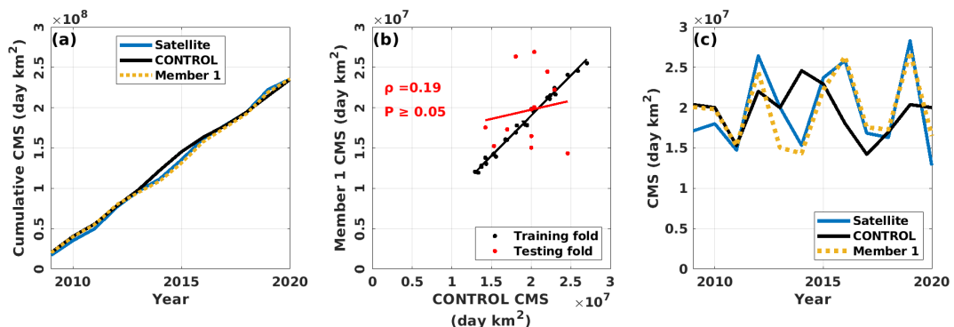
Figure F1. Panels (a) and (b) are same as Fig. 7m and s. (c) Time series of the CMS for satellite estimates, CONTROL and Member 1 during the testing fold period.
