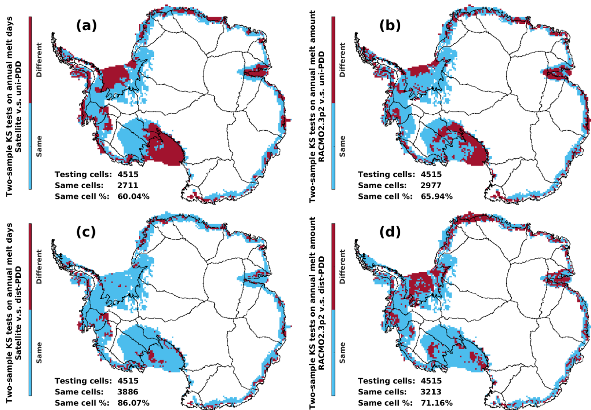
Figure 4. The two-sample KS test results. The two-sample KS tests are performed individually for each of the 4515 computing cells. The test result “Same” means the tested cell is a “same distribution cell” where there is no statistically significant evidence for the rejection of the null hypothesis that the testing two samples are from the same continuous distribution (Sect. 3.3.1). Otherwise, the cell is a “different distribution cell” (“Different”). Panels (c) and (a): the two-sample KS test results for testing the annual number of melt days between the satellite estimates and the dist-PDD/uni-PDD model outputs. Panels (d) and (b): the two-sample KS test results for testing the annual melt amount between RACMO2.3p2 simulations and the dist-PDD/uni-PDD model outputs.
