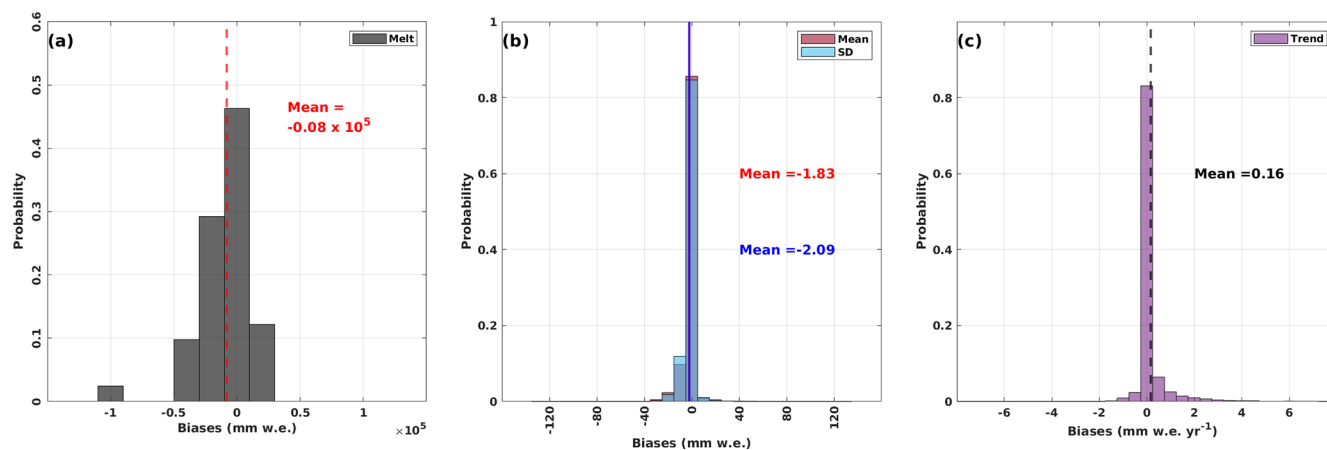
Figure D3. Panel (a): probability histogram for the biases between the dist-PDD and RACMO2.3p2 melt amounts. Vertical dashed red line indicates the mean of all biases. Panels (b) and (c): probability histograms for the biases between the dist-PDD outputs and RACMO2.3p2 simulations on mean, SD and trend. Vertical dashed red line indicates the mean of all biases between means. Vertical blue line indicates the mean of all biases between SDs. Vertical dashed black line indicates the mean of all biases between trends.
