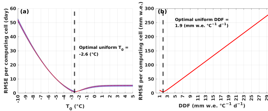
Figure C1. (a) Dotted red curve is the average of the RMSE across all satellites along each uni-PDD T_0 experiment. In each uni-PDD T_0 experiment, we calculate the RMSE between the time series of the annual sum of melt days over all computing cells between the uni-PDD model and each satellite estimate. Blue envelope covers the span of the three individual satellite results. Vertical dashed black line marks the optimal uni-PDD T_0 suggested by the minimal RMSE. (b) Red curve is the RMSE along each uni-PDD DDF experiment. In each uni-PDD DDF experiment, we calculate the RMSE between the time series of the annual sum of melt amount over all computing cells between the uni-PDD model and RACMO2.3p2. Vertical dashed black line marks the optimal uni-PDD DDF suggested by the minimal RMSE.
