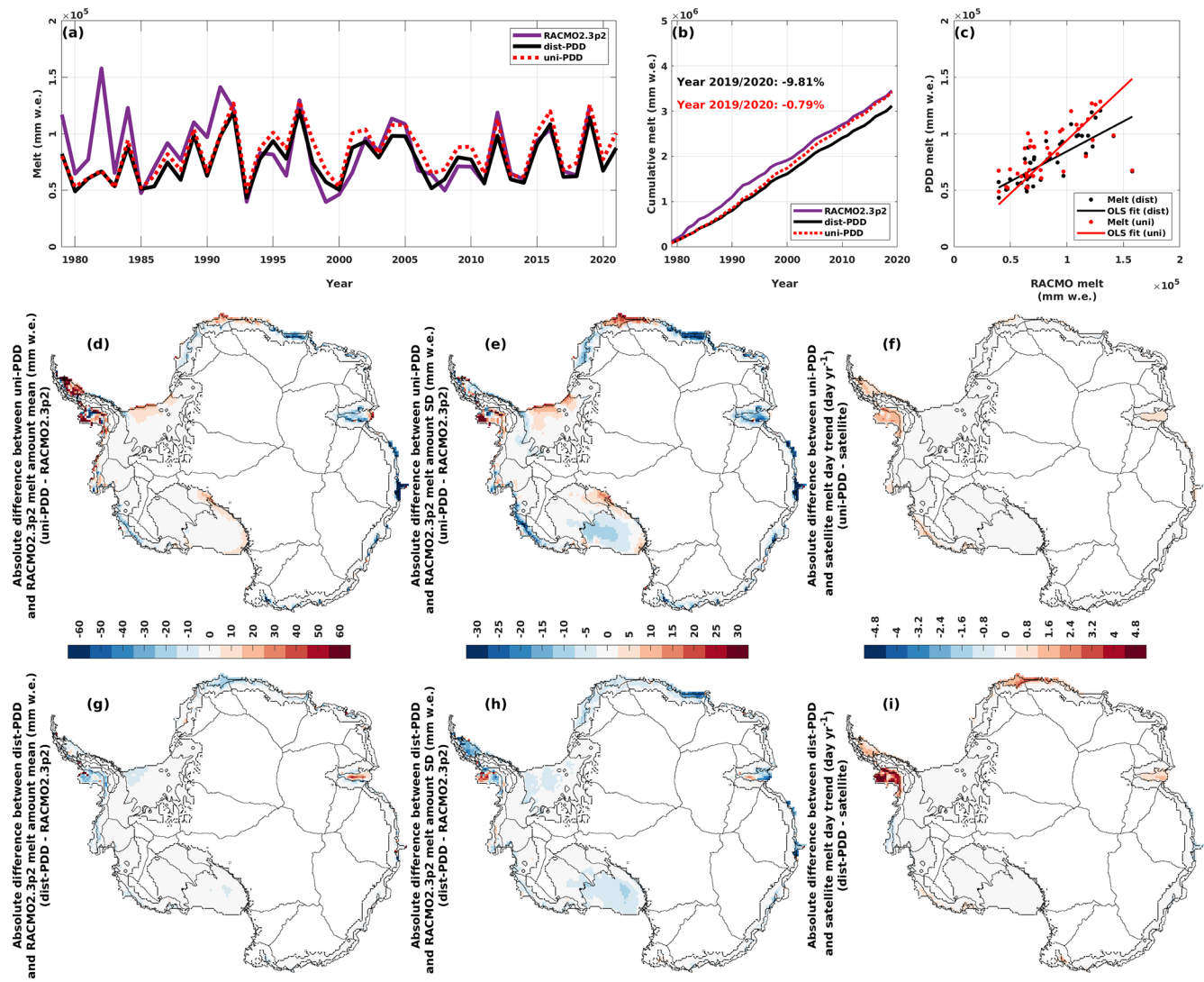
Figure 6. (a) Time series for the annual melt amount (mm w.e.) for RACMO2.3p2 simulations during the period from 1979/1980 to 2019/2020 and for dist-PDD/uni-PDD outputs during the period from 1979/1980 to 2021/2022. (b) Cumulative annual melt amount for RACMO2.3p2 simulations and dist-PDD/uni-PDD outputs from 1979/1980 to 2019/2020. (c) Scatter plot and ordinary least squares (OLS) fit between satellite annual melt amount and dist-PDD/uni-PDD annual melt amount. Panels (d) to (i): absolute differences between mean, standard deviation (SD) and trend of dist-PDD/uni-PDD outputs and RACMO2.3p2 simulations on the annual melt amount. Mean, SD and trend for the dist-PDD/uni-PDD outputs and satellite estimates are calculated over the period from 1979/1980 to 2019/2020 respectively.
