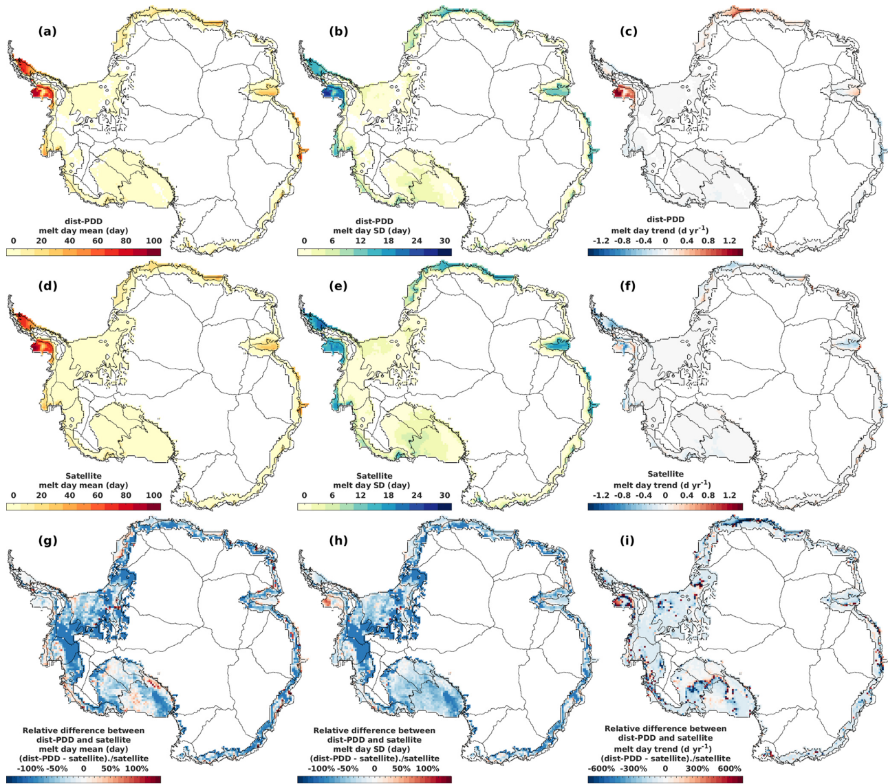
Figure D2. Panels (a) to (f): mean, SD and trend of dist-PDD/satellite melt days for the period 1979/1980 to 2020/2021 respectively. Panels (g) to (i): relative difference between dist-PDD and satellite melt day mean, SD and trend for the period 1979/1980 to 2020/2021 respectively. Note that for all panels the satellite estimates from 2002/2003 to 2010/2011 are the average the SMMR and SSM/I sensors and the AMSR-E sensor. The satellite estimates from 2012/2013 to 2020/2021 are the average the SMMR and SSM/I sensors and the AMSR-2 sensor. For all panels, the periods 1986/1987, 1987/1988, 1988/1989 and 1991/1992 are omitted.
