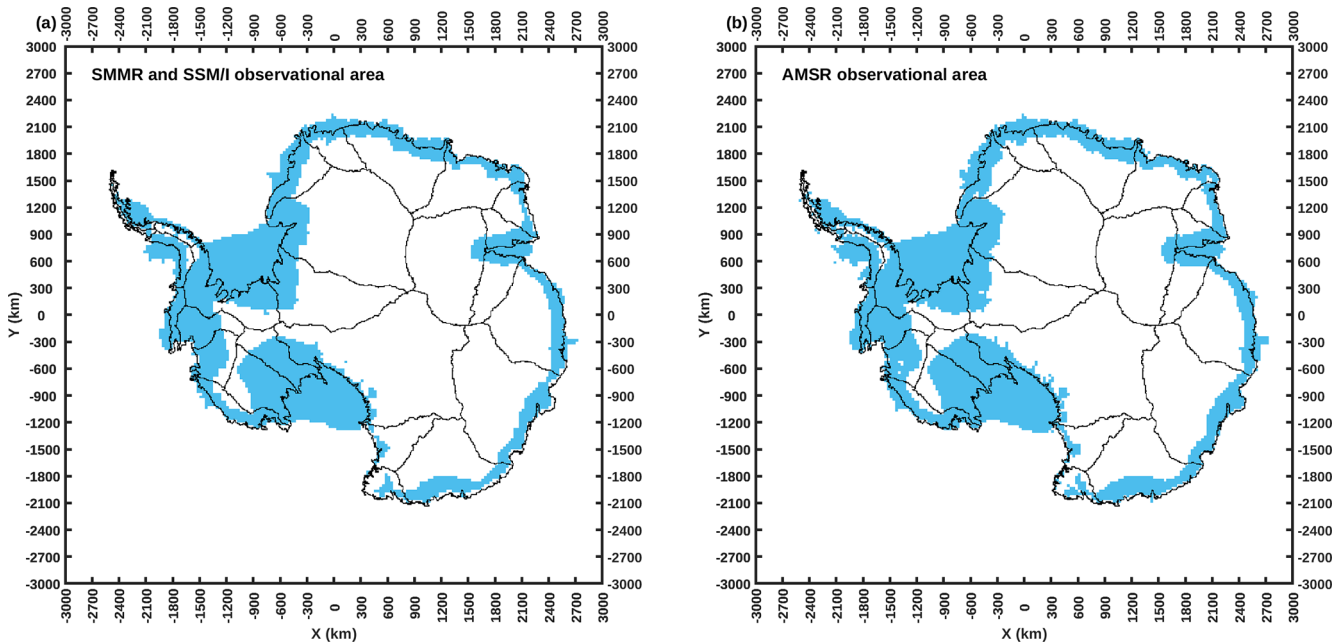
Figure A2. (a) Mask of the satellite SMMR and SSM/I observational area. (b) Mask of the satellite AMSR (AMSR-E and AMSR-2) observational area. Both masks are bilinearly remapped to the 30 km × 30 km polar stereographic grid.
