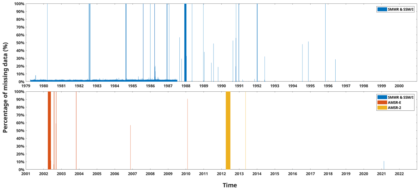
Figure A1. Daily percentage of missing data for satellite estimates. Satellite SMMR and SSM/I cover the period from 1 April 1979 to 31 March 2021. Satellite AMSR-E covers the period from 1 April 2002 to 31 March 2011. Satellite AMSR-2 covers the period from 1 April 2012 to 31 December 2021.
