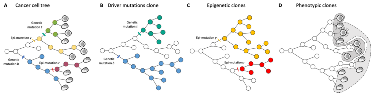
Fig. 2: Defining clones is a matter of dividing up the cancer cell tree.
