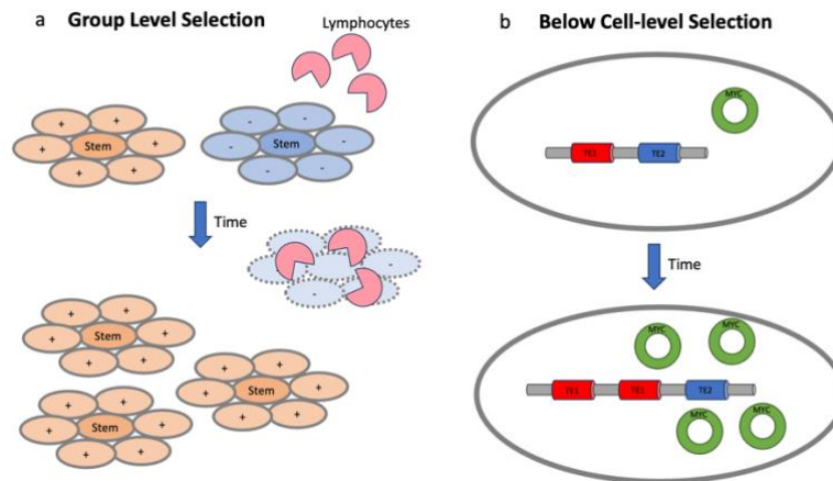
Fig. 1: Cancer evolution by natural selection can operate at multiple levels of biological organization at once.
