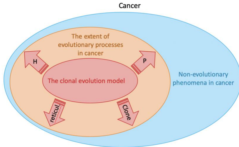
Fig. 5: Explanatory power of clonal evolution
