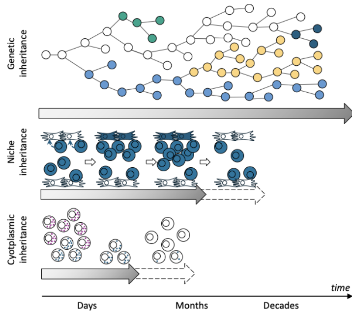
Fig. 4: Types of inheritance over various timescales.
