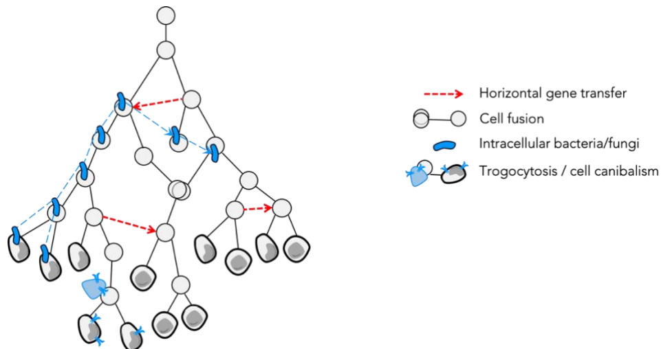
Fig. 3: Clonal evolution is more complex than a bifurcating tree of cells.
