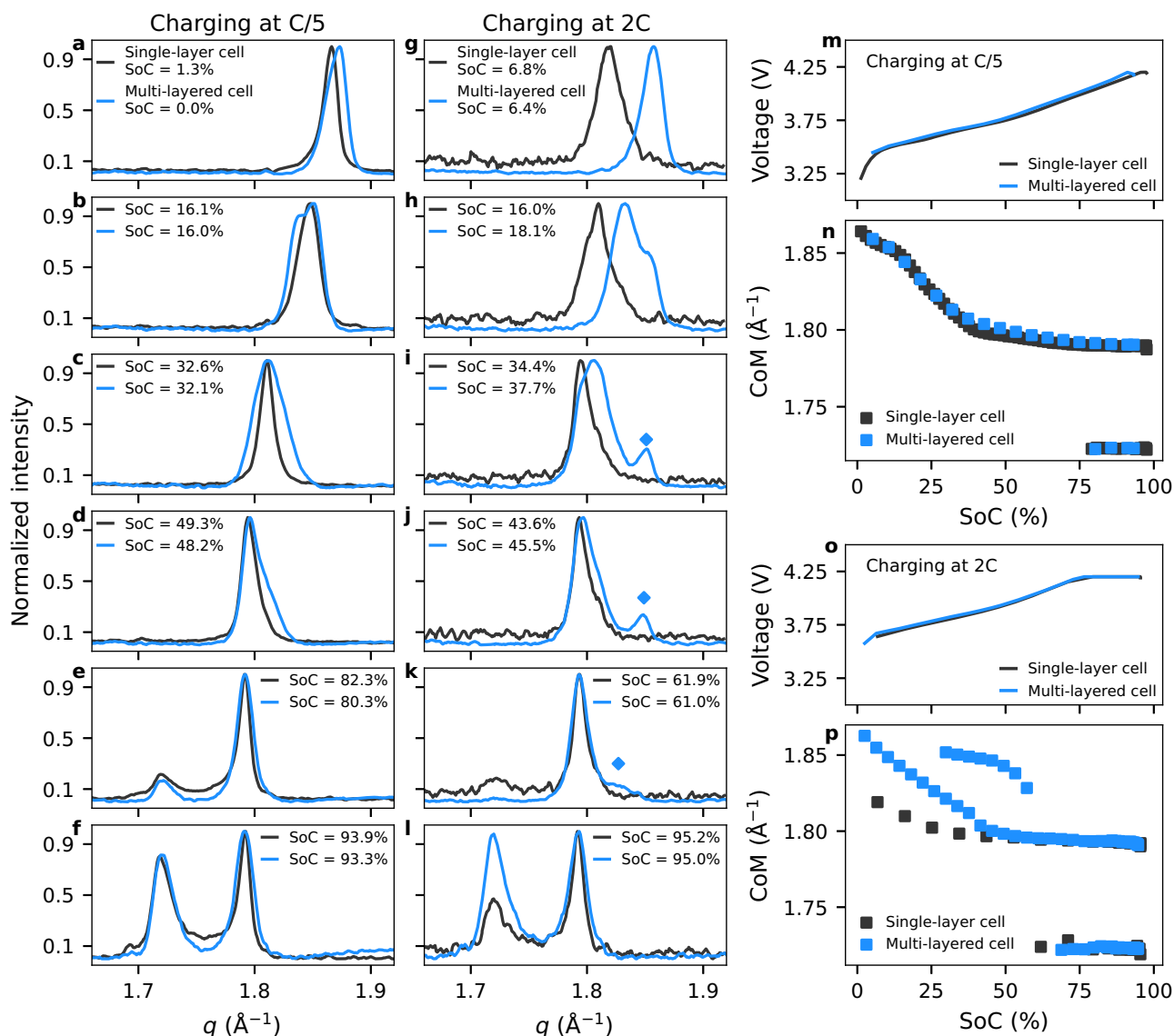
Fig. 3 | Effect of C-rate and cell design on graphite lithiation kinetics during charging. The multi-layered cell data are plotted in blue, and the single-layer cell data are plotted in black. Diffraction patterns show the evolution of the graphite (002), \text{LiC}_{12} and \text{LiC}_6 (001) peaks during charging (from -0%, top, to -95%, bottom) at (a–f) C/5 and (g–l) 2 C. Note that the initial peaks in C/5 data are very similar, indicating the same state of charge (SoC) in the initial fully delithiated state, while it
