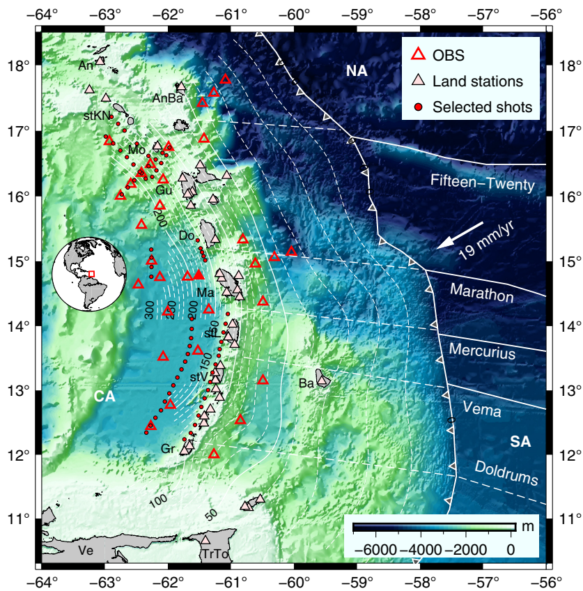
▲ Figure 1. Tectonic map of the Lesser Antilles subduction zone. The inset map shows the location of study region. Offshore and onshore seismic stations used in this study are marked by empty red and filled triangles, respectively. Light-white contours depict refined slab geometry from this study. Reference station in the 1D velocity inversion is filled by red filled triangle. Red dots in the back-arc indicate active shots included in the inversion. Details of land stations incorporated in this study are shown in © Figure S1. Inferred fracture zone and spreading-ridge structures (Schlaphorst et al. , 2016) are shown with white lines. CA, Caribbean plate; NA, North American plate; OBS, ocean-bottom seismometer; SA, South American plate. See © Figure S1 for details of island name abbreviations. The color version of this figure is available only in the electronic edition.
