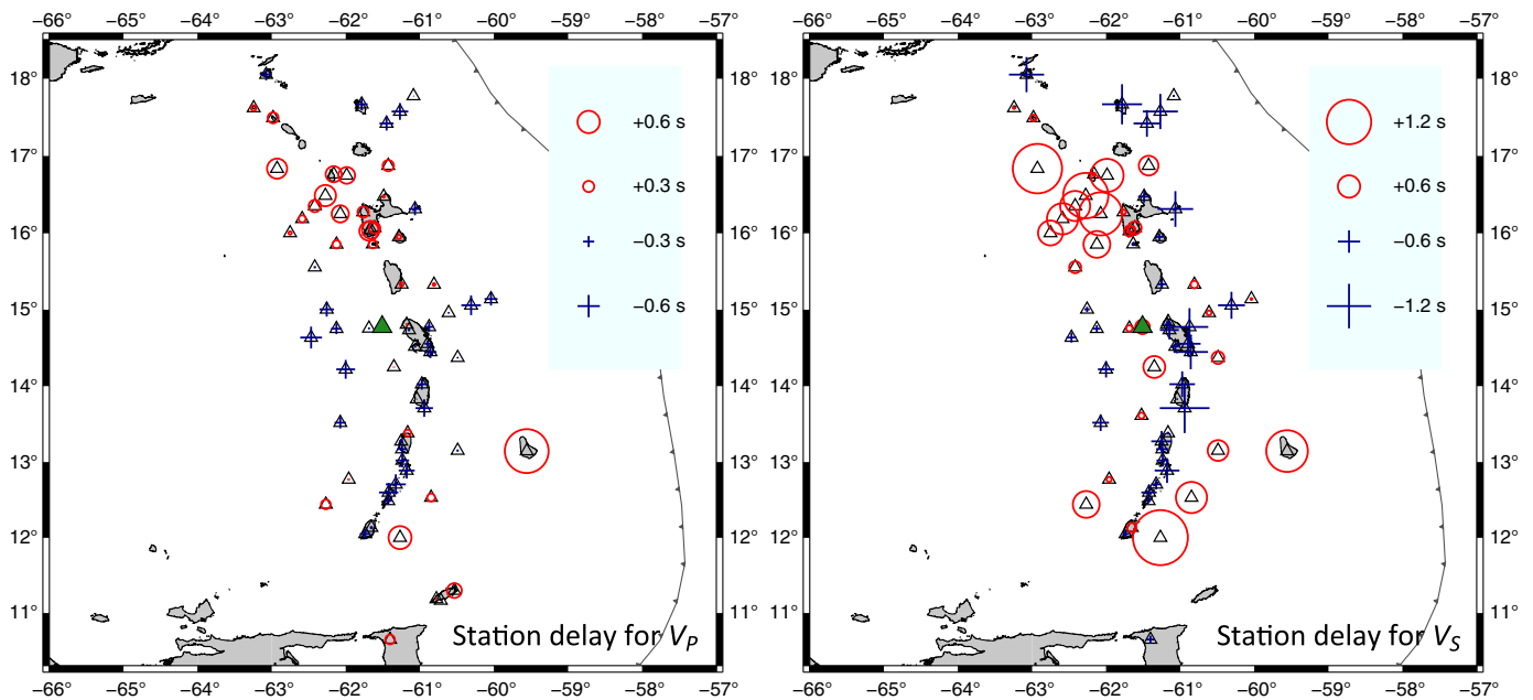
▲ Figure 3. Station corrections associated with the velocity model shown in Figure 2b. The color version of this figure is available only in the electronic edition.
