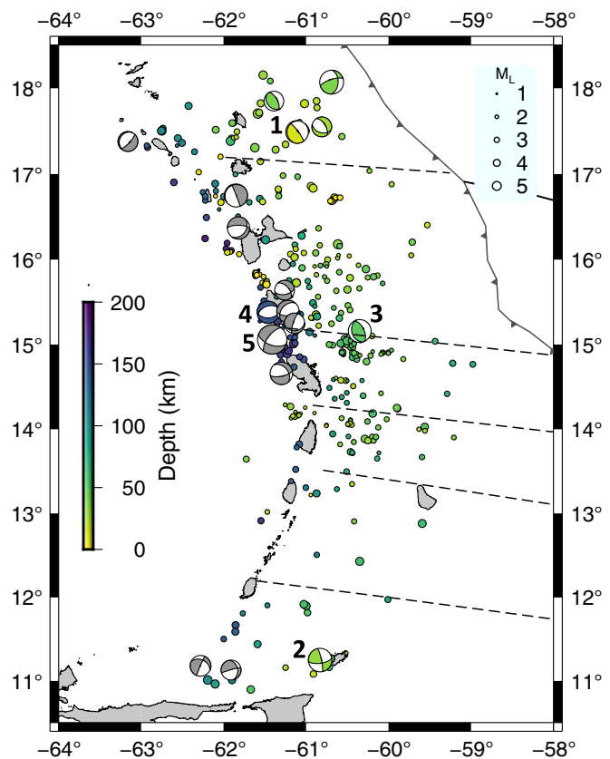
▲ Figure 6. Local seismicity as derived from this study. Focal mechanisms (FMs) for events with Global CMT (see Data and Resources ) during the period of passive-seismic experiments are colored by depth. FMs for all historical deep (>70 km) normal fault events (at least one slip direction between -145^\circ and -90^\circ ) in the Global CMT catalog and from Gonzalez et al. (2017) are marked in gray. FM 1: M_w 5.7, 17 April 2017; FM 2: M_w 5.9, 6 December 2016; FM 3: M_w 5.8, 3 February 2017; FM 4: M_w 5.6, 18 October 2016; FM 5: M_w 7.4, 29 November 2007. The color version of this figure is available only in the electronic edition.
