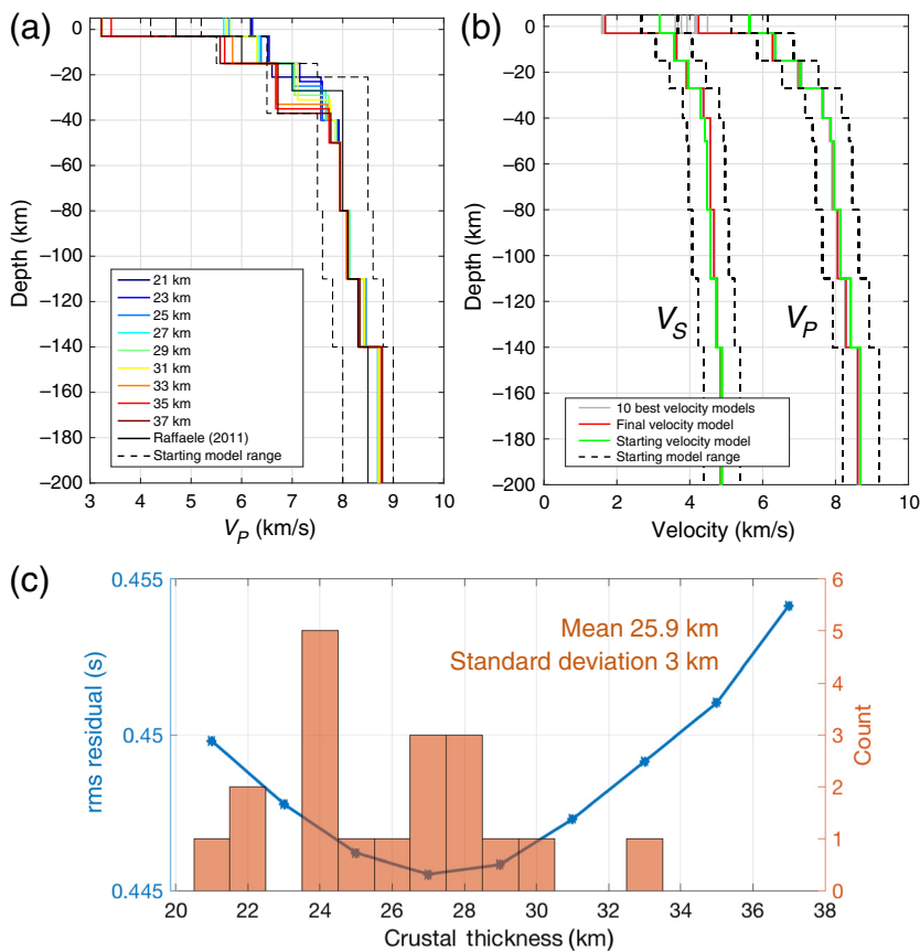
▲ Figure 2. (a) Best V_P models for simulations with different starting velocity layer configuration. The crustal thickness varies from 21 to 37 km, in 2 km increments. (b) Final V_P and V_S models for the Lesser Antilles subduction zone. (c) Root mean square (rms) residual versus the tested crustal thickness. The minimum rms misfit is achieved with a crustal thickness of 27 km. The bar chart shows the distribution of crustal thickness derived by González et al. (2018) from 19 land stations along the arc. The color version of this figure is available only in the electronic edition.
