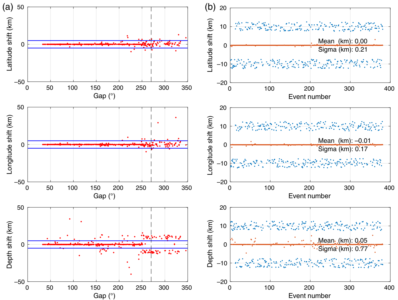
▲ Figure 4. Stability test using the velocity model shown in Figure 2b to recover the randomly perturbed earthquakes (blue points) in the longitude, latitude, and depth directions. Those recovered (red points) to be within 5 km (marked as blue line in (a)) from their original locations and having azimuthal gap smaller than 270^\circ (black dashed line) are deemed as events with good quality and shown in Figures 5 and 6. (b) The mean and standard deviation of the difference between the recovered (red points) and perturbed (blue points) earthquake locations in three directions for good quality events. The color version of this figure is available only in the electronic edition.
