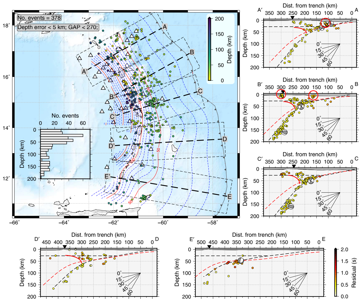
▲ Figure 5. Distribution of the relocated 378 events colored by hypocentral depth. The inset shows the number of events versus depth. Triangles are the stations from the Volatiles Recycling in the Lesser Antilles ocean-bottom seismometer deployment. Dashed blue and red lines represent the refined slab geometry from this study. Red curve delineates the wedge-shaped mantle corner seismicity. Depth profiles through the regional events comprise earthquakes that are within 75 km perpendicular distance of the labeled lines on the map. In the profiles, earthquakes are colored by their rms misfit after the relocation using the best 1D velocity models from this study. The side hemisphere focal mechanisms from the Global Centroid Moment Tensor (CMT) project (see Data and Resources ) are plotted. Black dashed curves are from slab model generated in this study, whereas the red dashed curves are from Slab2.0 (Hayes et al. , 2018). The color version of this figure is available only in the electronic edition.
