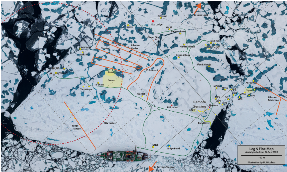
Figure 5. Main sampling locations and measurement sites of the third MOSAiC Central Observatory during late summer 2020. The background of the map is an aerial photo of the ice floe (photo credit S. Graupner). Primary water column sampling was from RV Polarstern (light blue, lower righthand side). Ocean City did not have a CTD-rosette system. Ice cores (not new ice formations) in August and September 2020 were sampled from a single site (yellow area). New ice formation and waters from the upper ocean (1-2m) were sampled at RS, OC, ROV, and Luna leads. ECO Lodge (red square) was established adjacent to Ocean City lead, approximately 300 m from the ship. The map had been simplified to show main sampling and measurement positions for the ecosystem work program. Additional MOSAiC measurement sites from teams ATMO, ICE, and OCEAN can be viewed in the respective MOSAiC Overviews by Nicolaus et al. (2022b), Rabe et al. (2022) and Shupe et al. (2022).
