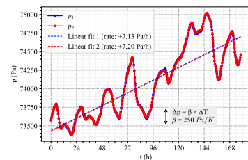
Figure 6. Leakage tests conducted at equilibrium pressure for approximately one week, with Tanks 1 and 2 disconnected. The pressure variation due to a temperature variation of 1 K is indicated by the black arrow.
